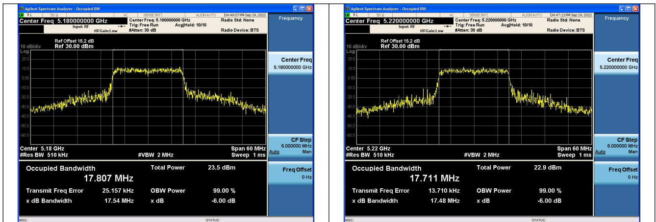
Test Mode:802.11n HT20 5180MHz Chain0
