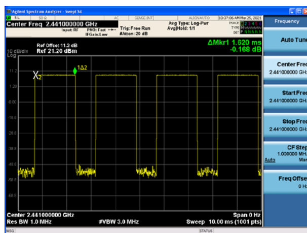
Modulation: GFSK DH3 2441
