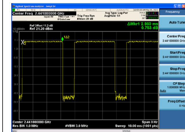
Modulation: 8DPSK DH5 2441
