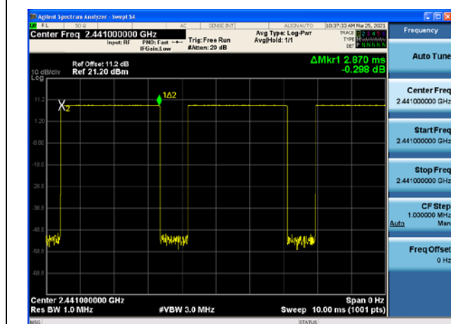
Modulation: GFSK DH5 2441
