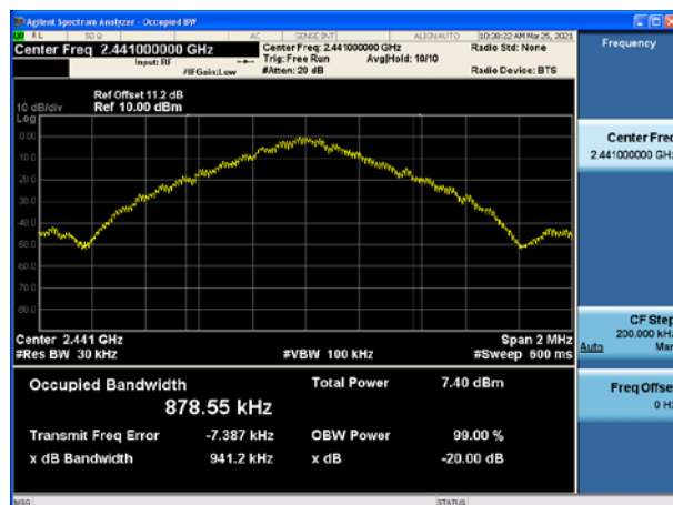
Modulation: GFSK 2441MHz
