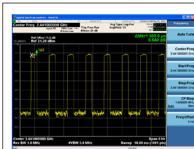
Modulation: 8DPSK DH1 2441
