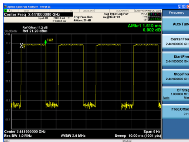
Modulation: 8DPSK DH3 2441
