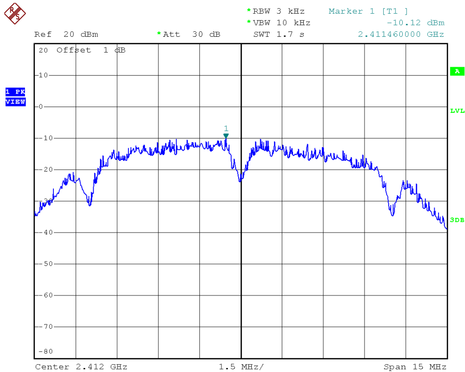
802.11b - Channel 1
