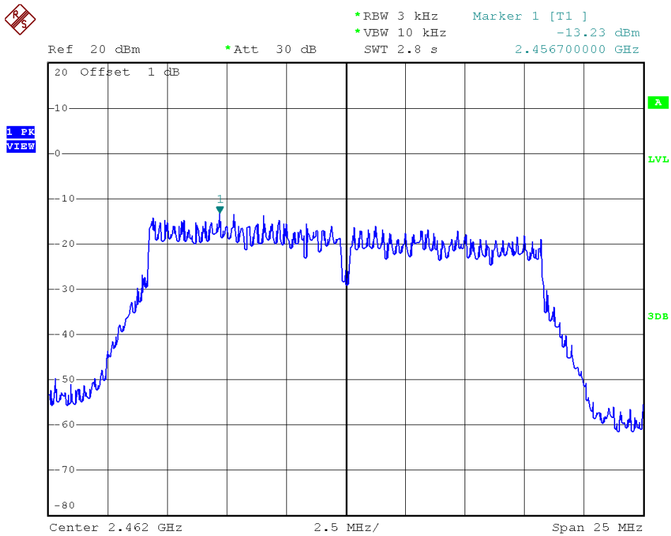
802.11g - Channel 11
