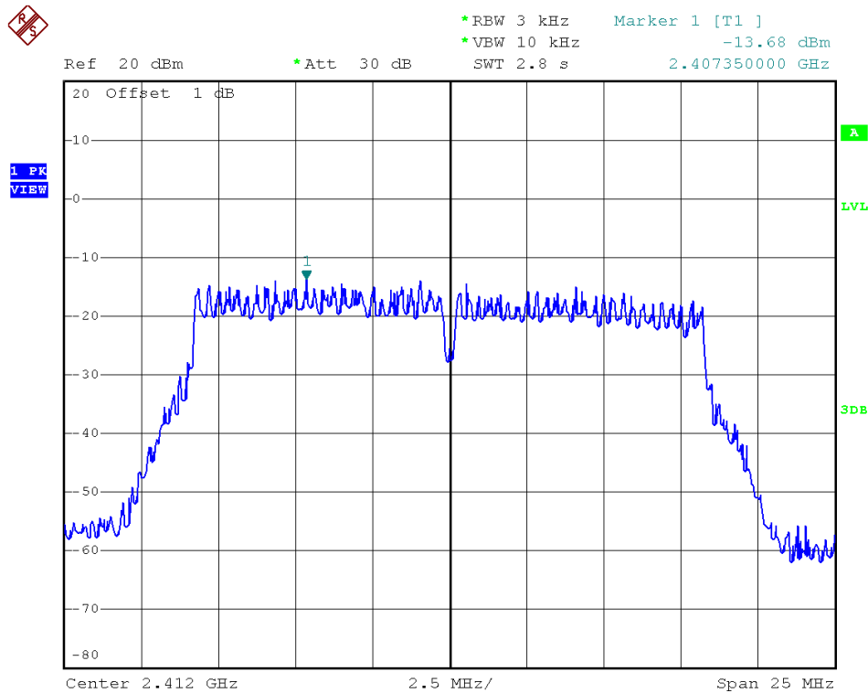
802.11g - Channel 1
