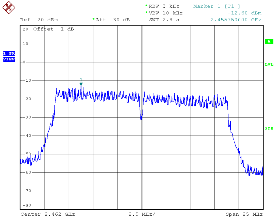
802.11n20 - Channel 11
