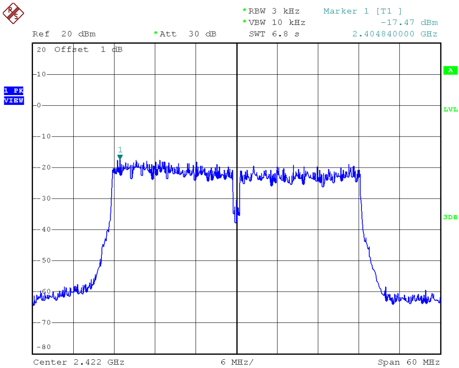
802.11n40 - Channel 3
