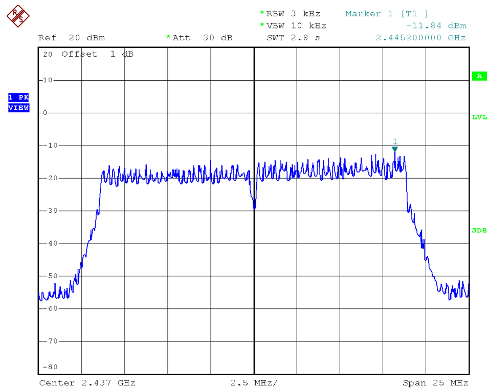
802.11n20 - Channel 6
