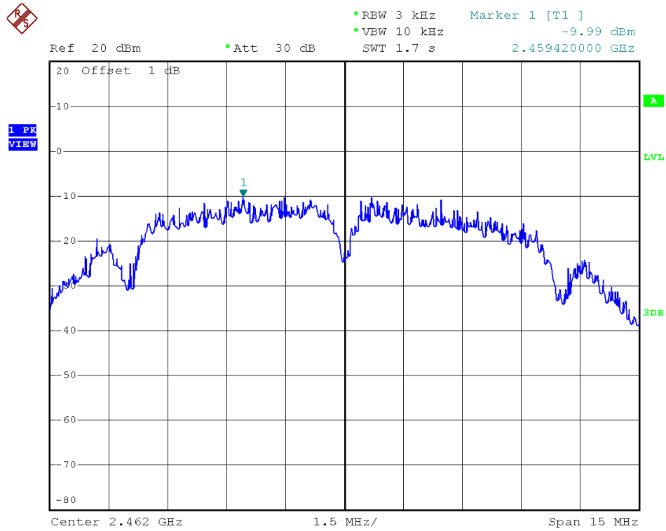
802.11b - Channel 11
