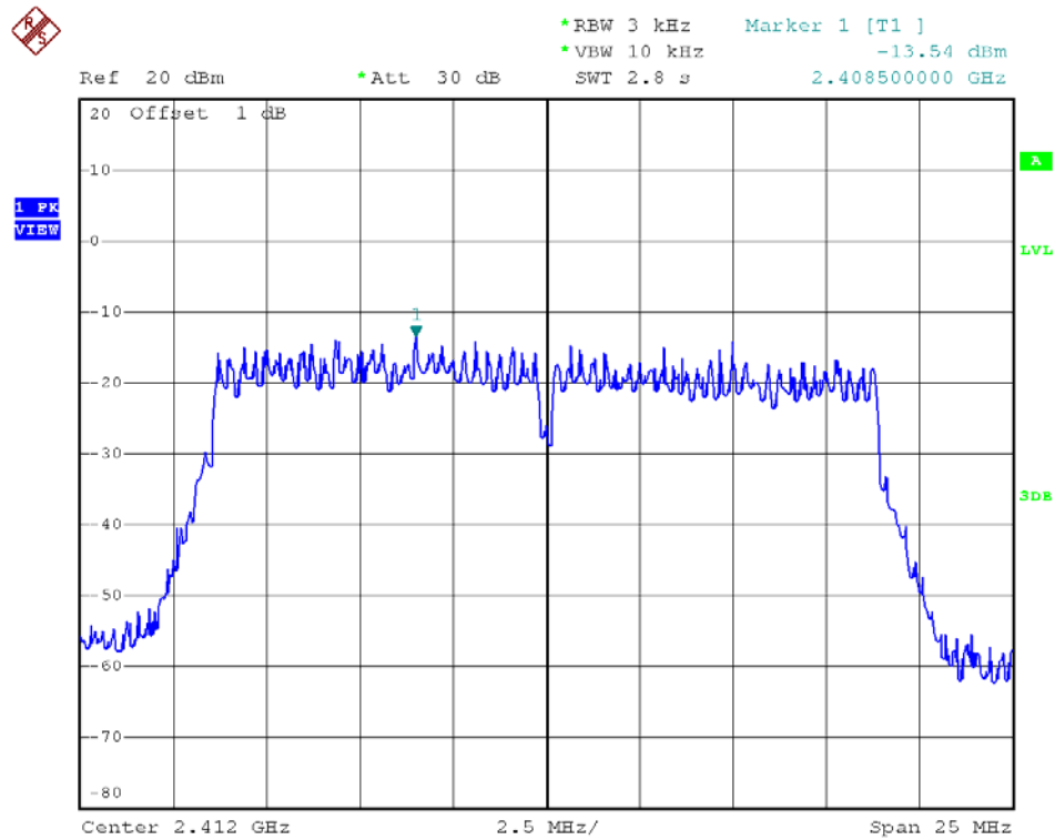
802.11n20 – Channel 1
