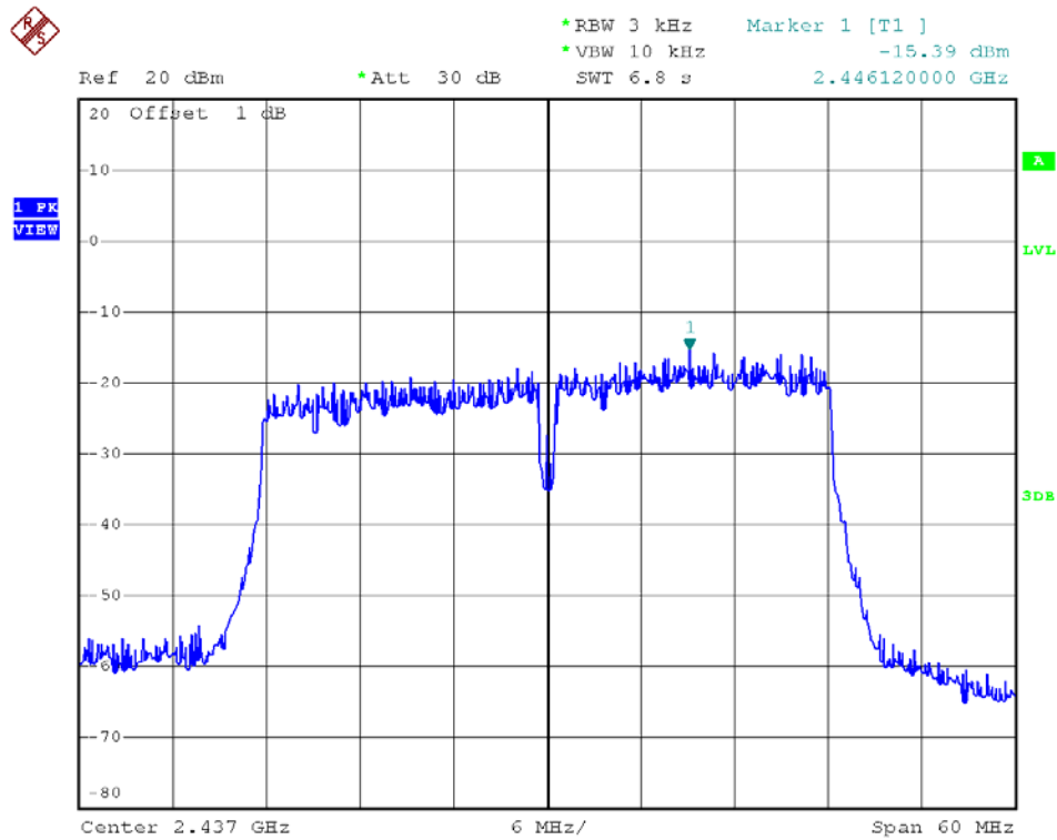
802.11n40 – Channel 6
