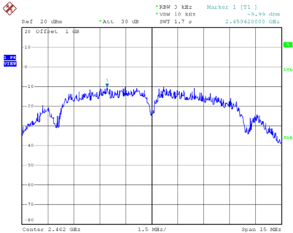
802.11b – Channel 11
