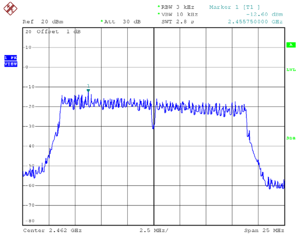
802.11n20 – Channel 11
