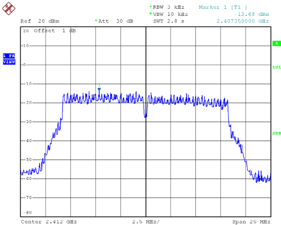
802.11g – Channel 1
