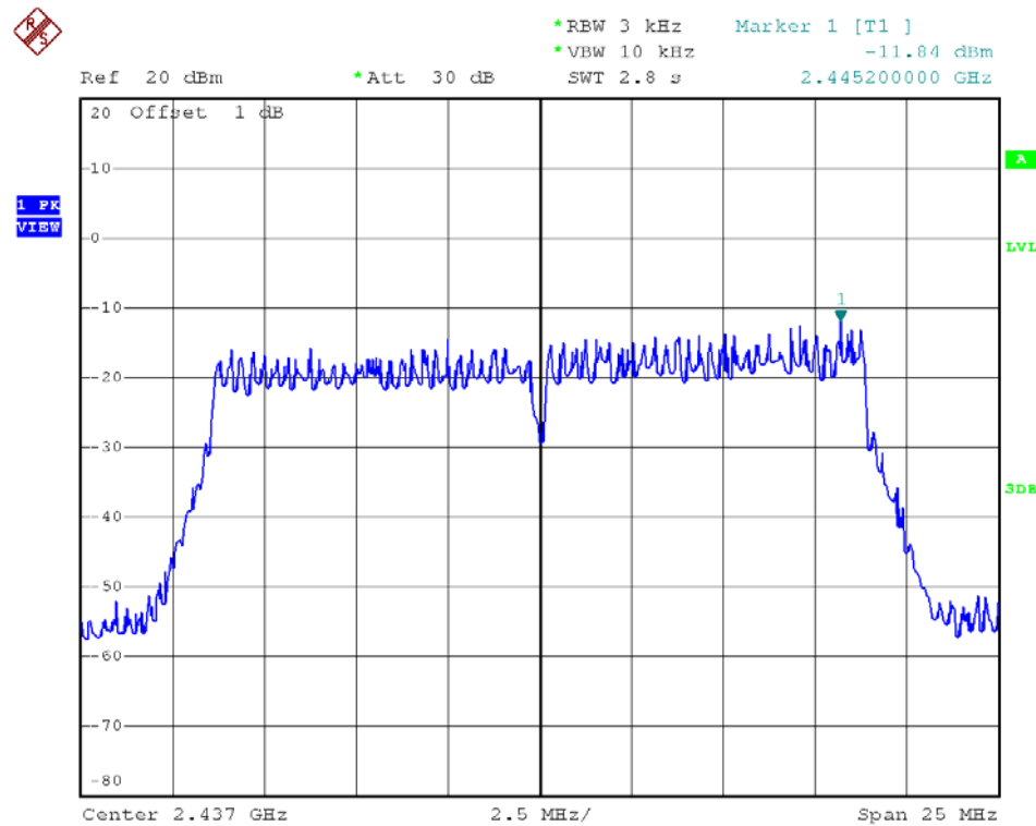
802.11n20 – Channel 6
