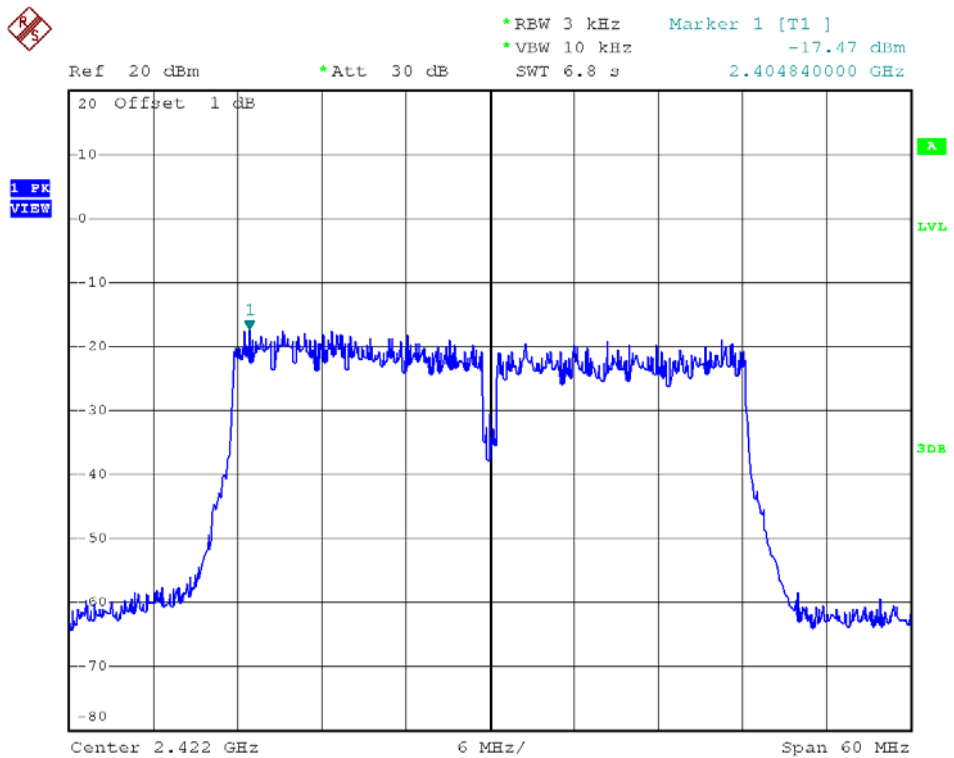
802.11n40 – Channel 3
