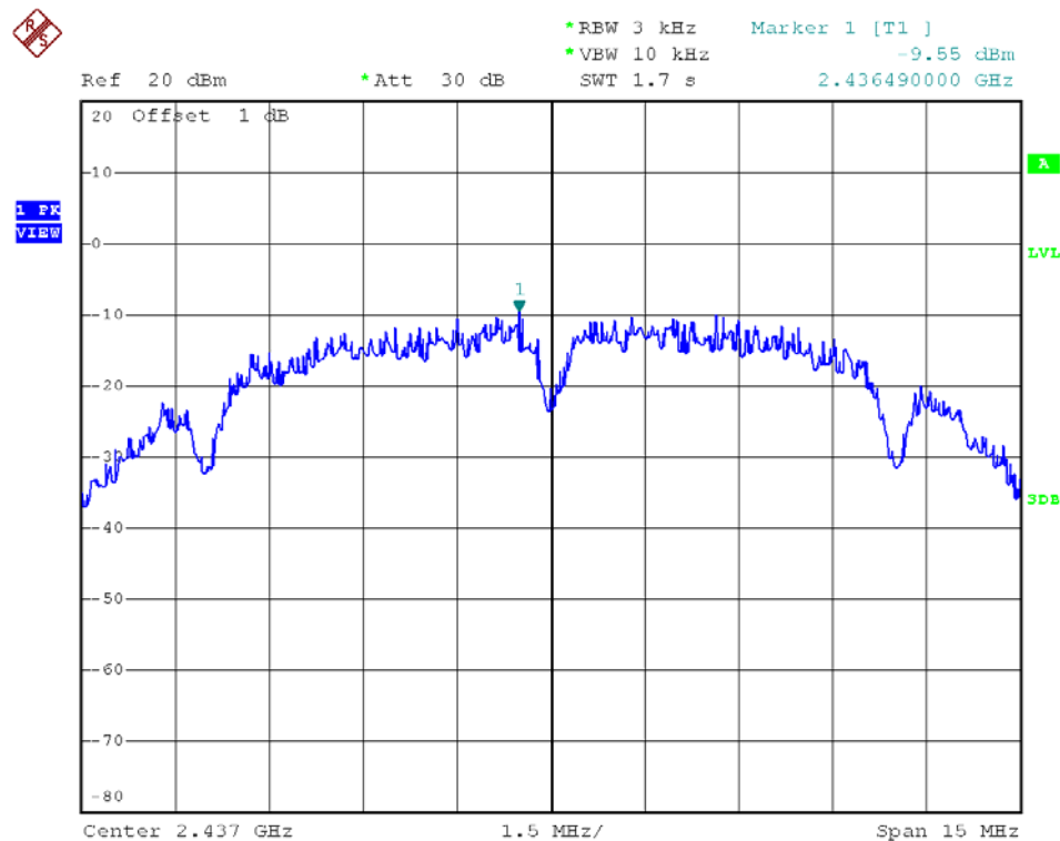
802.11b – Channel 6
