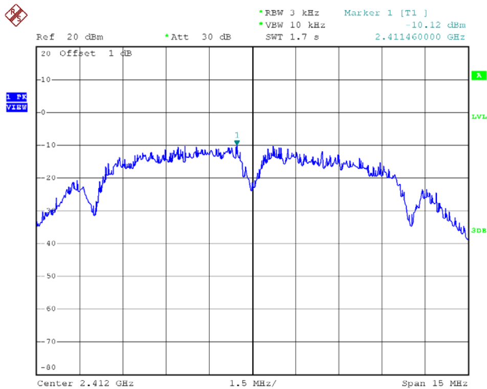
802.11b – Channel 1
