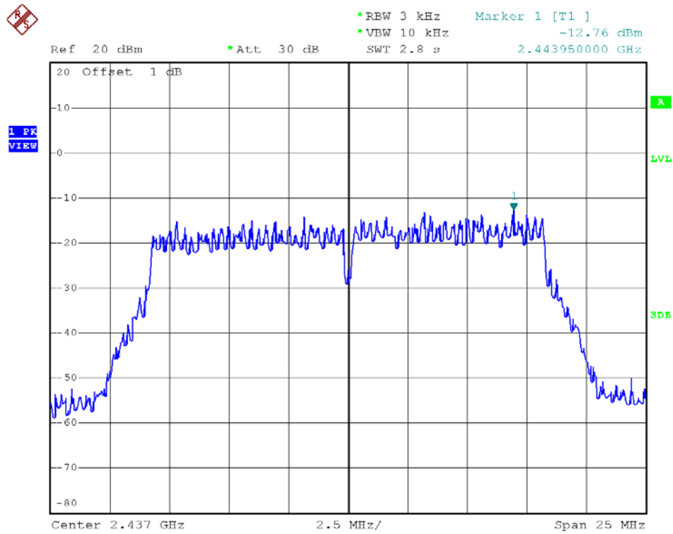
802.11g – Channel 6
