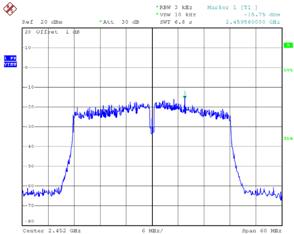
802.11n40 – Channel 9
