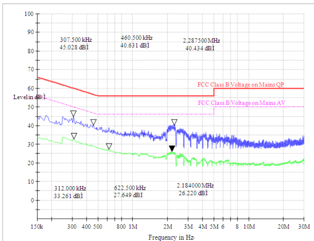
FCC Class B Voltage Test
