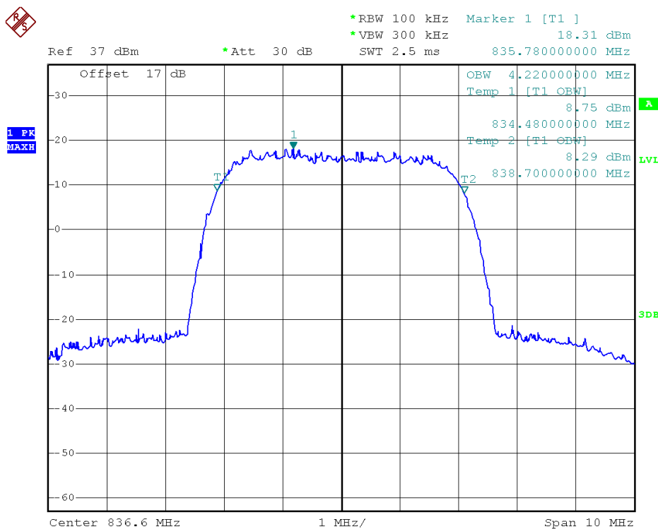
(Plot E4: WCDMA 850MHz Channel = 4183 99% Occupied Bandwidth)
