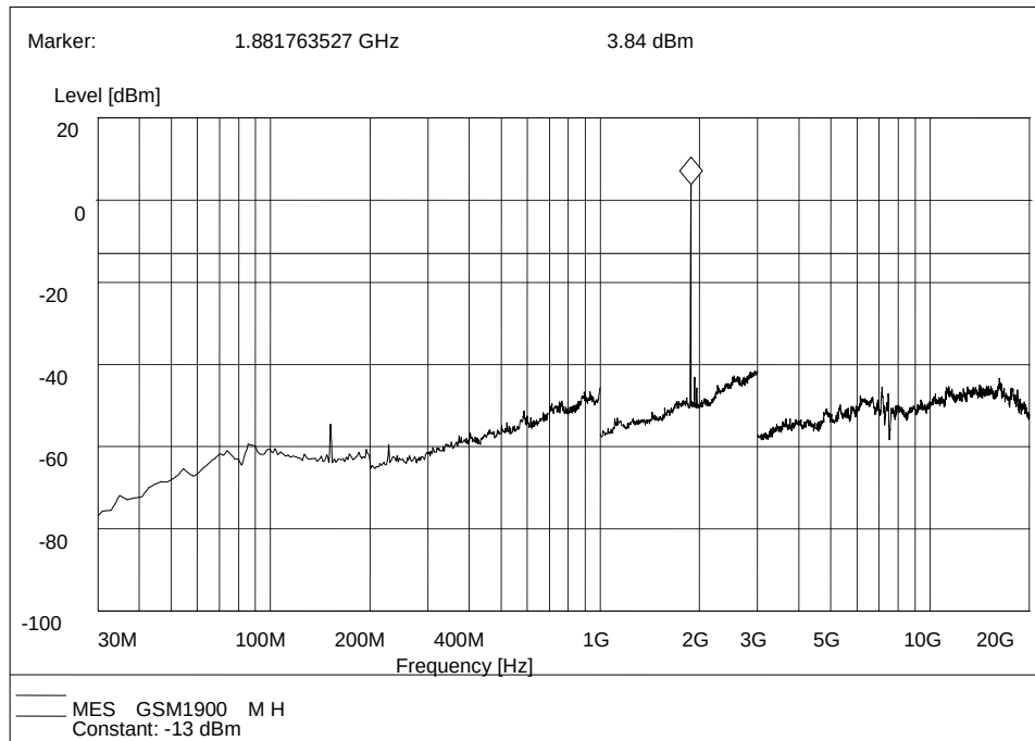
GSM 1900MHz, Test Antenna Horizontal
