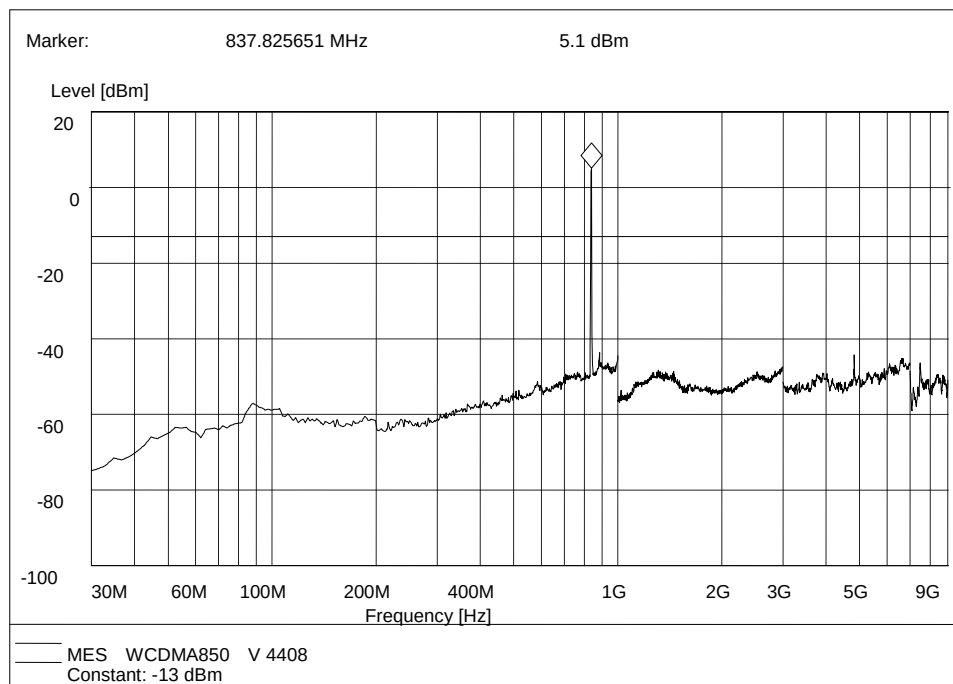
WCDMA 850MHz, Test Antenna Vertical
