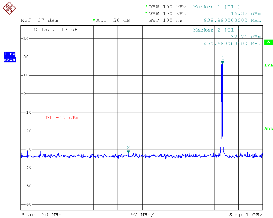
WCDMA850MHz Channel = 4183, 30MHz to 1GHz
