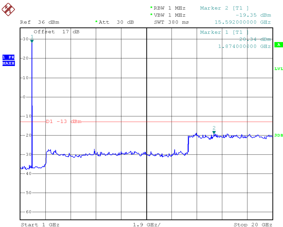
EDGE 1900MHz Channel = 661, 1GHz to 20GHz
