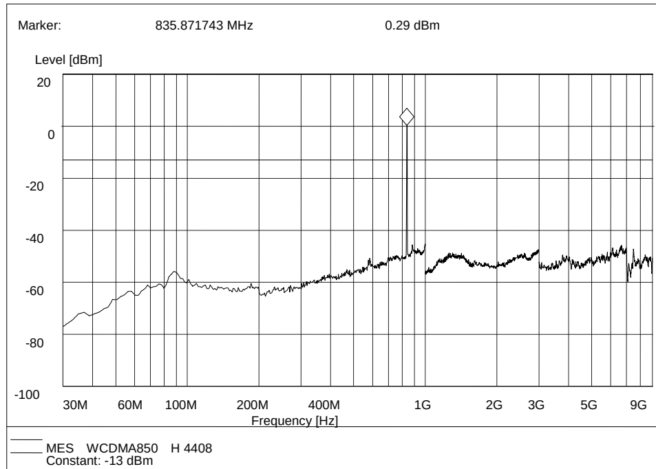
WCDMA 850MHz, Test Antenna Horizontal
