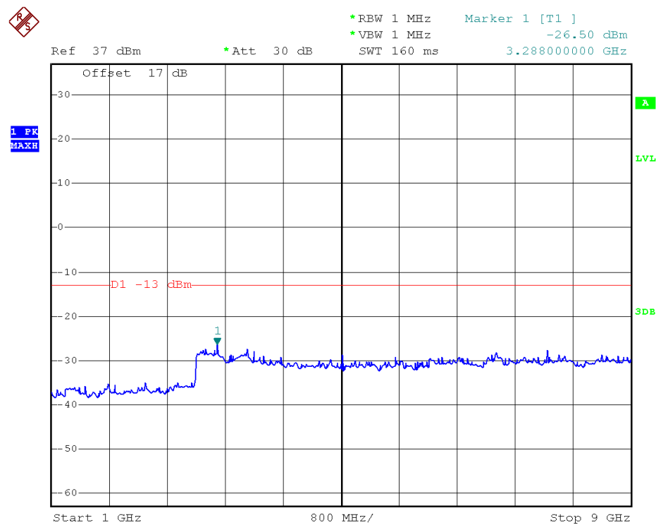
WCDMA850MHz Channel = 4183, 1GHz to 9GHz
