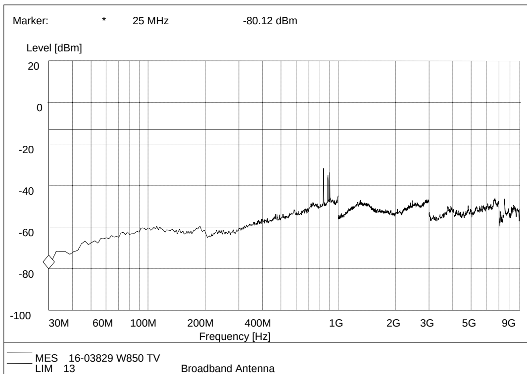
WCDMA 850MHz, Test Antenna Vertical
