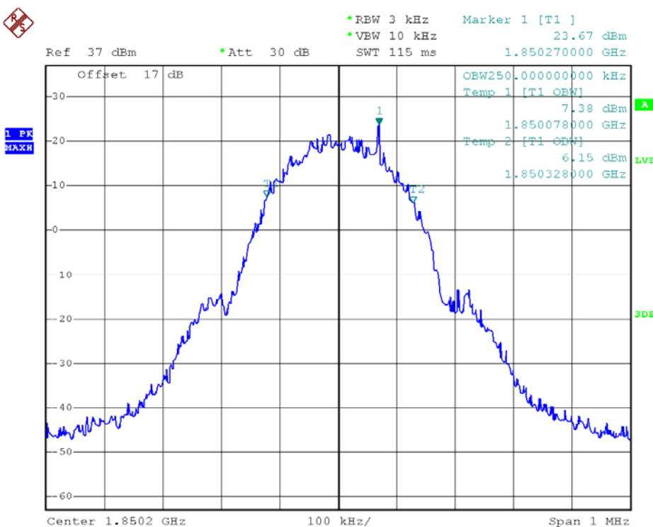
(Plot B2: GSM 1900MHz Channel = 512 99% Occupied Bandwidth)
