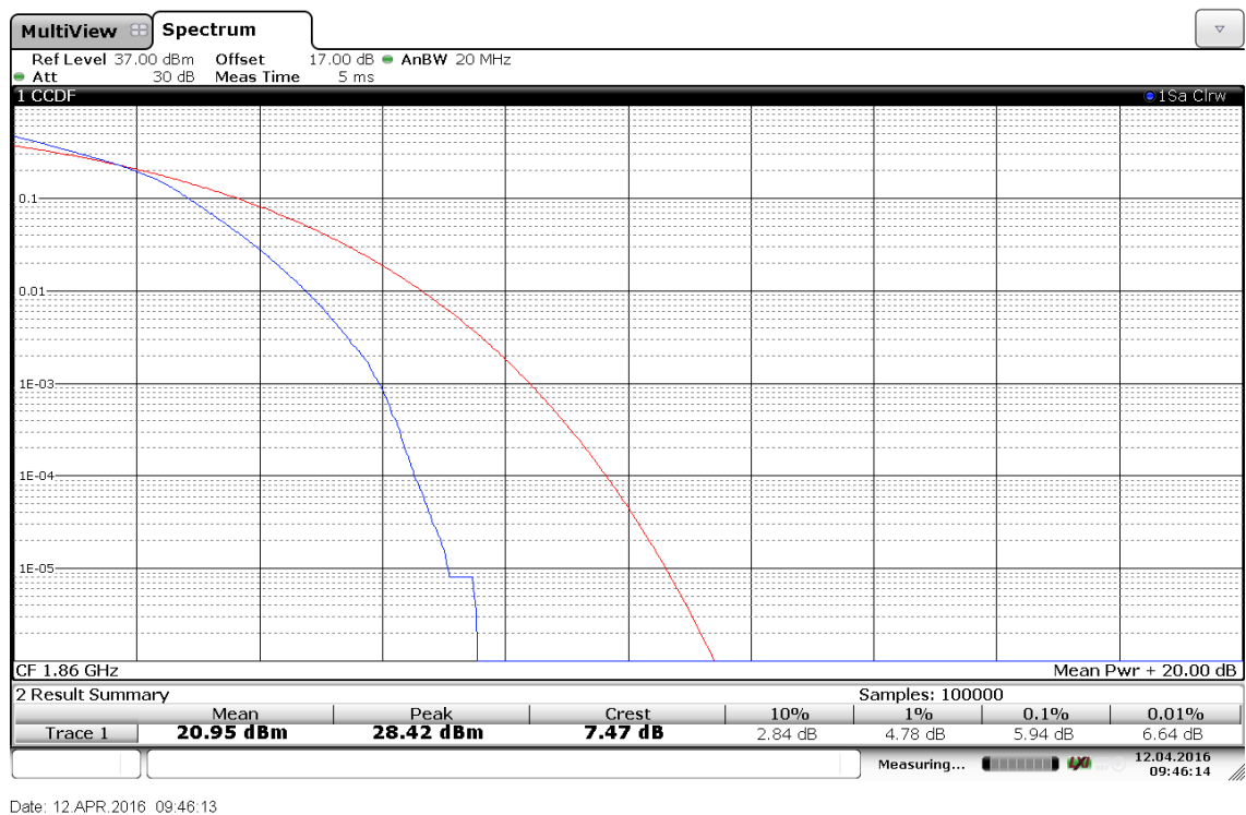
(Plot A2: Band 2/20MHz/16QAM in L Ch 100RB Size)
