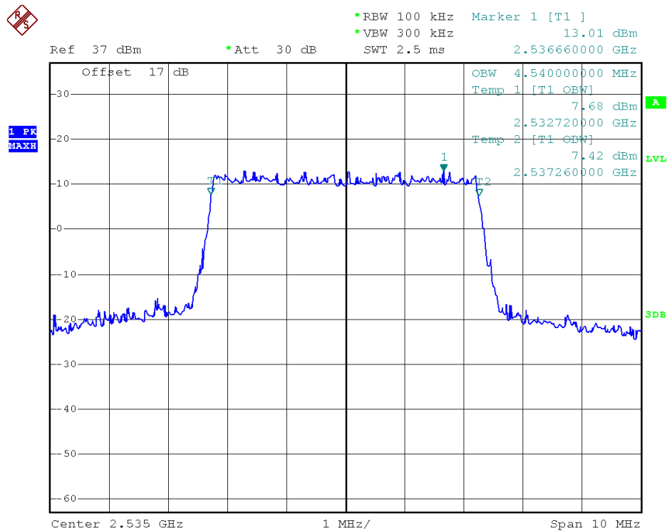
99% Occupied Bandwidth LTE Band 7/5MHz/16QAM
