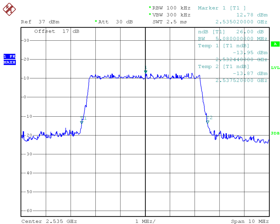
26dB Bandwidth LTE Band 7/5MHz/16QAM
