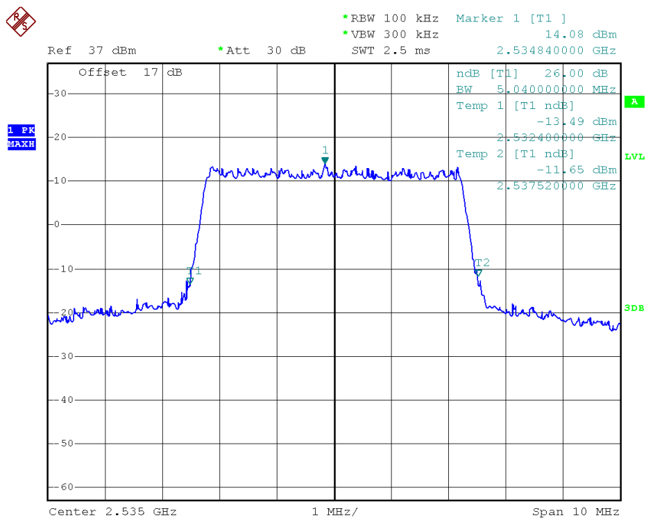
26dB Bandwidth LTE Band 7/5MHz/QPSK
