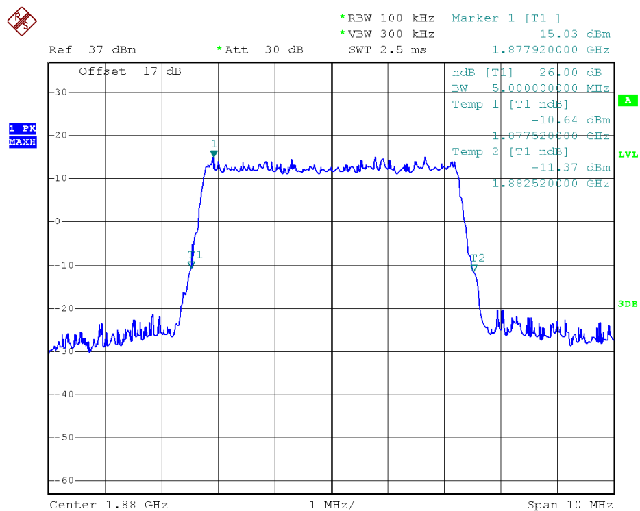
26dB Bandwidth LTE Band 2/5MHz/16QAM
