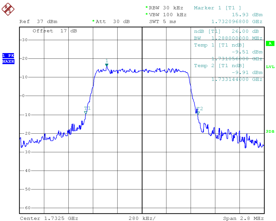
26dB Bandwidth LTE Band 4/1.4MHz/16QAM
