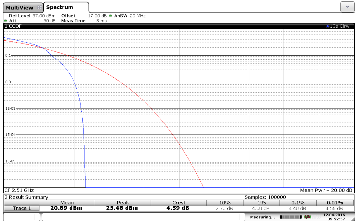
(Plot C1: Band 7/20MHz/16QAM in L Ch 1RB Size )
