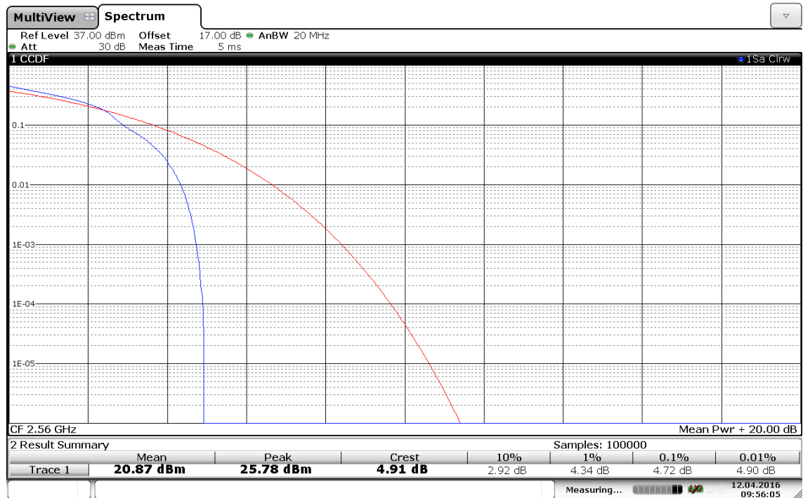
(Plot C5: Band 7/20MHz/16QAM in H Ch 1RB Size)
