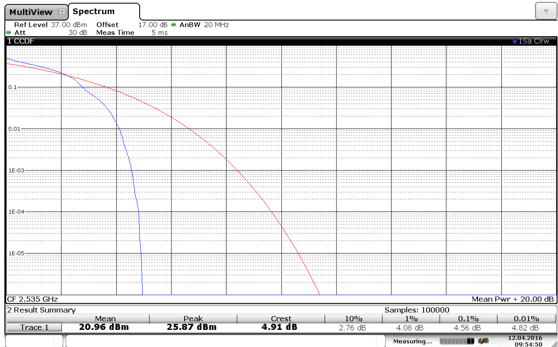
(Plot C3: Band 7/20MHz/16QAM in M Ch 1RB Size)
