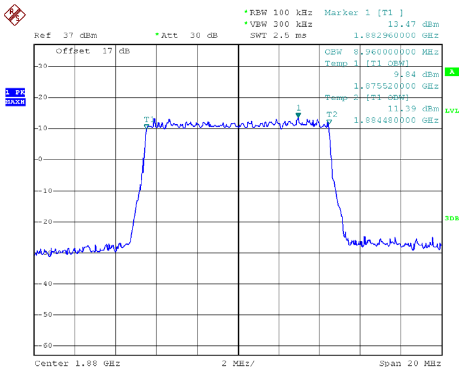
99% Occupied Bandwidth LTE Band 2/10MHz/QPSK
