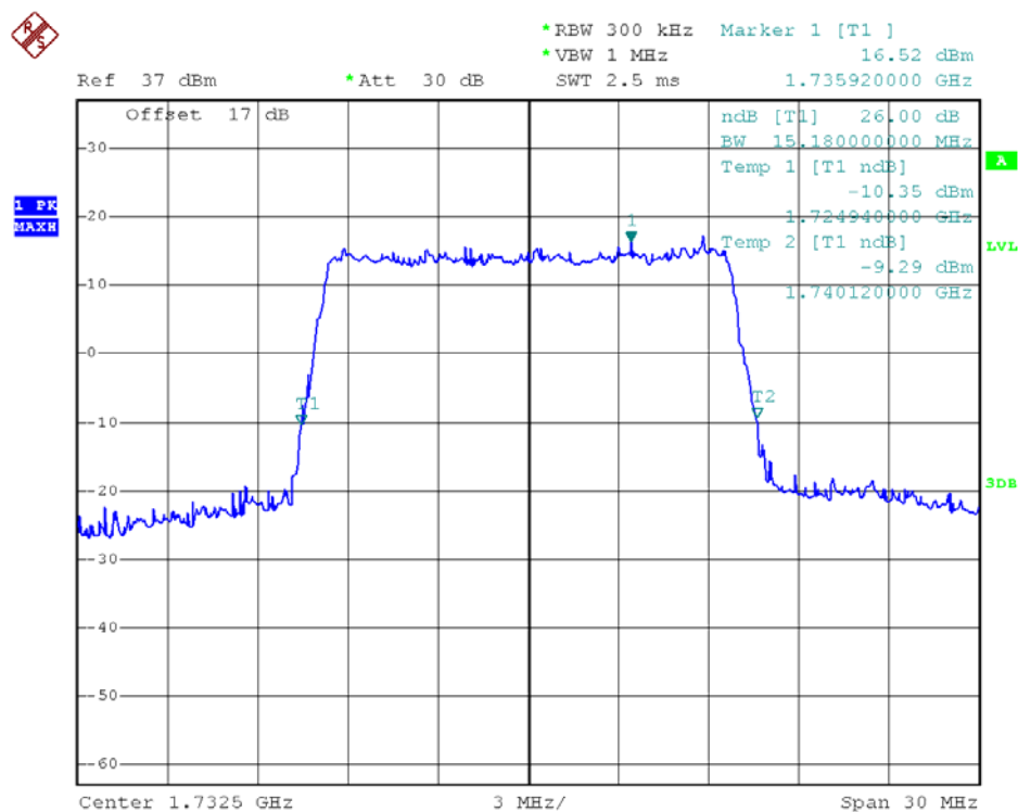
26dB Bandwidth LTE Band 4/15MHz/QPSK
