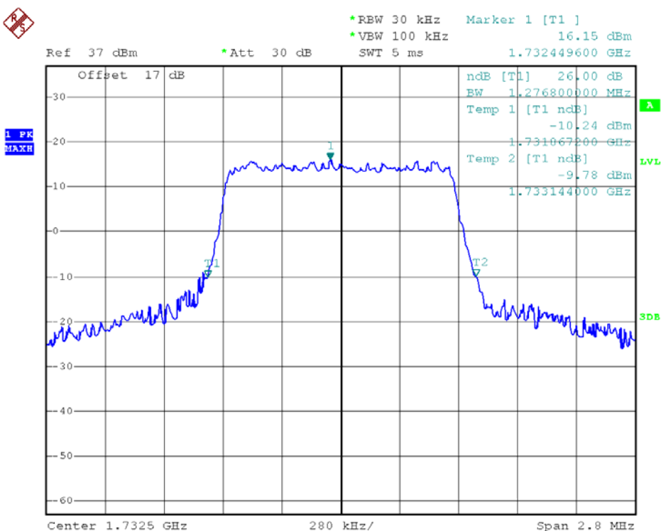
26dB Bandwidth LTE Band 4/1.4MHz/QPSK
