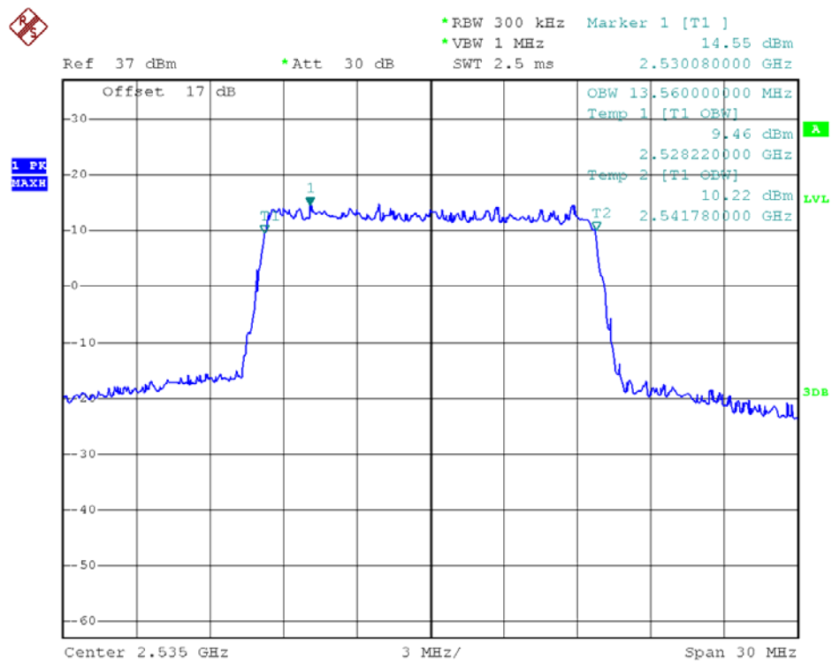
99% Occupied Bandwidth LTE Band 7/15MHz/QPSK
