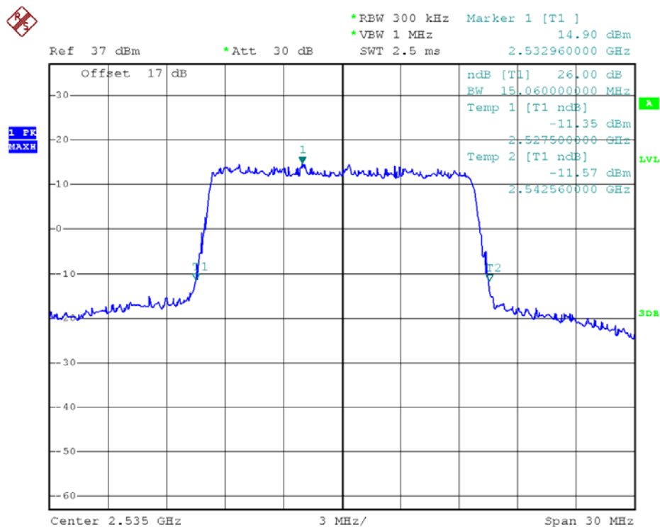
26dB Bandwidth LTE Band 7/15MHz/QPSK
