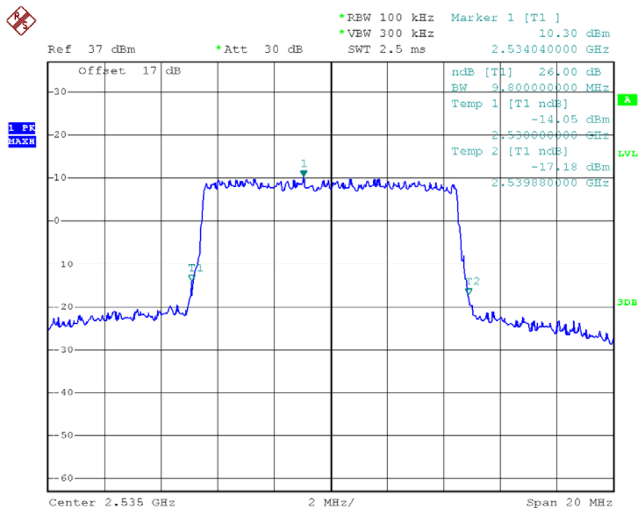
26dB Bandwidth LTE Band 7/10MHz/16QAM
