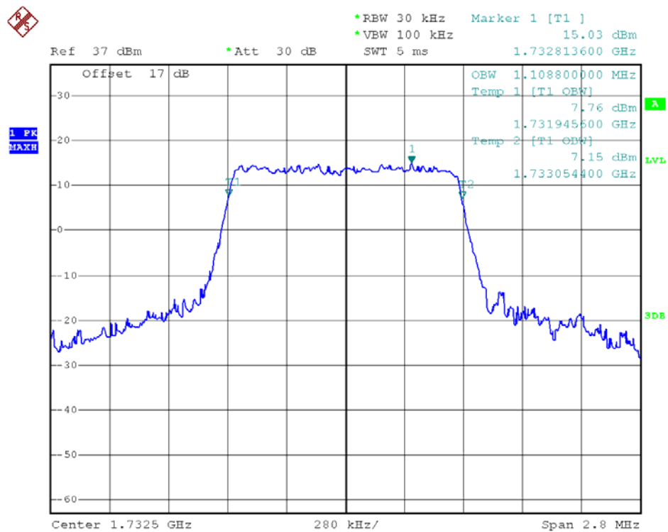
99% Occupied Bandwidth LTE Band 4/1.4MHz/16QAM
