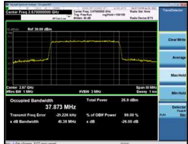
DC_2A_n41A P1/2 BPSK 40MHz CH-High
