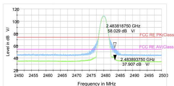
DH5-Channel 78: Peak & Average
