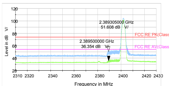
3DH5-Channel 0: Peak & Average
