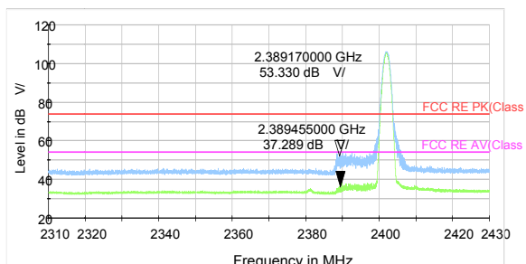
DH5-Channel 0: Peak & Average
