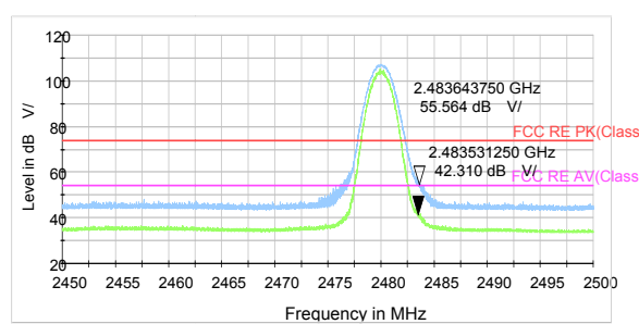
3DH5-Channel 78: Average & Average
