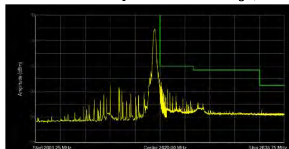
LTE Band 38 64QAM 15MHz CH-High, 1 RB
