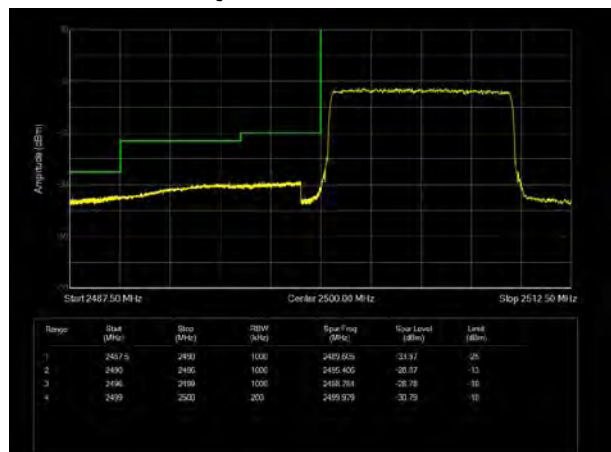
LTE Band 7 16QAM 10MHz CH-Low, 100%RB
