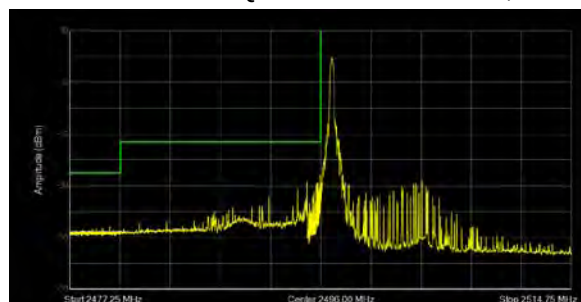
LTE Band 41 64QAM 15MHz CH-Low, 1 RB
