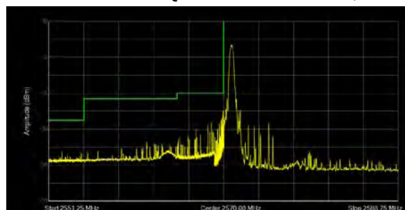
LTE Band 38 64QAM 15MHz CH-Low, 1 RB
