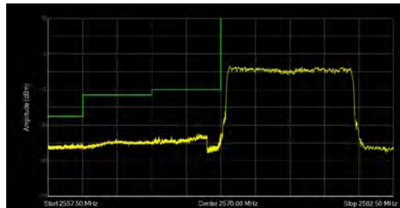
LTE Band 38 64QAM 10MHz CH-Low, 100%RB
