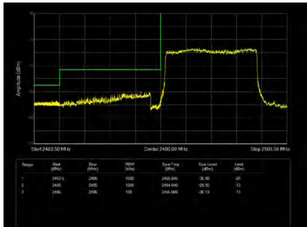
LTE Band 41 QPSK 15MHz CH-Low, 1 RB
