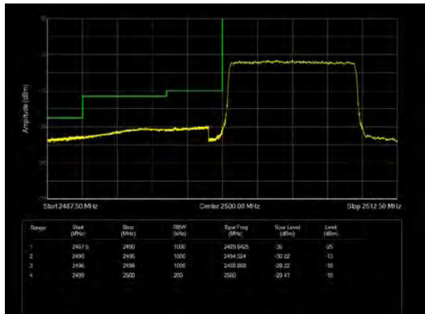
LTE Band 7 64QAM 15MHz CH-Low, 1 RB
