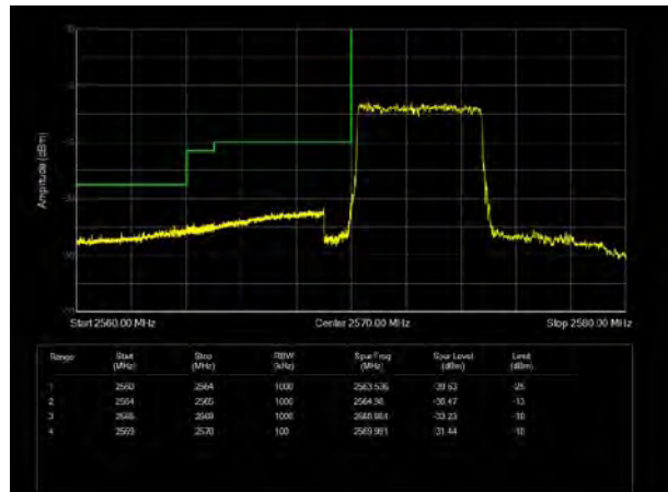
LTE Band 38 16QAM 10MHz CH-Low, 1 RB
