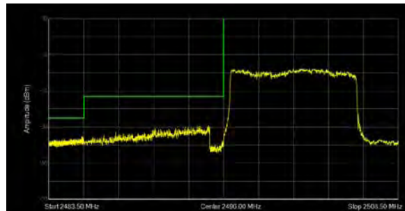
LTE Band 41 64QAM 10MHz CH-Low, 100%RB
