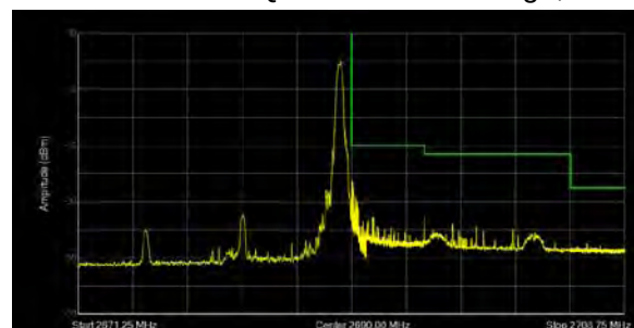
LTE Band 41 64QAM 15MHz CH-High, 1 RB
