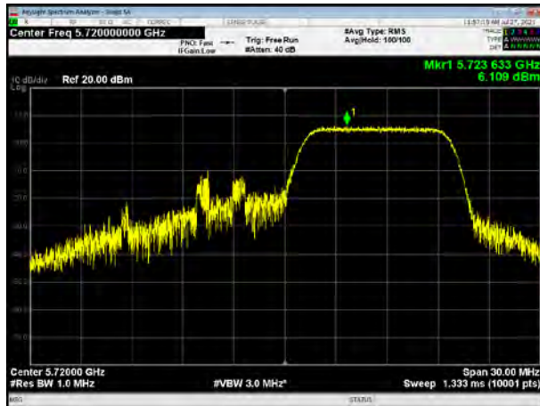
802.11ax HE20 106Tone: 5720
