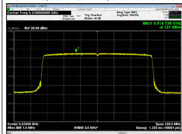
U-NII-2C, 802.11ax HE80, Channel No.: 106
