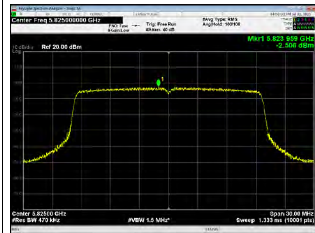
U-NII-3, 802.11ax HE20, Channel No.: 165
