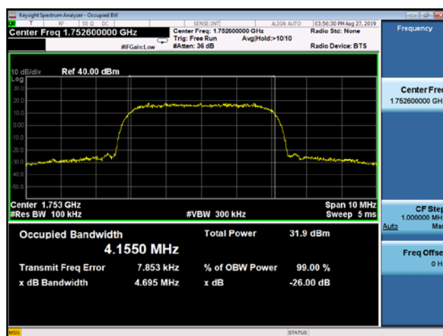
(Plot G2: WCDMA 1700 MHz Channel = 1513 bandwidth)
