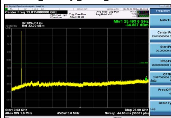
FDD02_LowRange_20MHz_30MHz~26GHz
