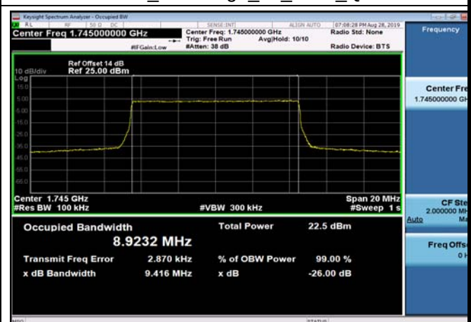
FDD66_MidRange_10_1745_Q16
