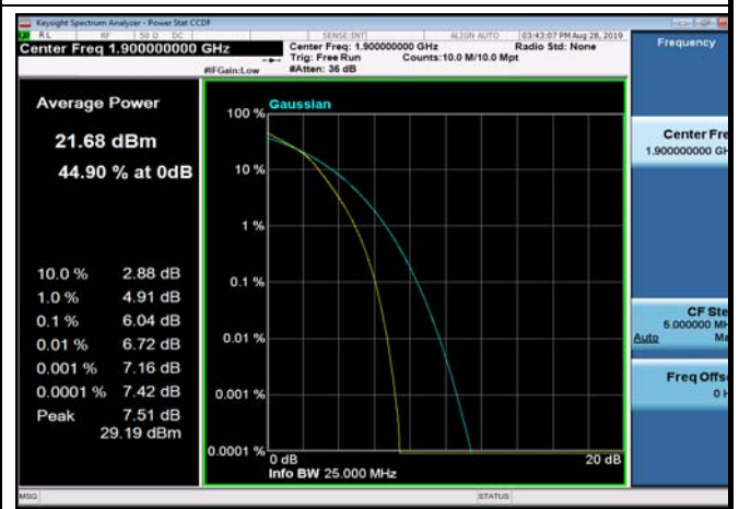
FDD02_HighRange_20MHz_1900_fullRB _Q16
