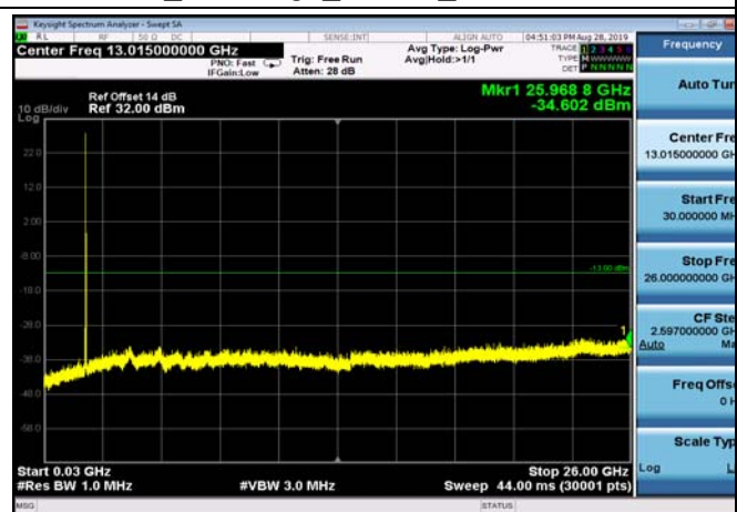
FDD02_MidRange_5MHz_30MHz~26GHz
