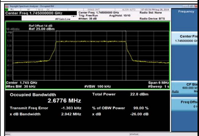
FDD66_MidRange_5_1745_Q16
