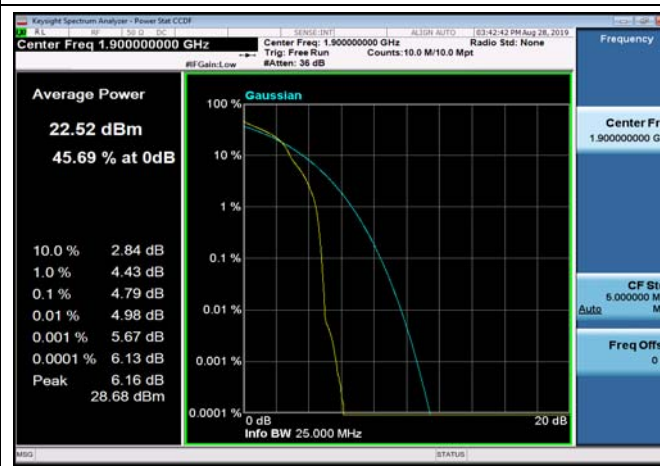
FDD02_HighRange_20MHz_1900_OneRB _high_Q16
