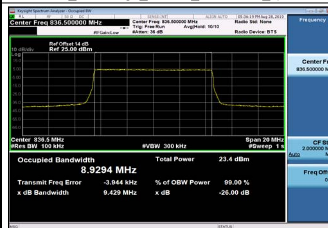
FDD05_MidRange_10MHz_836.5MHz_QPSK
