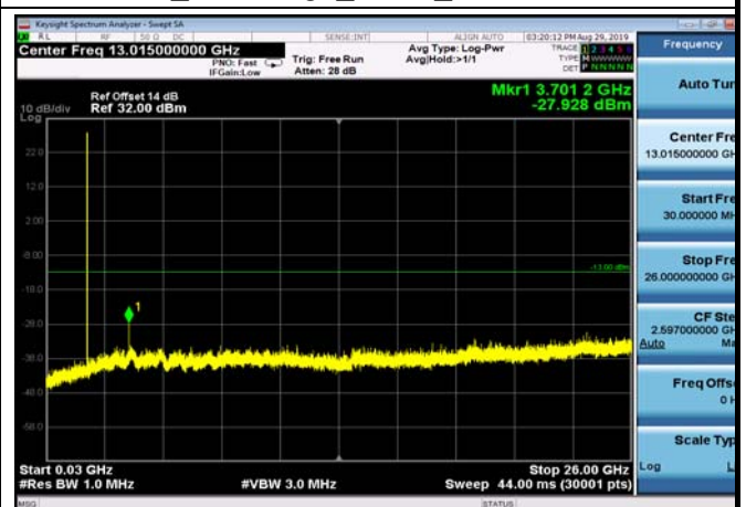
FDD02_LowRange_3MHz_30MHz~26GHz
