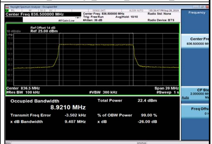
FDD05_MidRange_10MHz_836.5MHz_Q16
