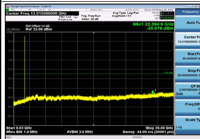
FDD02_LowRange_1.4MHz_30MHz~26GHz
