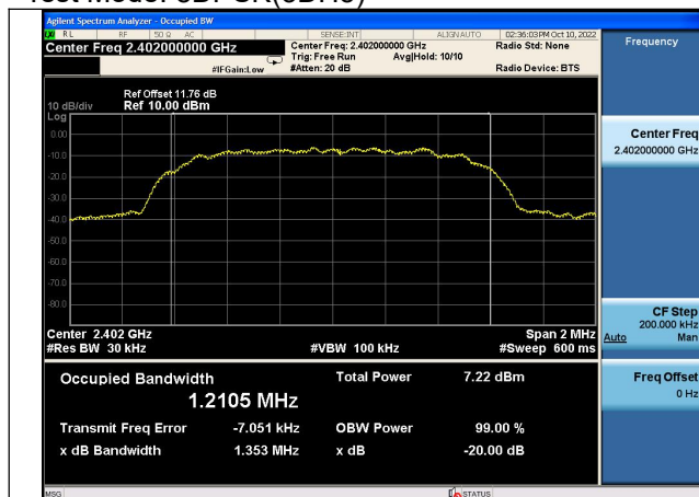
Test Mode:8DPSK(3DH5) 2402MHz
