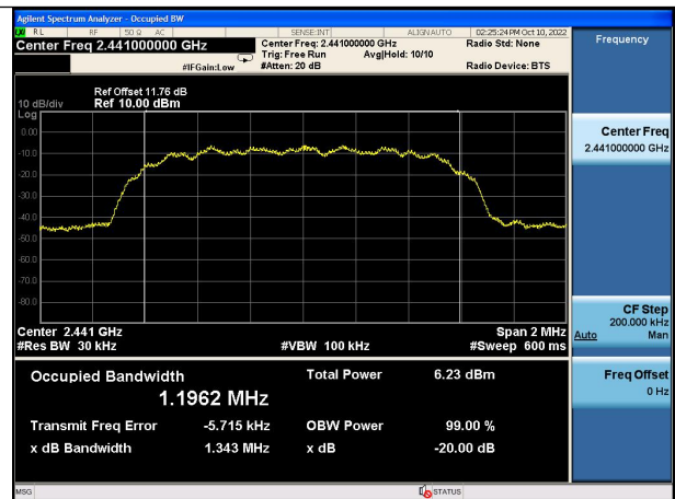
Test Mode: \pi/4 DQPSK(2DH5) 2441MHz
