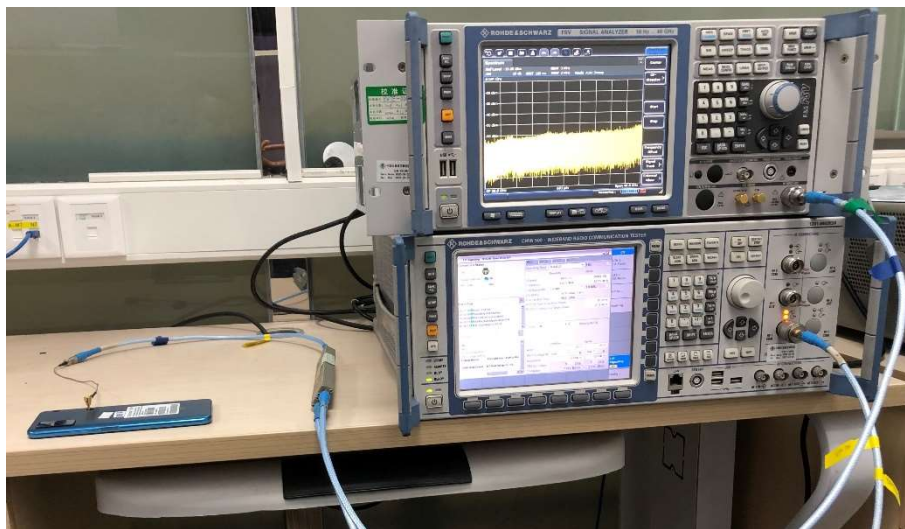
RF Conducted Test
