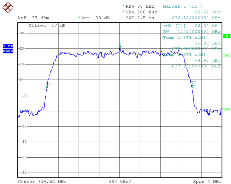
26dB Occupied Bandwidth Plot on Channel 384
