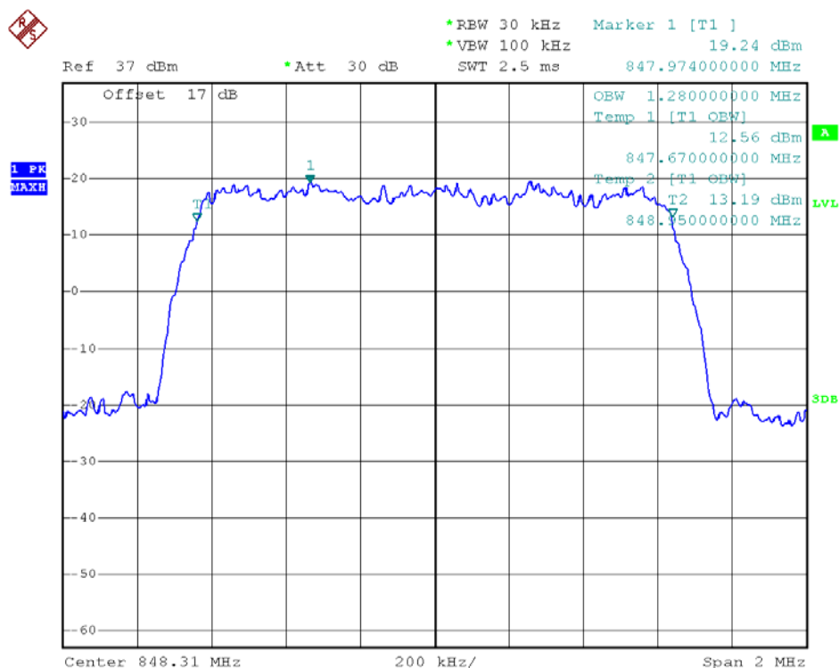
99% Occupied Bandwidth Plot on Channel 777
