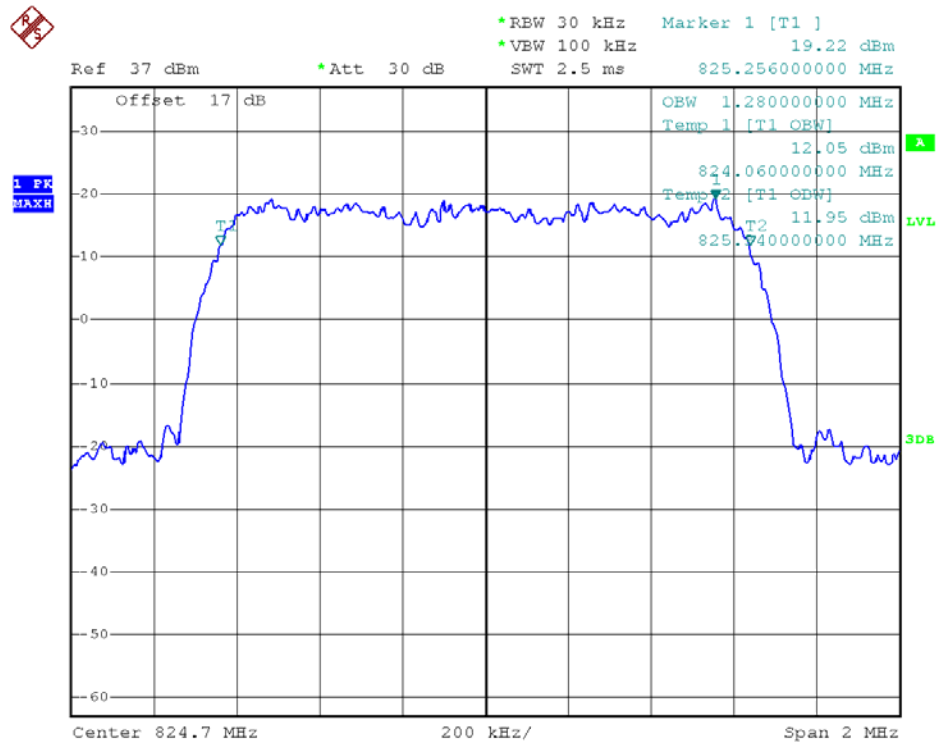
99% Occupied Bandwidth Plot on Channel 1013
