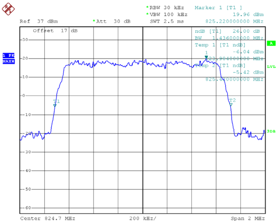
26dB Occupied Bandwidth Plot on Channel 1013
