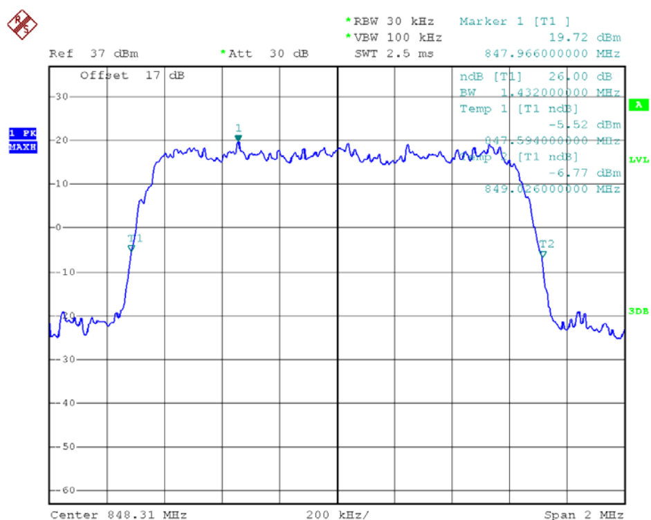
26dB Occupied Bandwidth Plot on Channel 777
