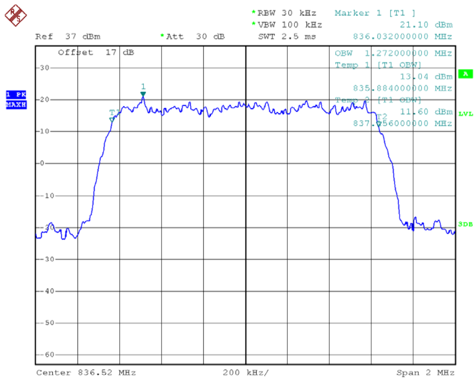
99% Occupied Bandwidth Plot on Channel 384
