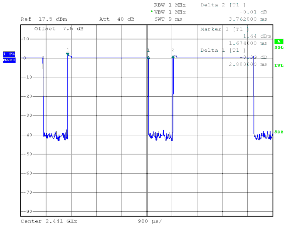
39 Channel @ 3DH5
