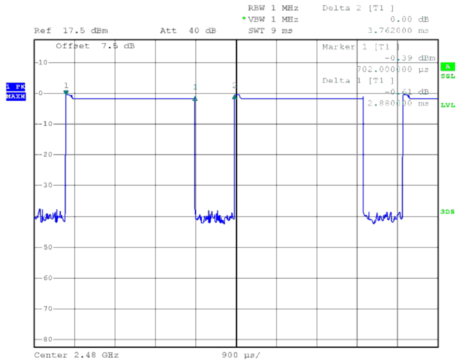
78 Channel @ 2DH5
