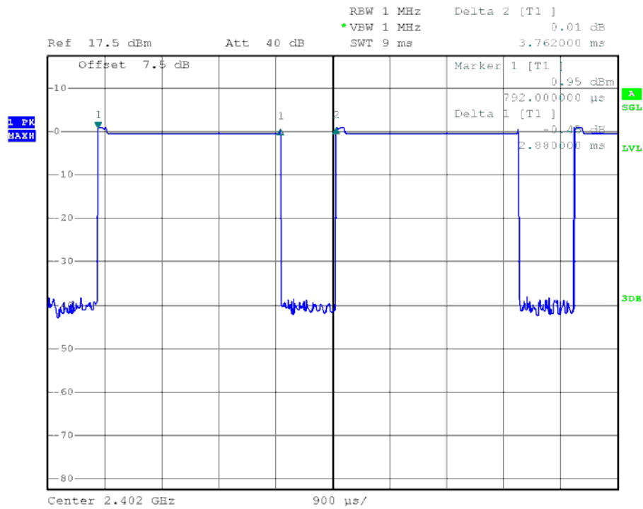
0 Channel @ 3DH5
