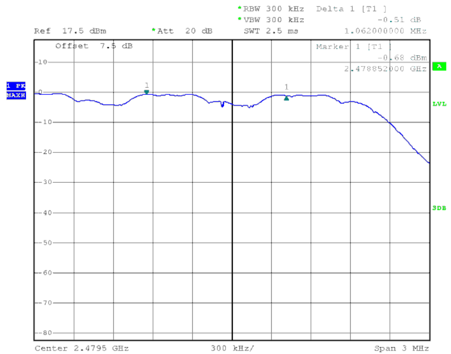
\pi/4 -DQPSK Mode, High Channel
