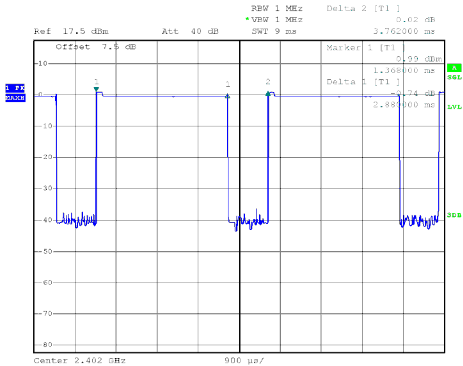
0 Channel @ 2DH5
