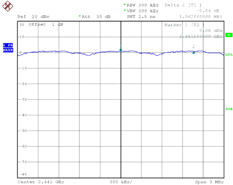
8-DPSK Mode, Middle Channel
