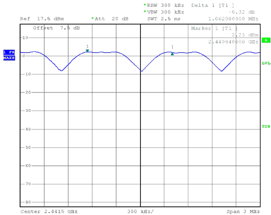
GFSK Mode, Mid Channel
