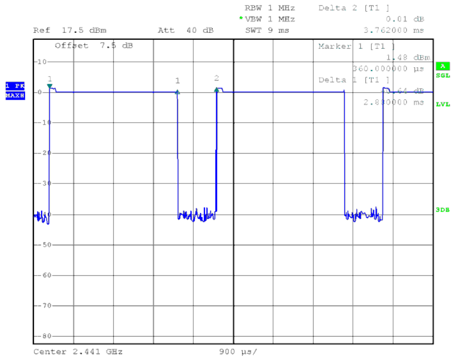
39 Channel @ 2DH5
