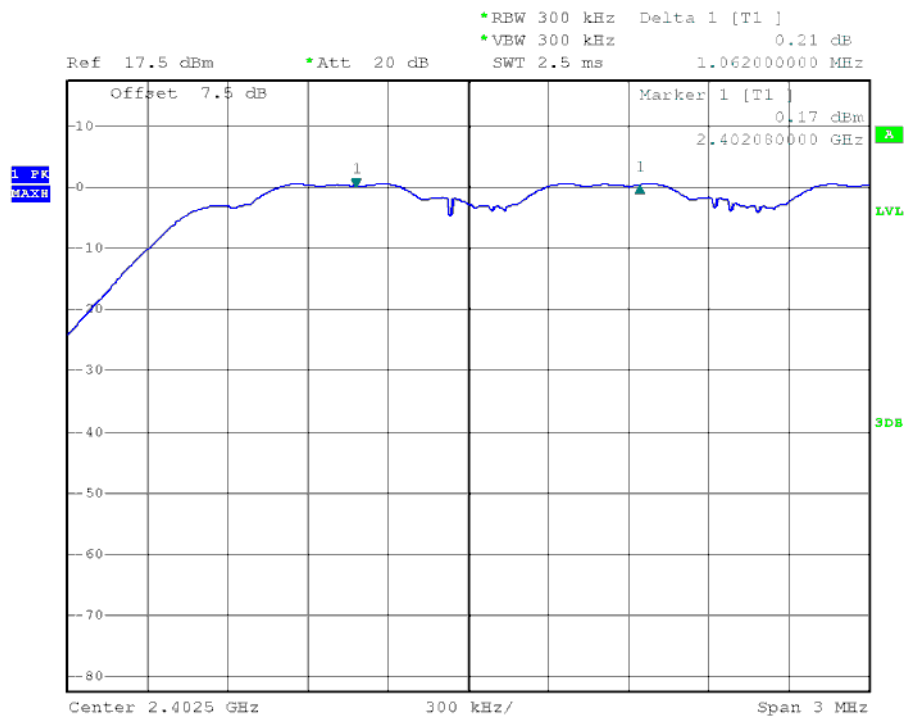
\pi/4 -DQPSK Mode, Low Channel
