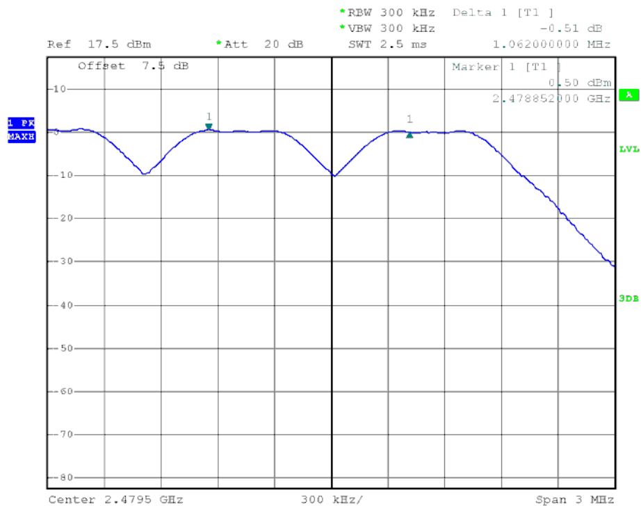
GFSK Mode, High Channel
