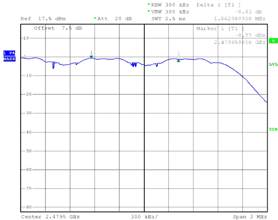
8-DPSK Mode, High Channel
