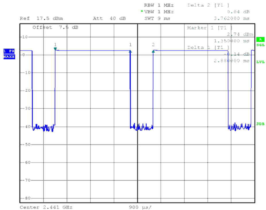
39 Channel @ DH5
