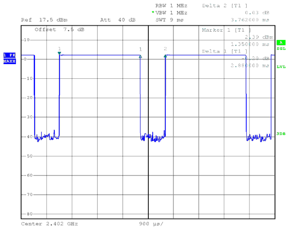
0 Channel @ DH5
