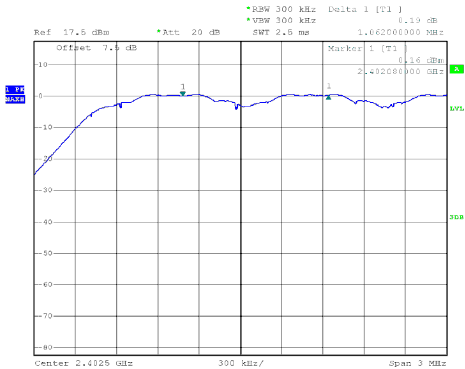
8-DPSK Mode, Low Channel
