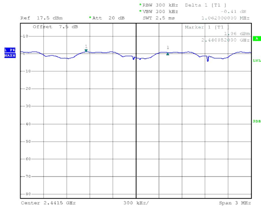
\pi/4 -DQPSK Mode, Middle Channel
