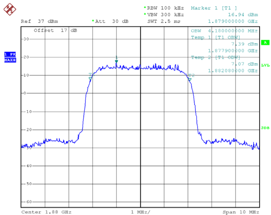
(Plot D4: WCDMA 1900MHz Channel = 9400 99% Occupied Bandwidth)
