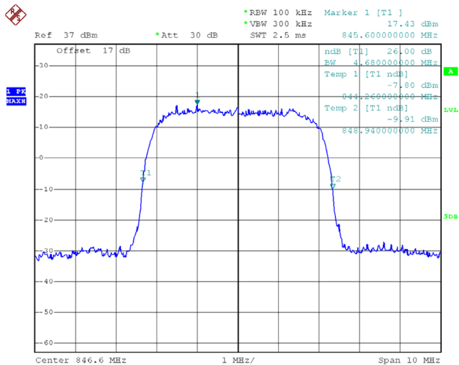
(Plot C5: WCDMA 850MHz Channel = 4233 26dB bandwidth)
