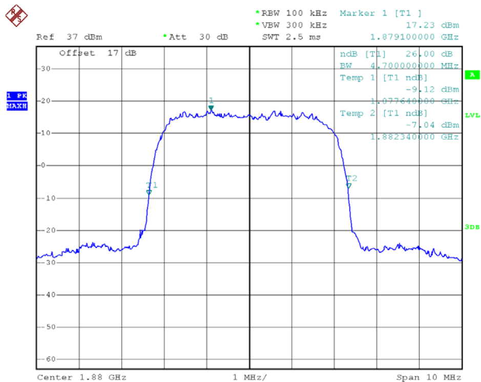
(Plot D3: WCDMA 1900MHz Channel = 9400 26dB bandwidth)
