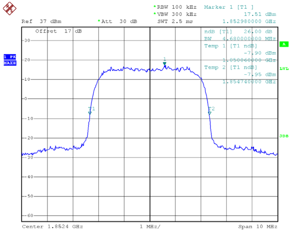
(Plot D1: WCDMA 1900MHz Channel = 9262 26dB bandwidth)
