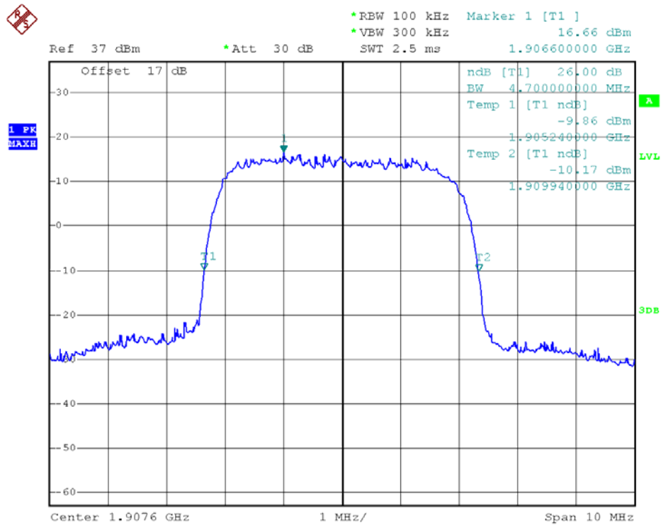
(Plot D5: WCDMA 1900MHz Channel = 9538 26dB bandwidth)
