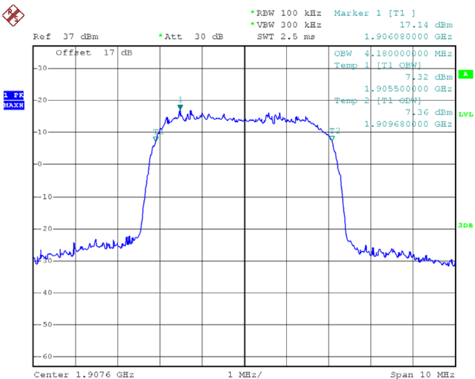
(Plot D6: WCDMA 1900MHz Channel = 9538 99% Occupied Bandwidth)
