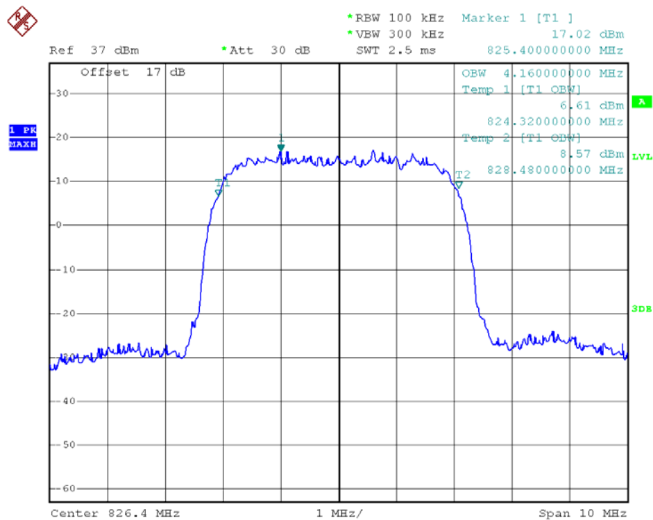
(Plot C2: WCDMA 850MHz Channel = 4132 99% Occupied Bandwidth)
