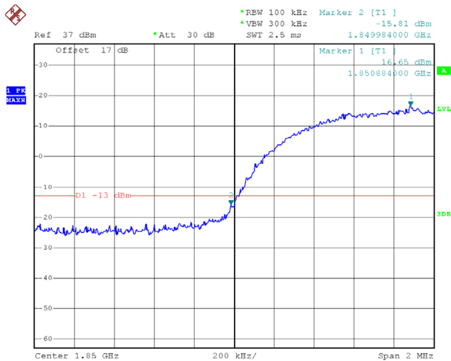
(Plot G: WCDMA 1900 Channel = 9262)
