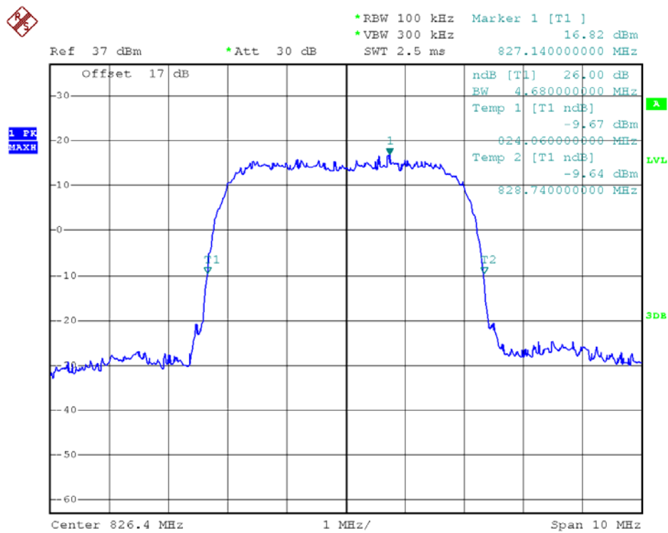
(Plot C1: WCDMA 850MHz Channel = 4132 26dB bandwidth)
