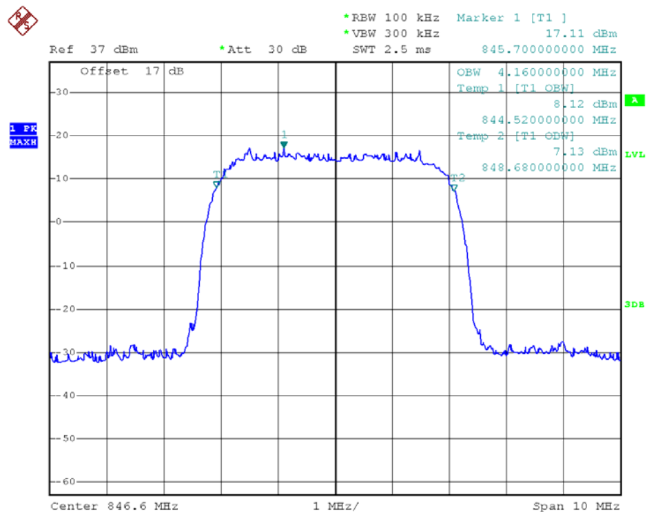
(Plot C6: WCDMA 850MHz Channel = 4233 99% Occupied Bandwidth)
