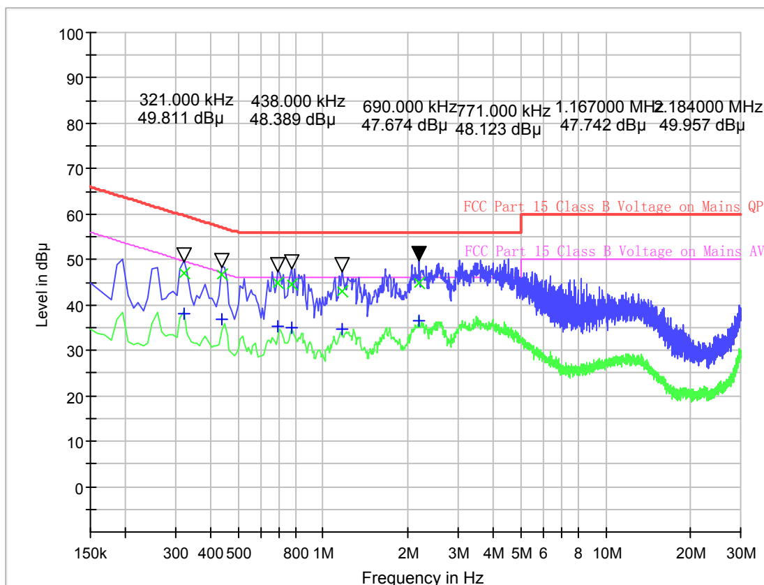
FCC Part 15 Class B Voltage Test
