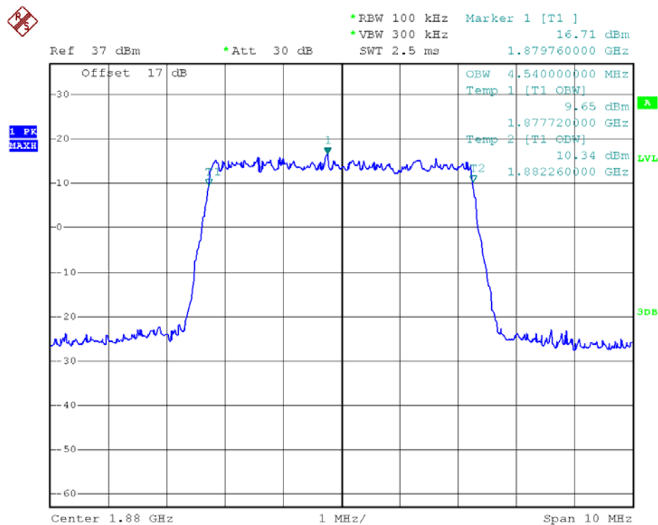
(Plot C1: 99% Occupied Bandwidth LTE Band 2/5MHz/QPSK)
