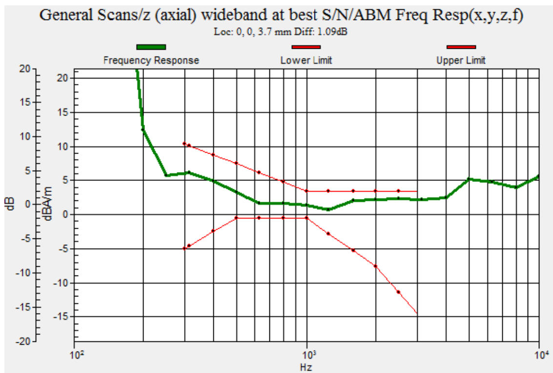
Figure 18 T-Coil WCDMA Band IV Z Axial
