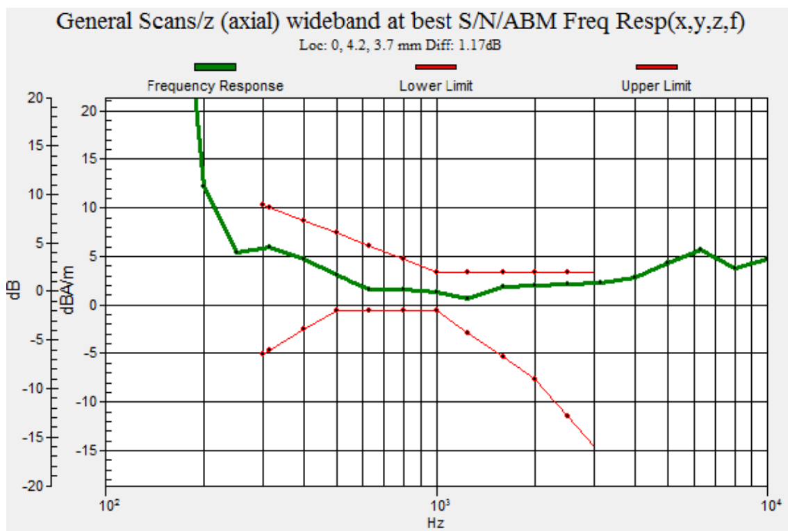
Figure 16 T-Coil WCDMA Band II Z Axial
