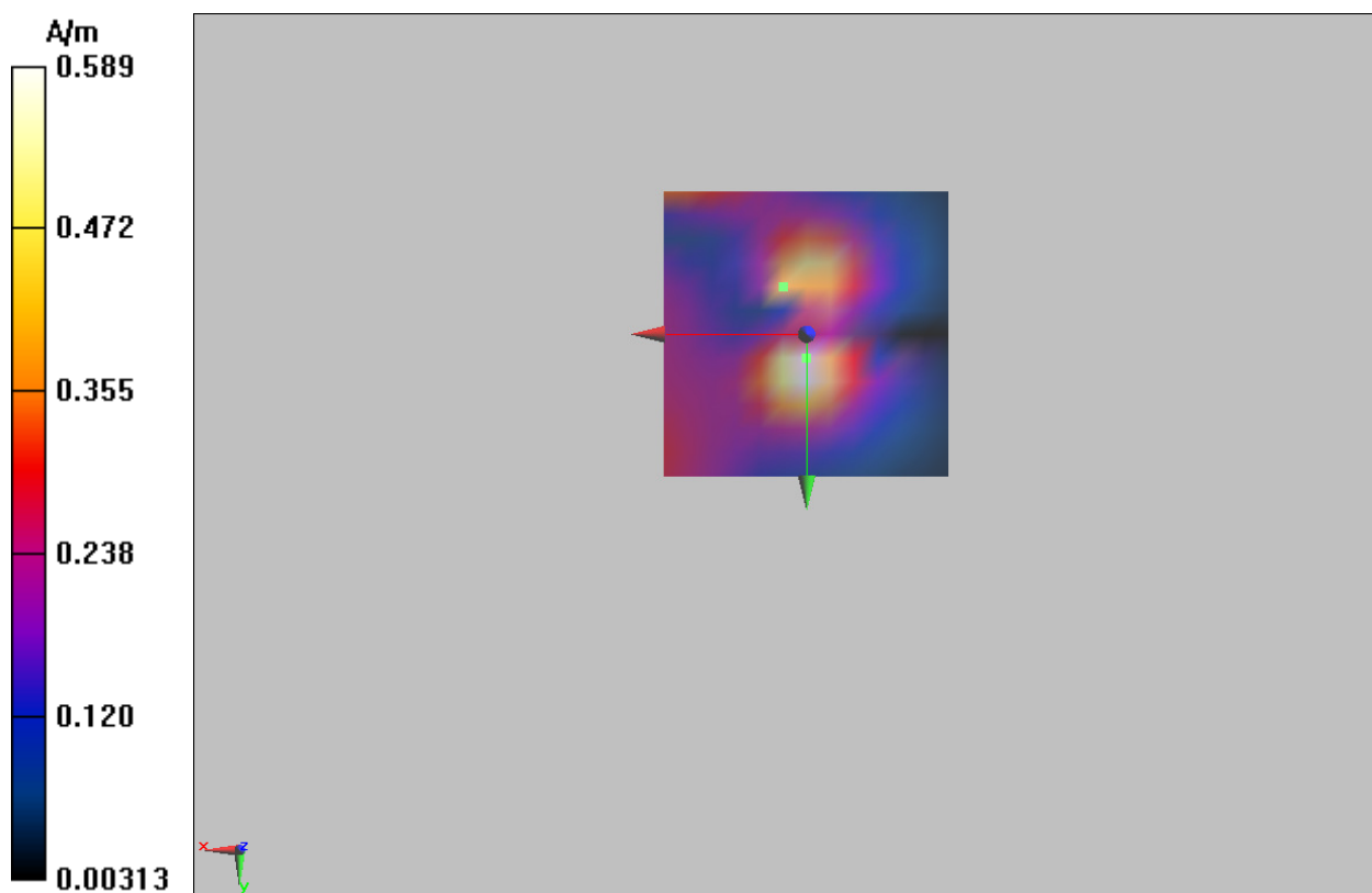
Figure 11 T-Coil GSM 850 Y transversal
