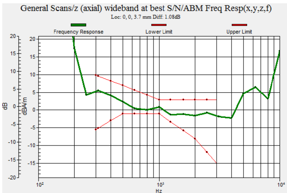
Figure 22 T-Coil CDMA BC0 Z Axial
