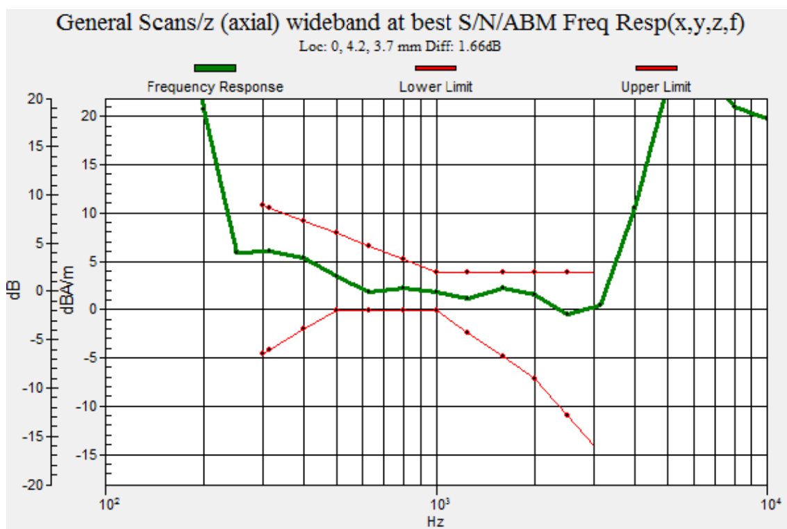
Figure 14 T-Coil GSM 1900 Z Axial
