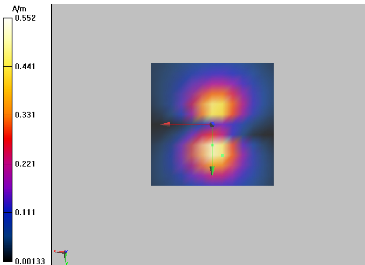
Figure 15 T-Coil WCDMA Band II Y transversal
