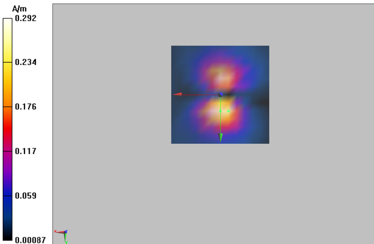
Figure 21 T-Coil CDMA BC0 Y transversal
