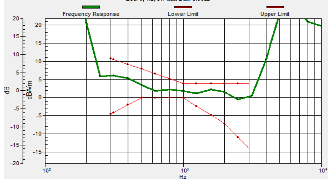
General Scans/z (axial) wideband at best S/N/ABM Freq Resp(x,y,z,f)
