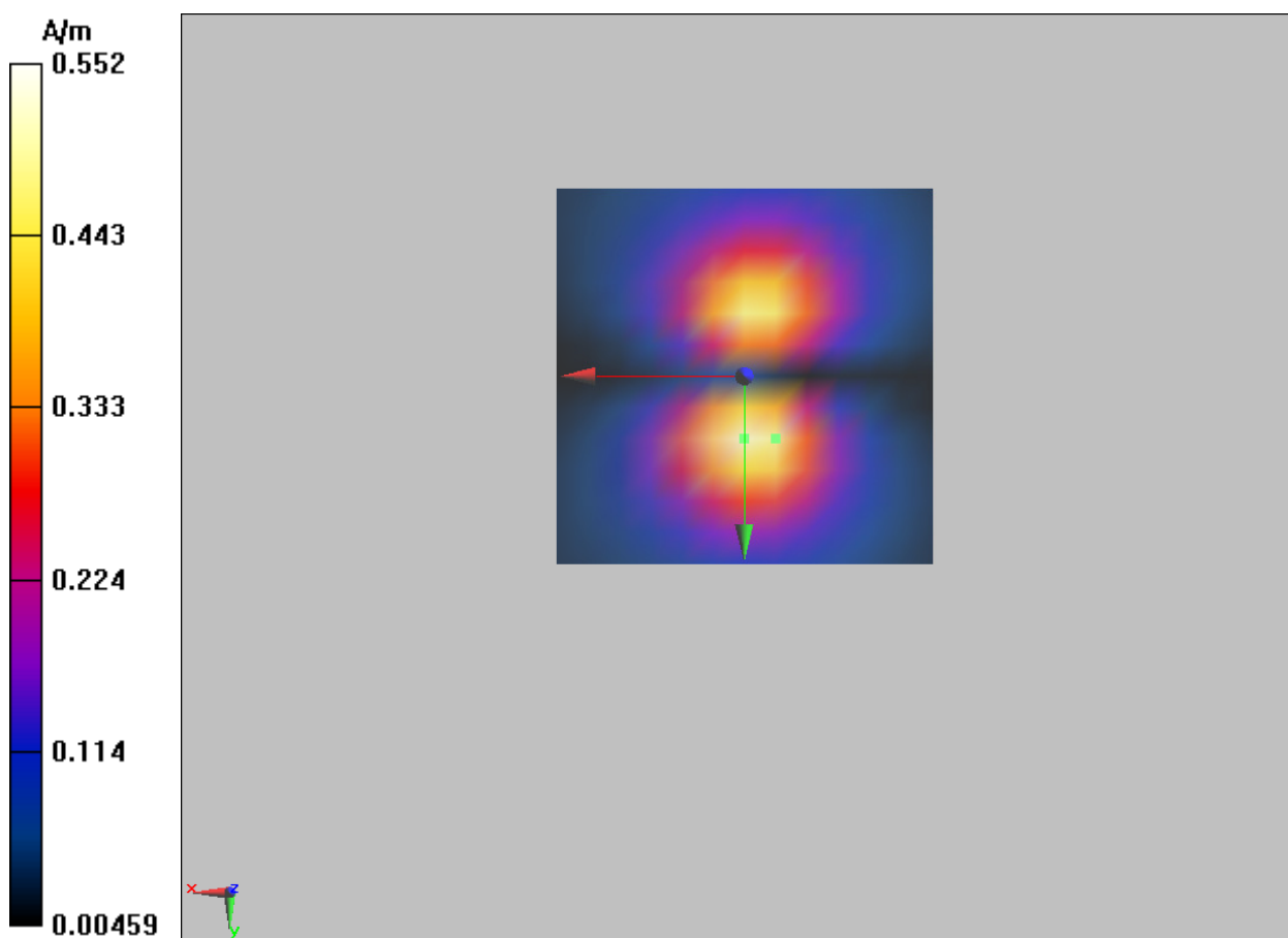
Figure 19 T-Coil WCDMA Band V Y transversal
