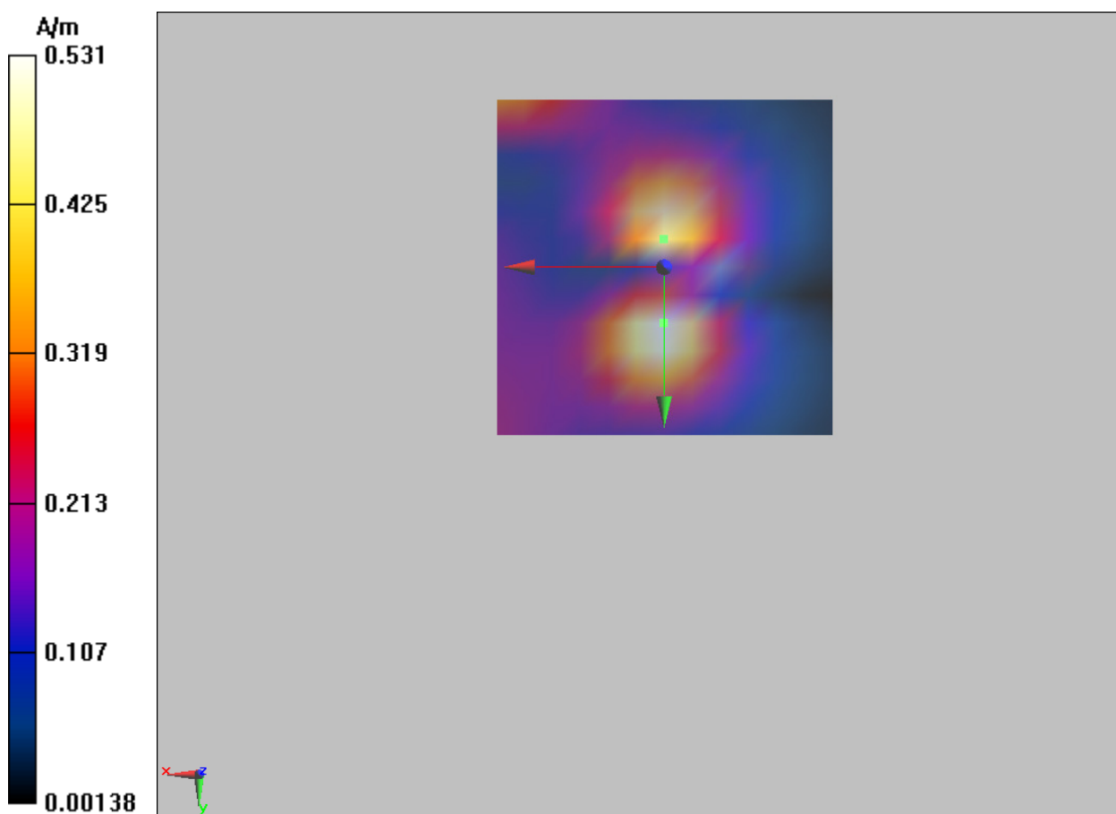
Figure 13 T-Coil GSM 1900 Y transversal
