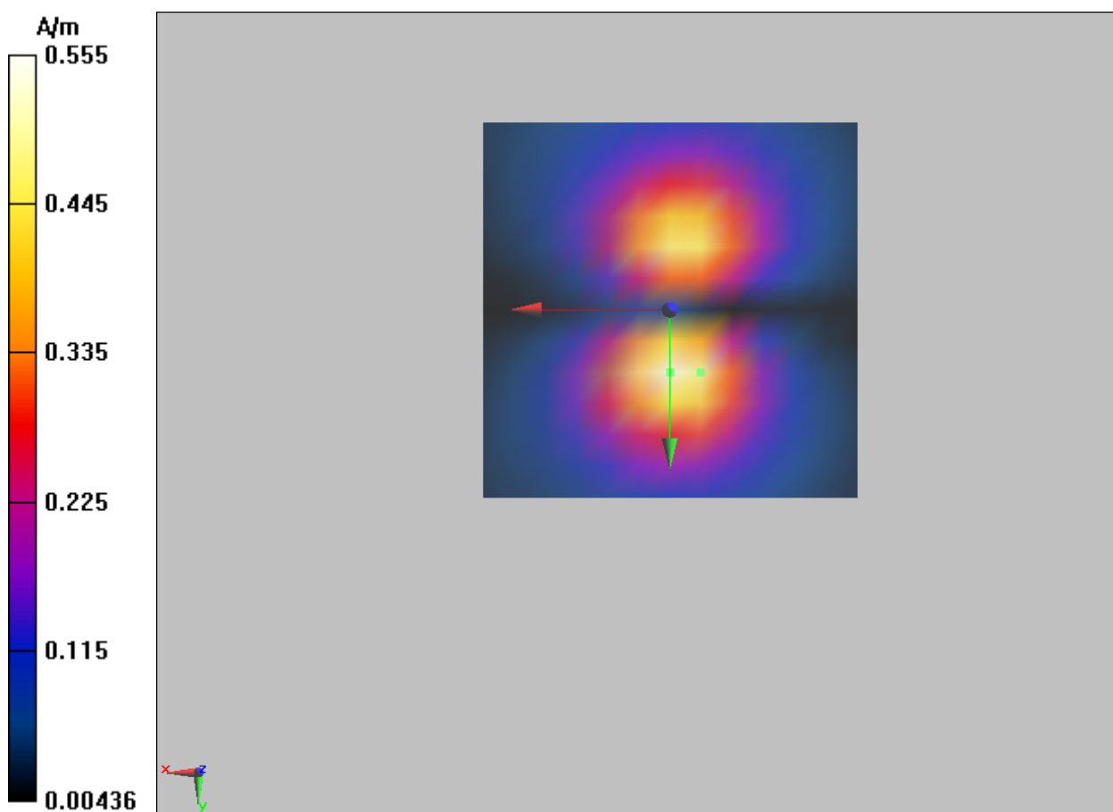
Figure 17 T-Coil WCDMA Band IV Y transversal
