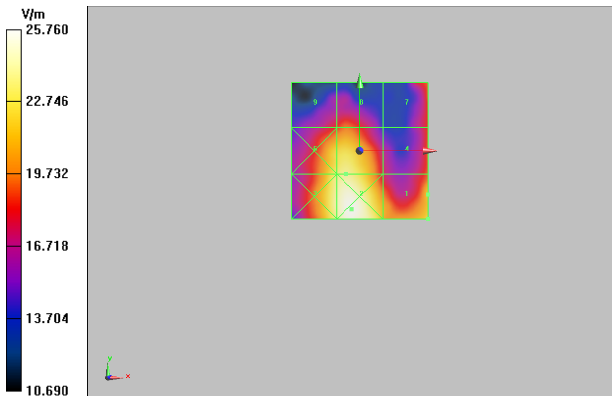
Figure 11 HAC RF E-Field GSM 1900 Channel 810
