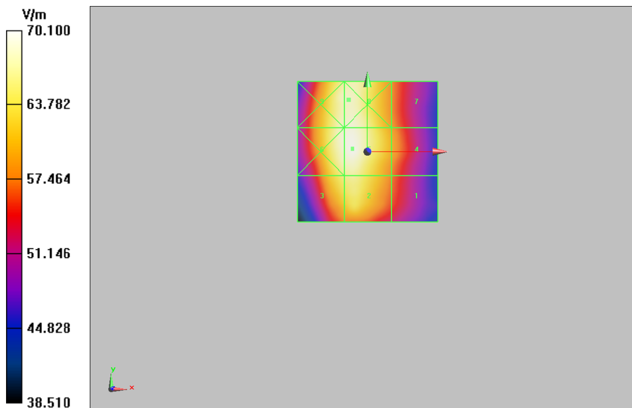
Figure 14 HAC RF E-Field CDMA BC0 Channel 777
