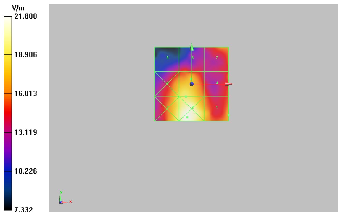
Figure 13 HAC RF E-Field GSM 1900 Channel 512
