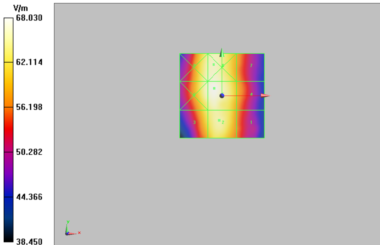
Figure 15 HAC RF E-Field CDMA BC0 Channel 384
