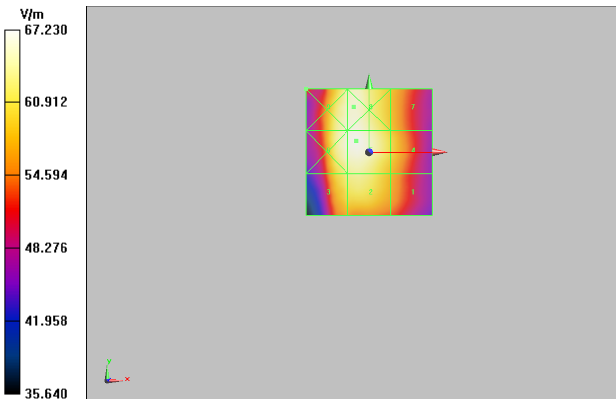
Figure 16 HAC RF E-Field CDMA BC0 Channel 1013
