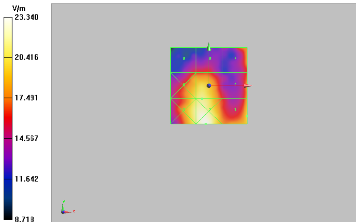
Figure 12 HAC RF E-Field GSM 1900 Channel 661
