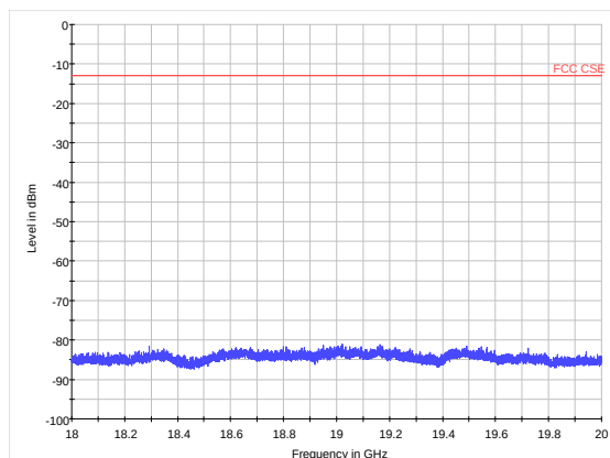
LTE Band 2 15MHz CH-Middle 18GHz~20GHz
