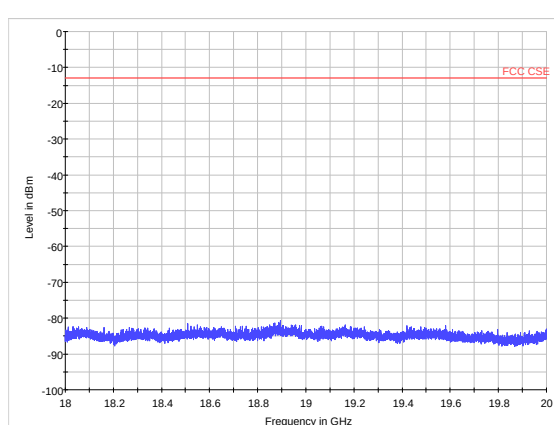
GSM 1900 CH-High 18GHz~20GHz
