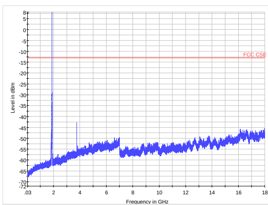
WCDMA Band II CH-High 30MHz~18GHz
