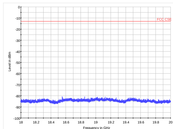
LTE Band 2 10MHz CH-Low 18GHz~20GHz
