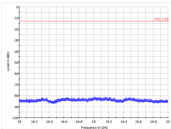
LTE Band 2 15MHz CH-Low 18GHz~20GHz
