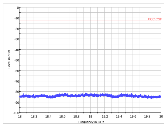
WCDMA Band II CH-High 18GHz~20GHz
