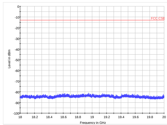
WCDMA Band II CH-Middle 18GHz~20GHz
