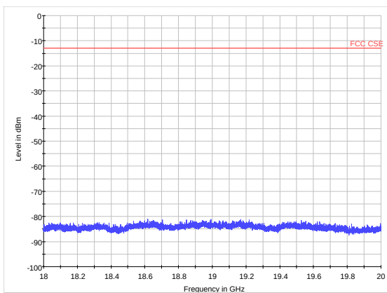
LTE Band 2 1.4MHz CH-Low 18GHz~20GHz
