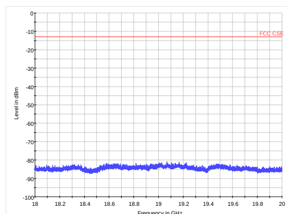
LTE Band 2 10MHz CH-High 18GHz~20GHz
