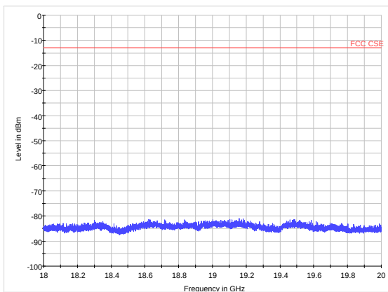
LTE Band 2 5MHz CH-High 18GHz~20GHz
