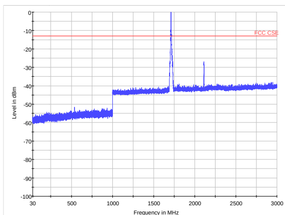
LTE Band 4 CH19975 30MHz~3GHz
