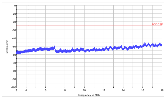
LTE Band 7 15MHz CH41515 3GHz~18GHz
