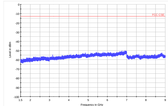
LTE Band 12 3MHz CH23025 1.5GHz~9GHz
