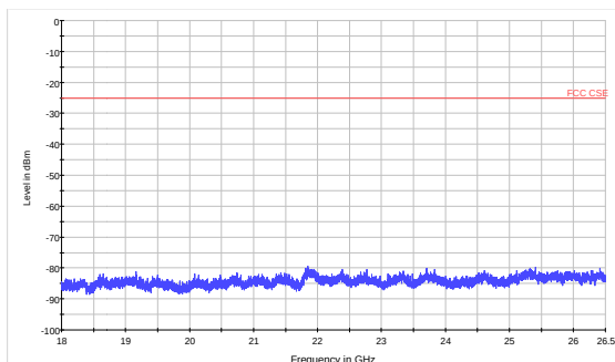
LTE Band 7 5MHz CH20775 18GHz~26.5GHz
