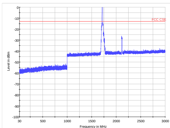
LTE Band 4 CH20025 30MHz~3GHz
