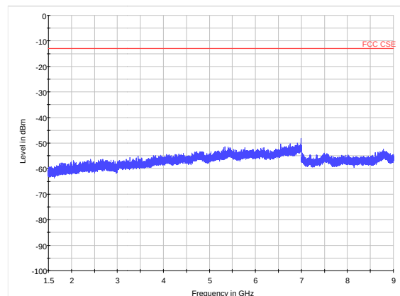
LTE Band 17 5MHz CH23825 1.5GHz~9GHz
