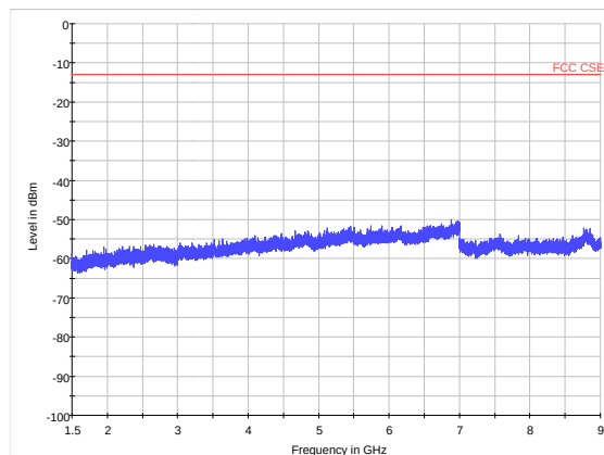
LTE Band 12 5MHz CH23035 1.5GHz~9GHz
