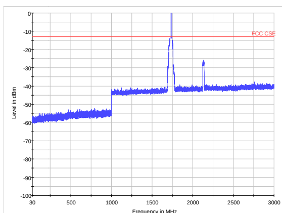
LTE Band 4 CH20175 30MHz~3GHz
