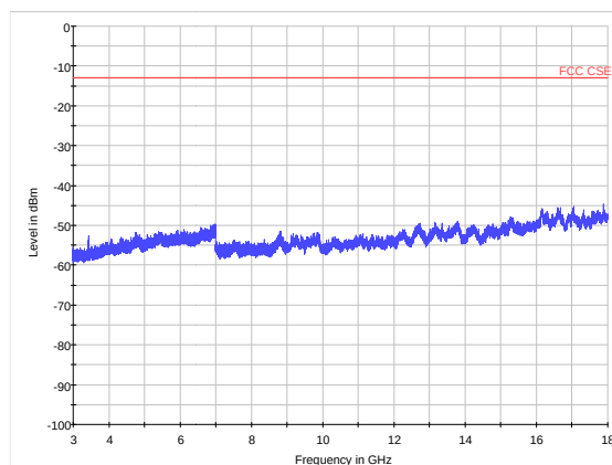
LTE Band 4 CH20025 3GHz~18GHz
