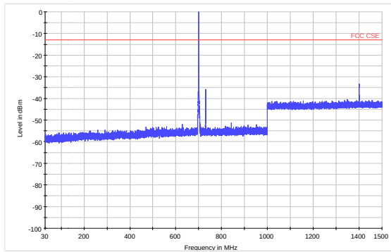
LTE Band 12 3MHz CH23025 30MHz~1.5GHz
