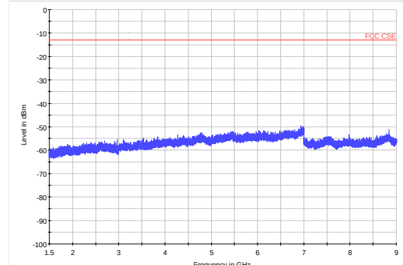
LTE Band 12 3MHz CH23095 1.5GHz~9GHz
