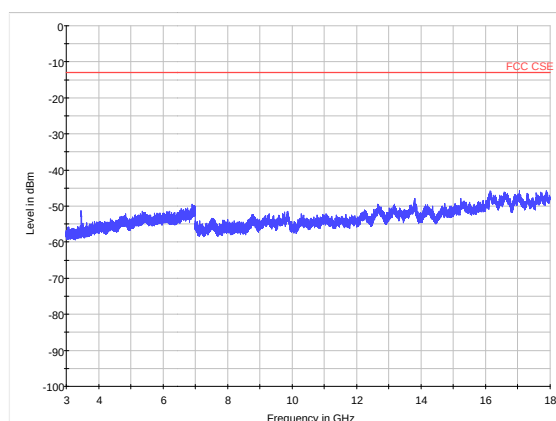
LTE Band 4 CH20175 3GHz~18GHz
