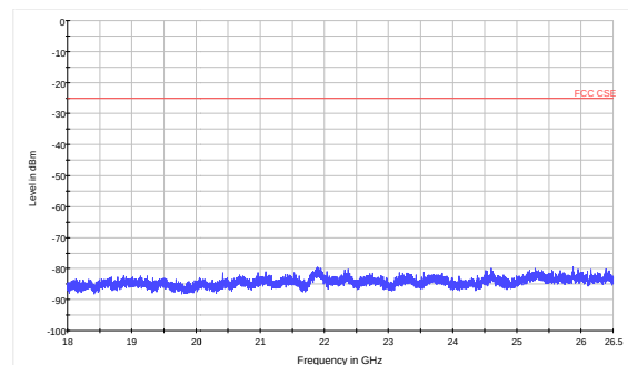
LTE Band 7 20MHz CH39750 18GHz~26.5GHz
