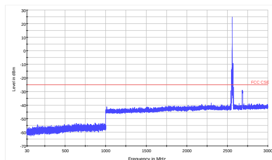
LTE Band 7 10MHz CH41540 30MHz~3GHz
