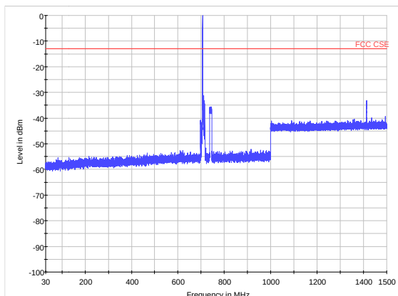
LTE Band 17 10MHz CH23800 30MHz~1.5GHz
