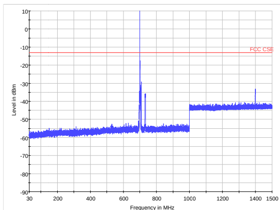
LTE Band 12 5MHz CH23035 30MHz~1.5GHz
