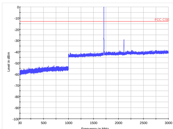
LTE Band 4 CH19957 30MHz~3GHz
