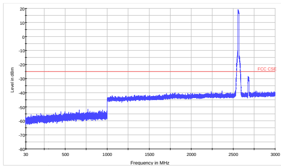
LTE Band 7 15MHz CH41515 30MHz~3GHz
