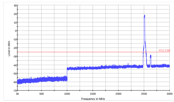
LTE Band 7 20MHz CH39750 30MHz~3GHz
