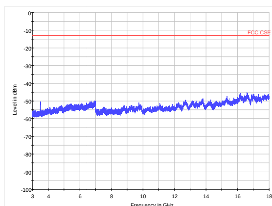
LTE Band 4 CH20385 3GHz~18GHz
