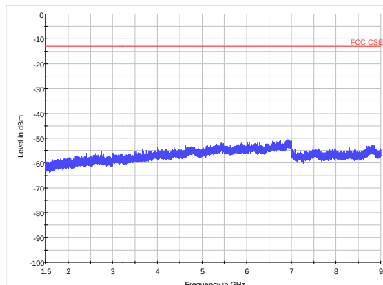
LTE Band 12 10MHz CH23060 1.5GHz~9GHz
