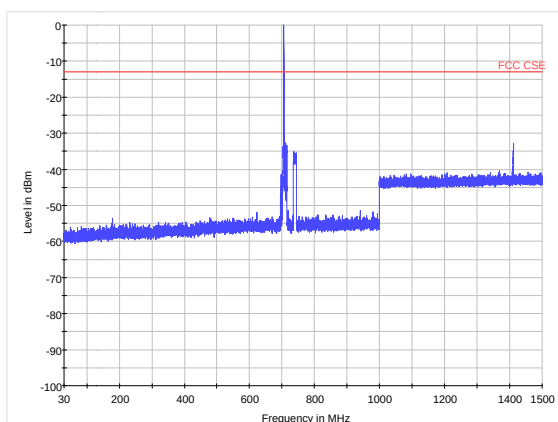
LTE Band 17 10MHz CH23790 30MHz~1.5GHz
