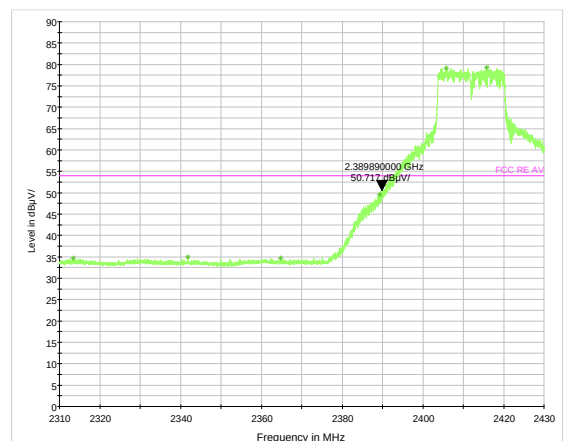
802.11g-Channel 1: Average
