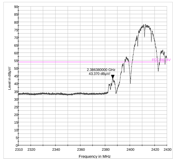
802.11b-Channel 1: Average
