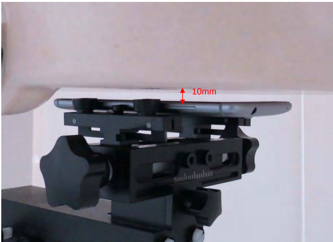
Picture 26: Front Side, the distance from handset to the bottom of the Phantom is 10mm (Variant)
