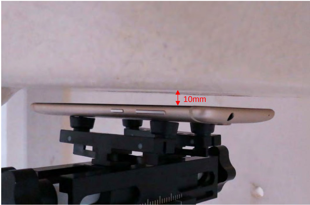
Picture 25: Front Side, the distance from handset to the bottom of the Phantom is 10mm (Original)
