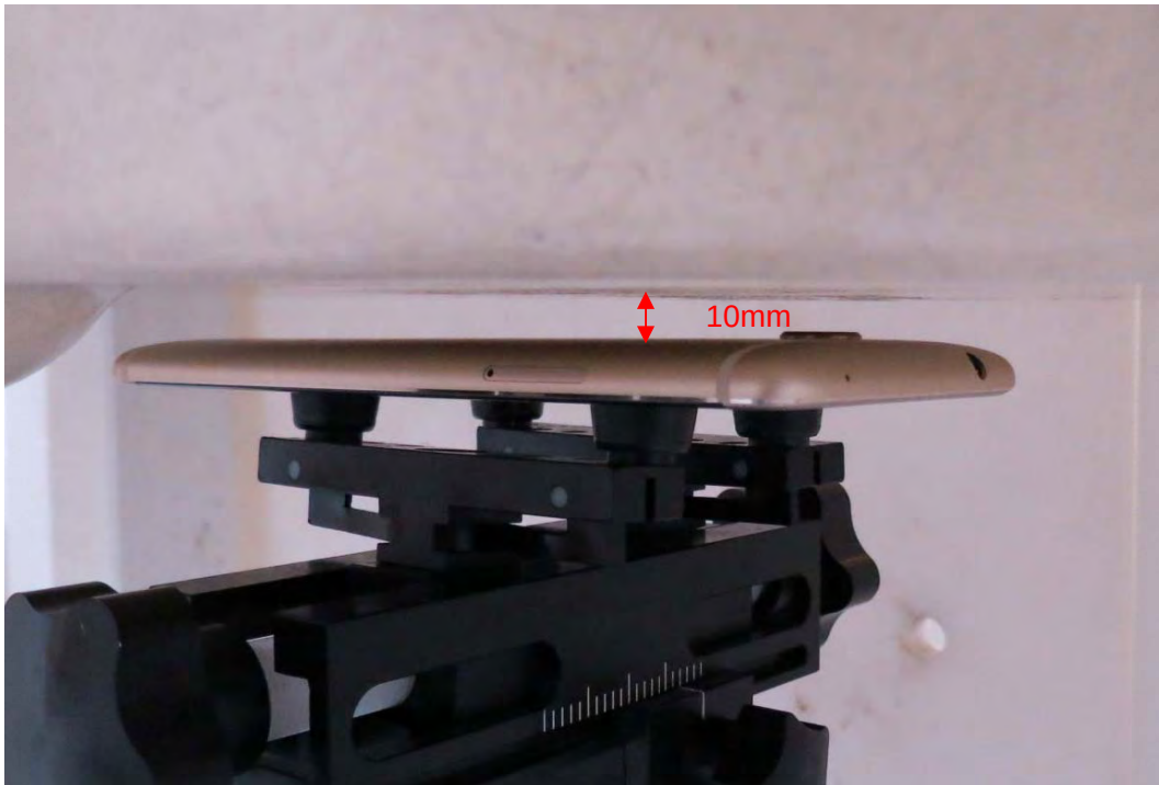
Picture 23: Back Side, the distance from handset to the bottom of the Phantom is 10mm (Original)
