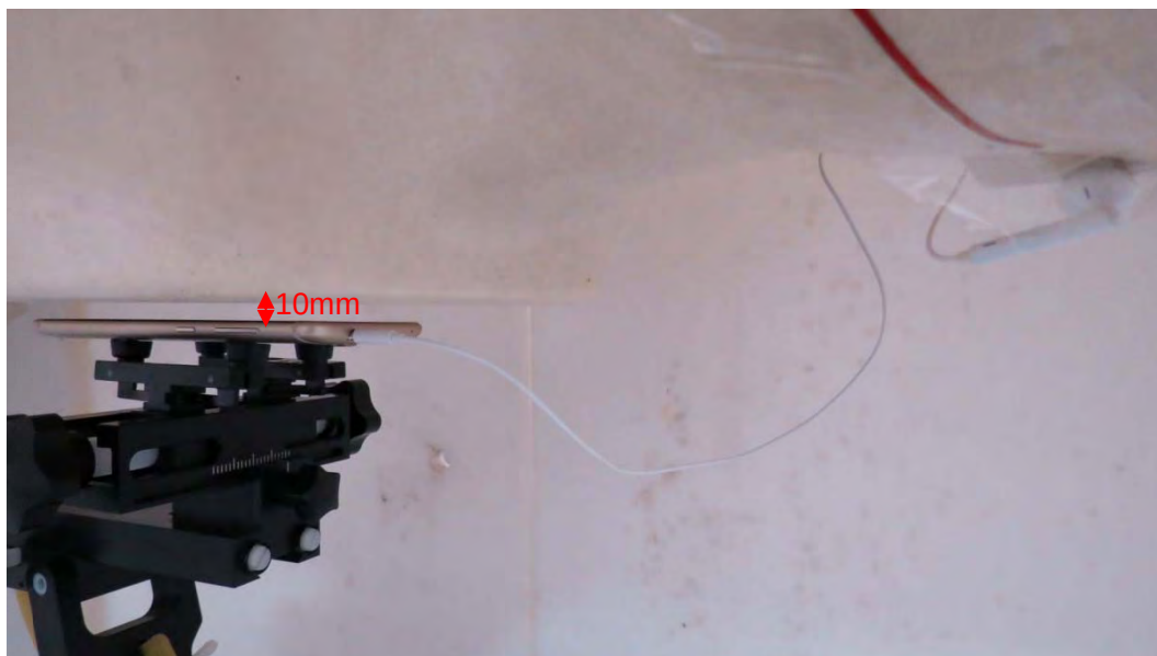
Picture 33: Front Side with Earphone, the distance from handset to the bottom of the Phantom is 10mm (Original)
