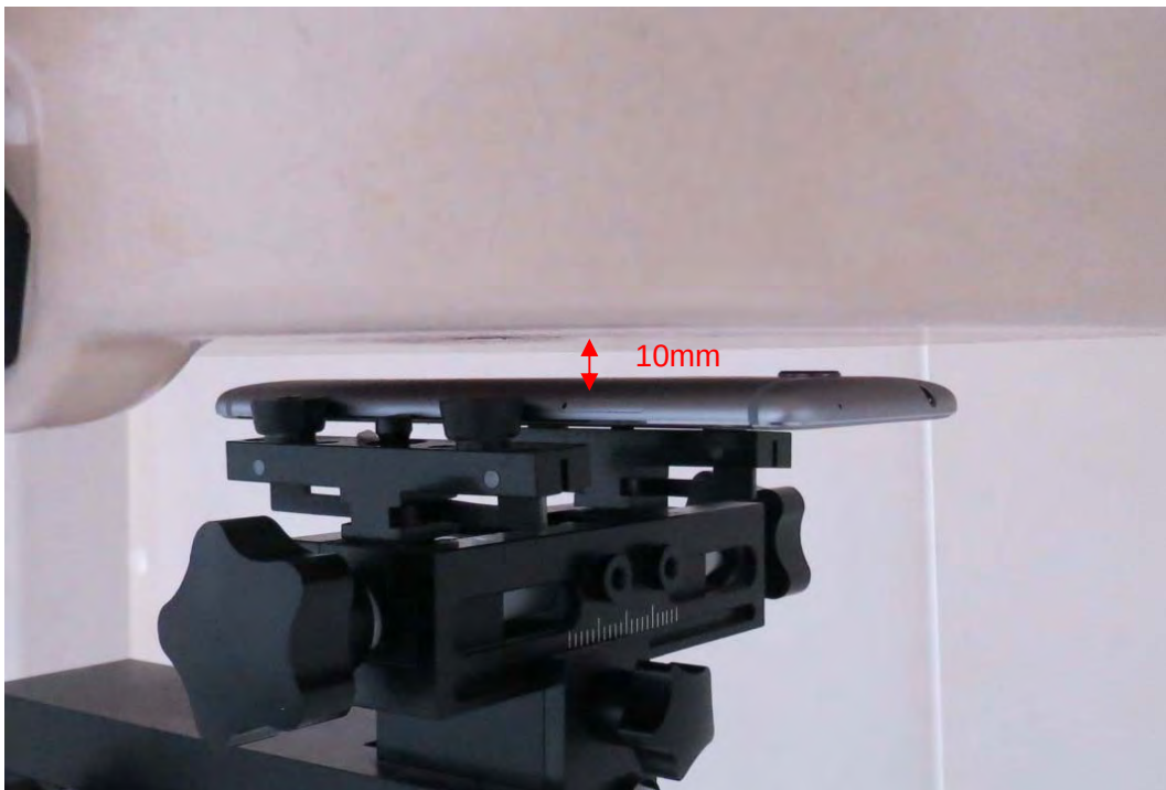
Picture 24: Back Side, the distance from handset to the bottom of the Phantom is 10mm (Variant)
