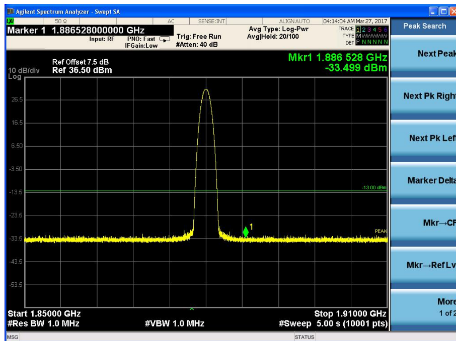
Channel 661, 1850MHz~1910MHz
