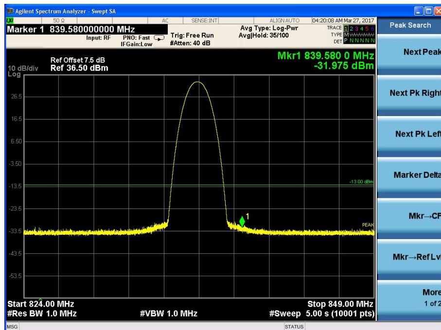
Channel 189, 824MHz~849MHz
