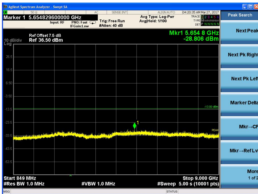
Channel 189, 849MHz~9GHz
