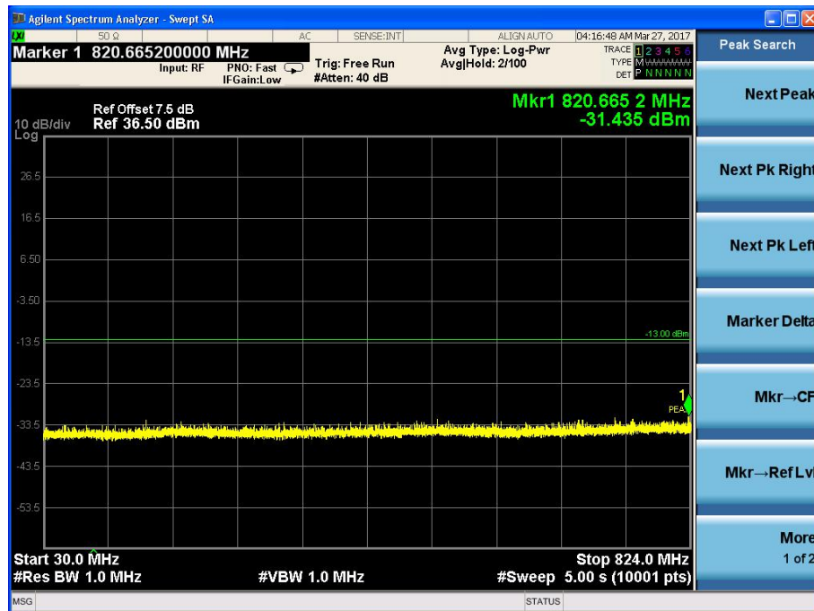
Channel 189, 30MHz~824MHz
