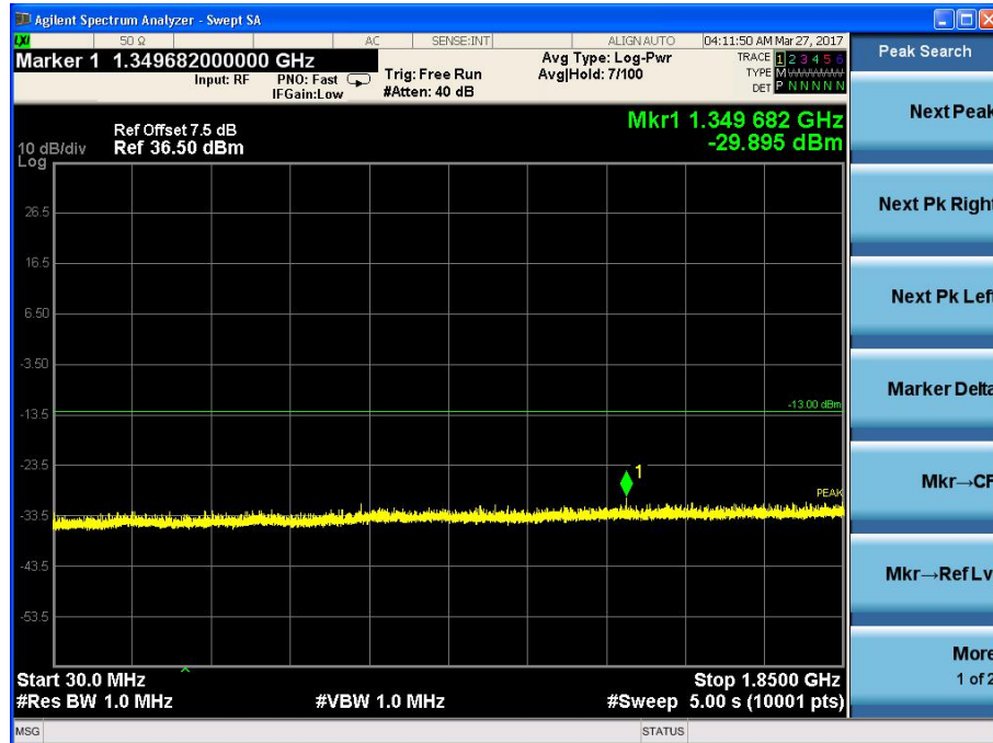
Channel 661, 30MHz~1850MHz
