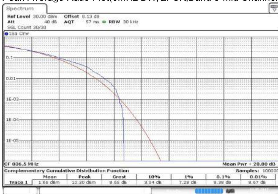
Peak-Average Ratio Plot(3MHz BW,QPSK,Band 5-mid Channel)
