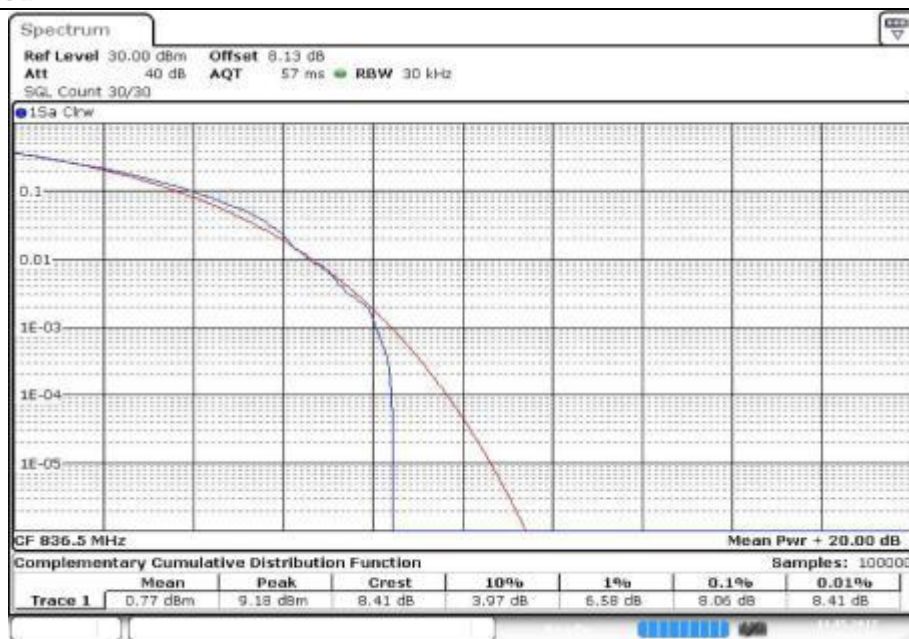
Peak-Average Ratio Plot(5MHz BW,QPSK,Band 5-mid Channel)
