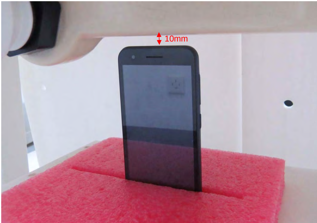
Picture 24: Top Side, the distance from handset to the bottom of the Phantom is 10mm
