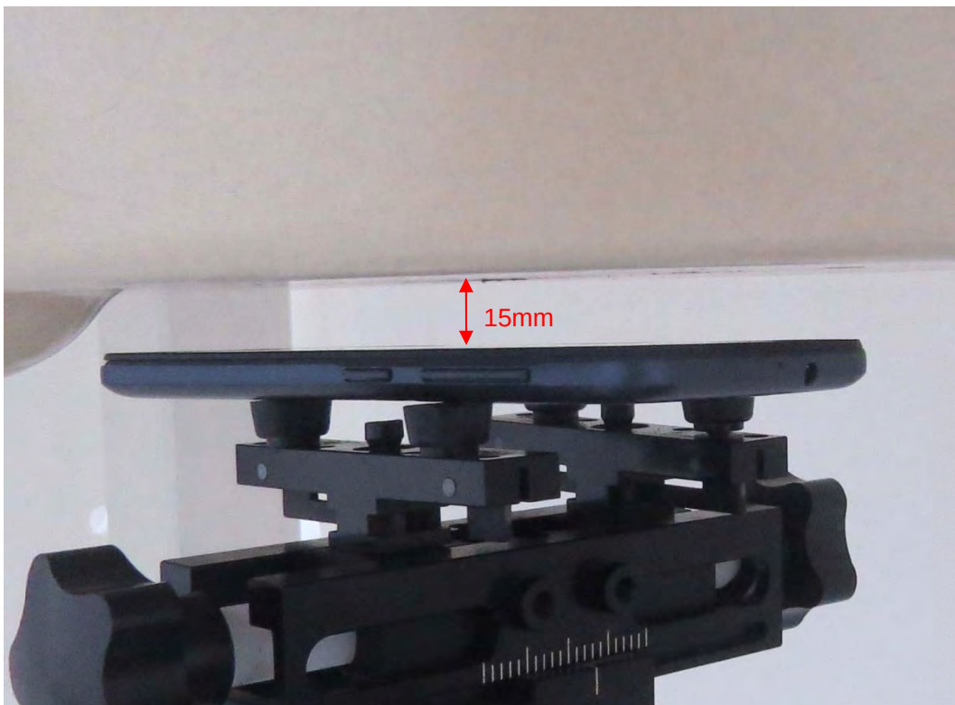
Picture 19: Front Side, the distance from handset to the bottom of the Phantom is 15mm
