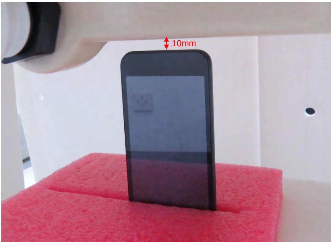
Picture 25: Bottom Side, the distance from handset to the bottom of the Phantom is 10mm
