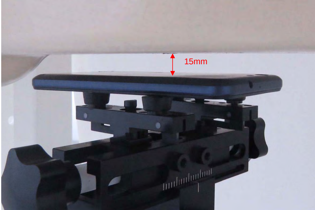
Picture 18: Back Side, the distance from handset to the bottom of the Phantom is 15mm
