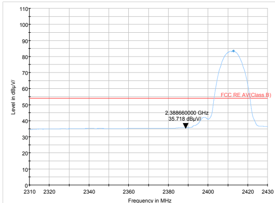
802.11b-Channel 1: Average
