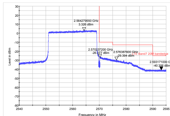
LTE Band 7 QPSK 20MHz CH-High, 100%RB
