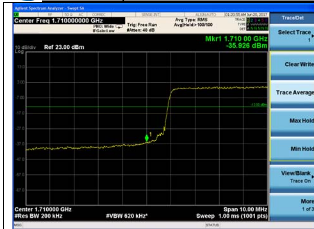
LTE Band 4 16QAM 1.4MHz CH-Low, 1 RB
