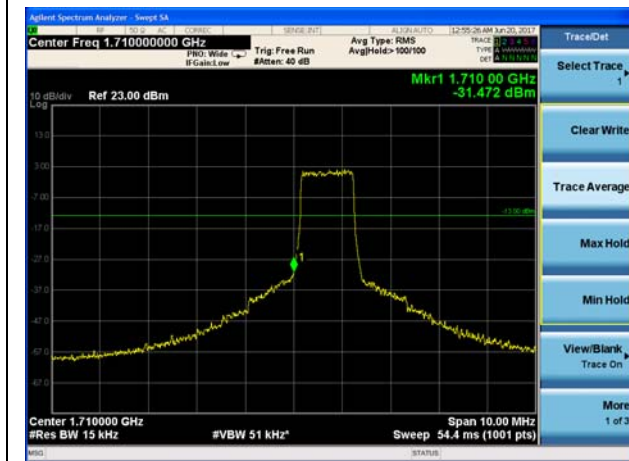
LTE Band 4 16QAM 1.4MHz CH-Low, 100%RB
