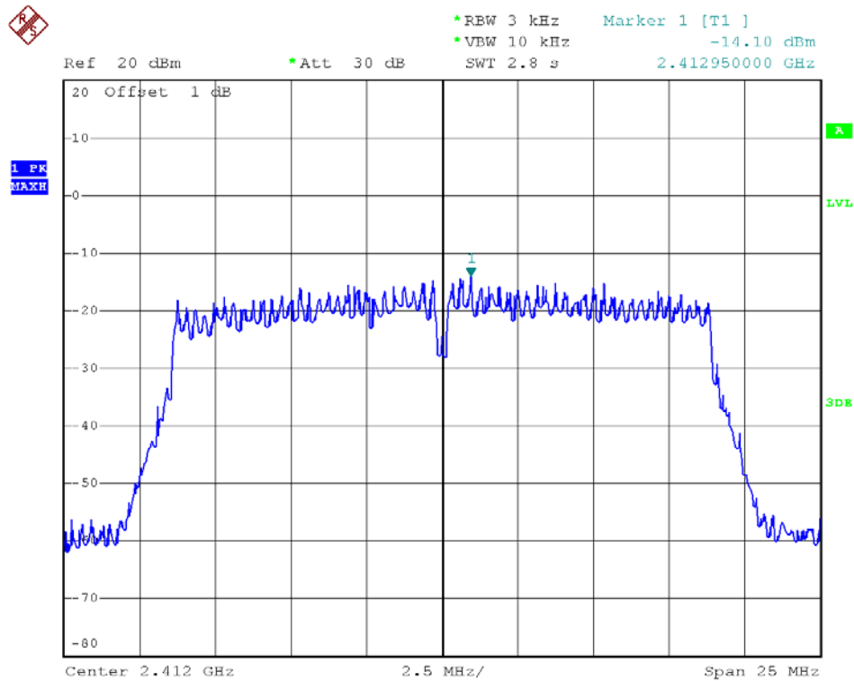
802.11n20 - Channel 1
