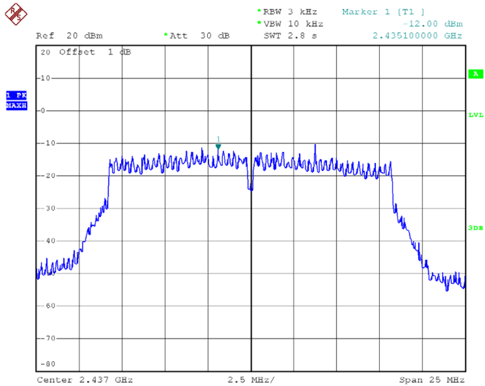
802.11g - Channel 6
