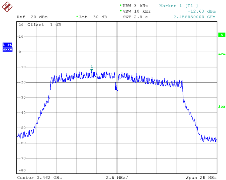
802.11g - Channel 11
