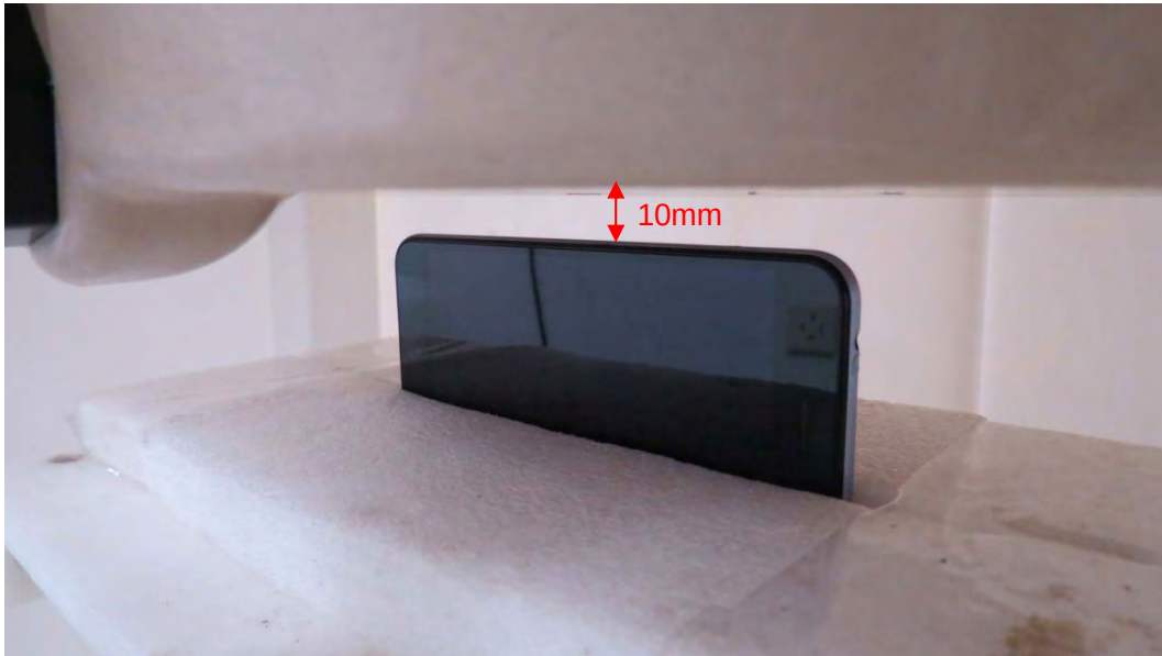
Picture 20: Left Side, the distance from handset to the bottom of the Phantom is 10mm
