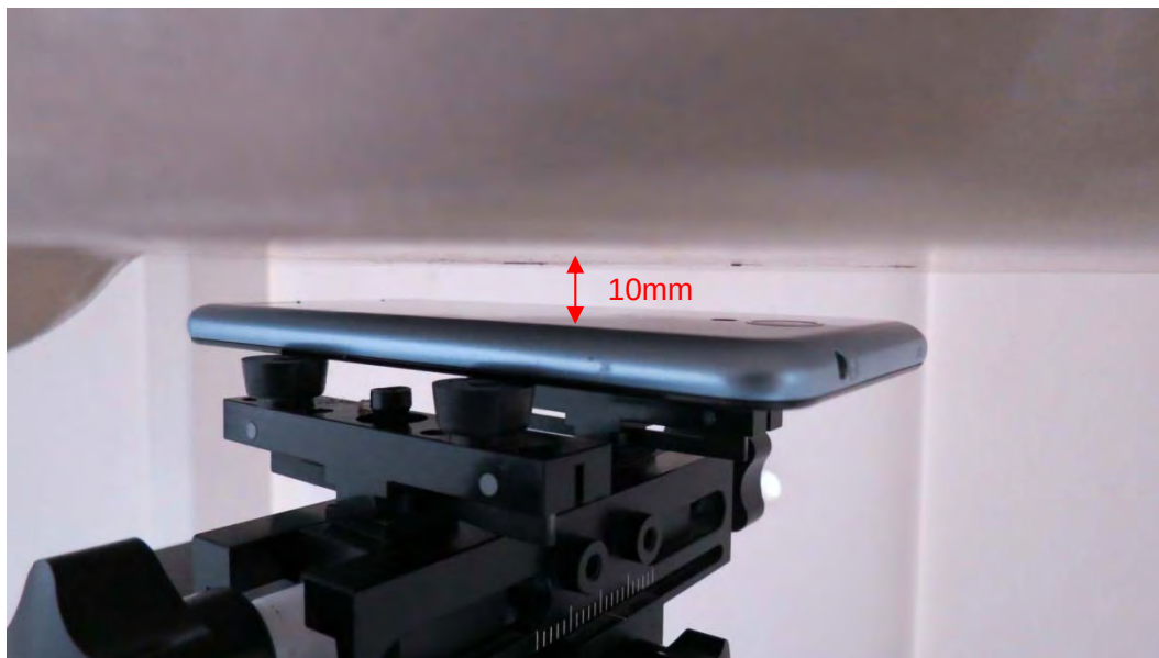
Picture 18: Back Side, the distance from handset to the bottom of the Phantom is 10mm
