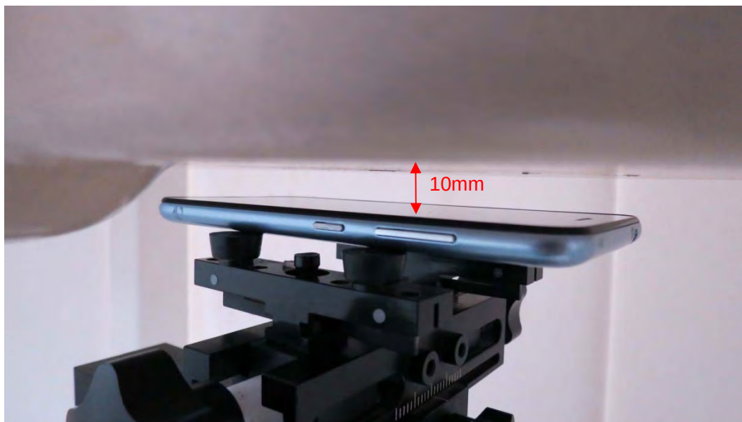
Picture 19: Front Side, the distance from handset to the bottom of the Phantom is 10mm
