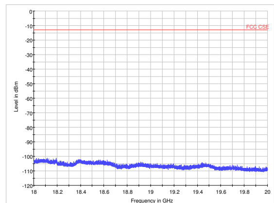
LTE Band 2 3MHz CH-High 18GHz~20GHz
