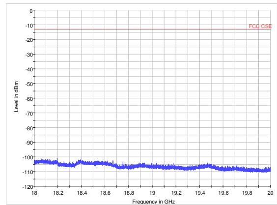
LTE Band 2 10MHz CH-Low 18GHz~20GHz
