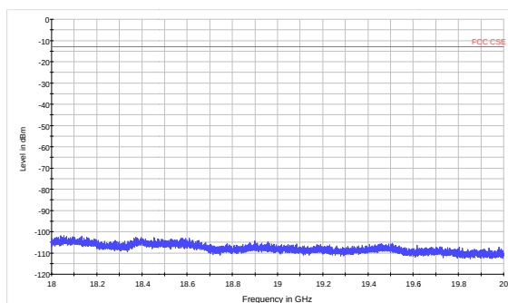
LTE Band 4 10MHz CH-High 18GHz~20GHz
