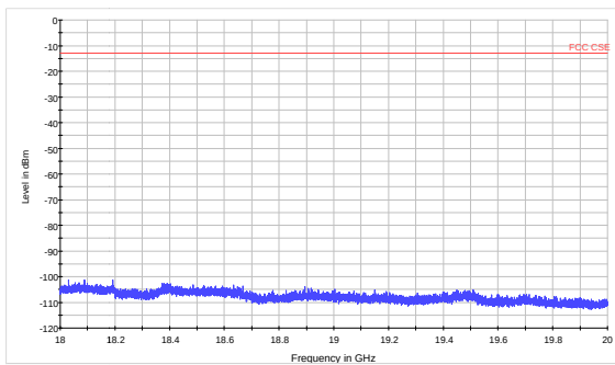
LTE Band 4 5MHz CH-High 18GHz~20GHz
