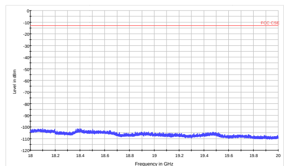
LTE Band 4 1.4MHz CH-Middle 18GHz~20GHz
