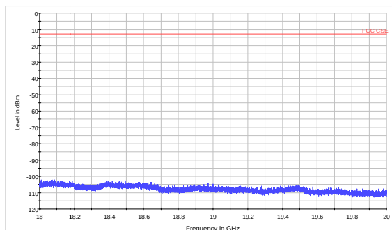
LTE Band 4 15MHz CH-High 18GHz~20GHz
