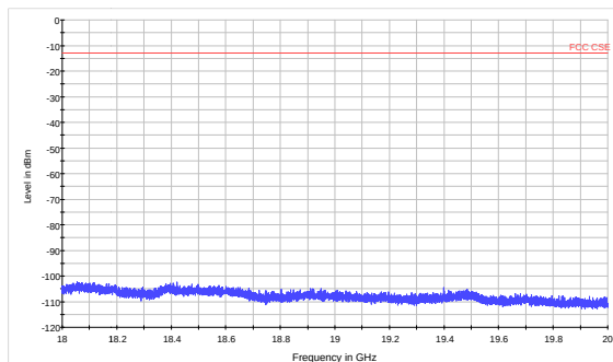
LTE Band 4 5MHz CH-Low 18GHz~20GHz
