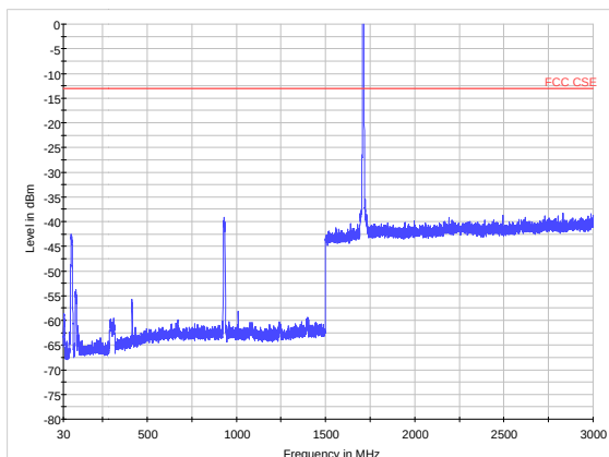
WCDMA Band IV CH-Middle 30MHz~3GHz
