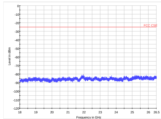
LTE Band 7 20MHz CH-High 18GHz~26.5GHz
