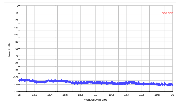
LTE Band 4 5MHz CH-Middle 18GHz~20GHz
