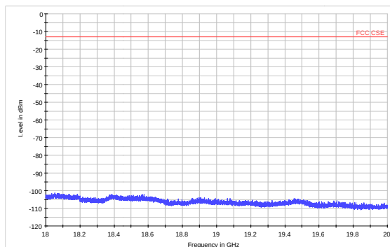
LTE Band 4 20MHz CH-Low 18GHz~20GHz
