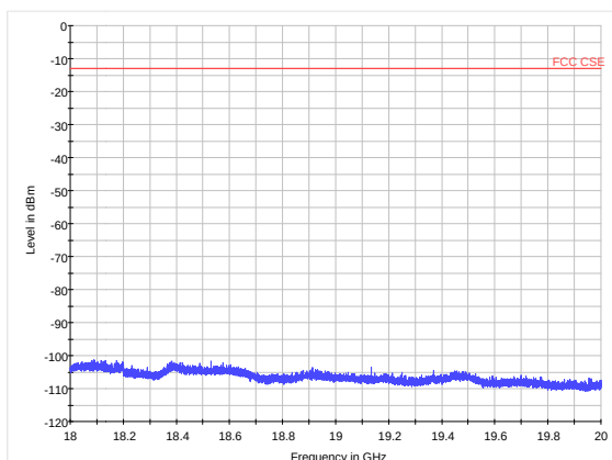
LTE Band 4 20MHz CH-Middle 18GHz~20GHz
