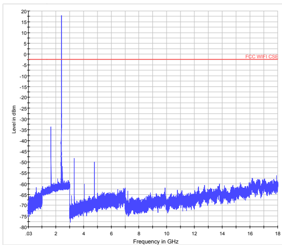
EDR-CH39 30MHz to 18GHz
