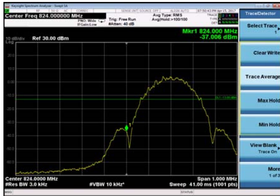
WCDMA Band V CH-Low
