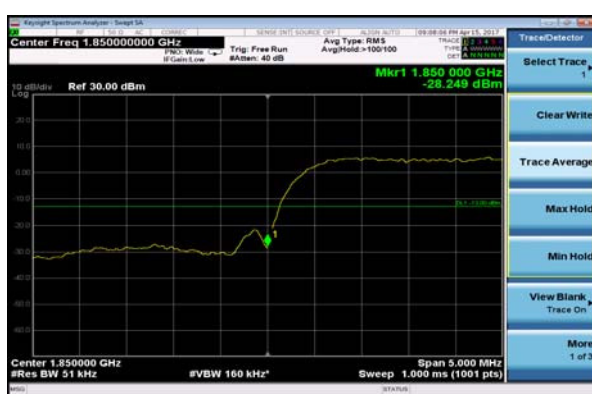
WCDMA Band II RMC CH-Low
