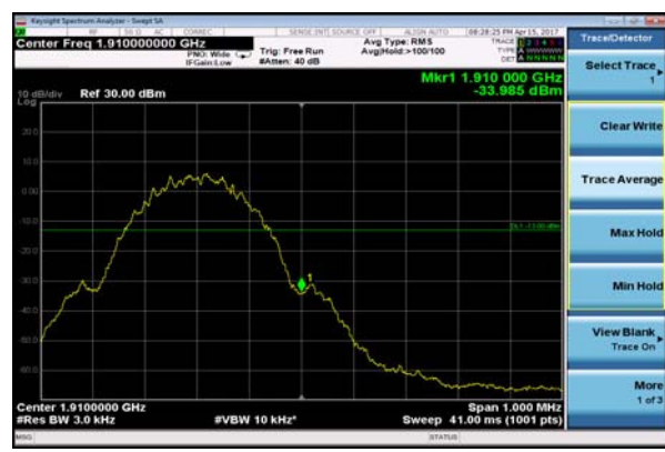
GSM 1900 EGPRS CH-High
