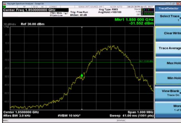
GSM1900 GPRS CH-Low
