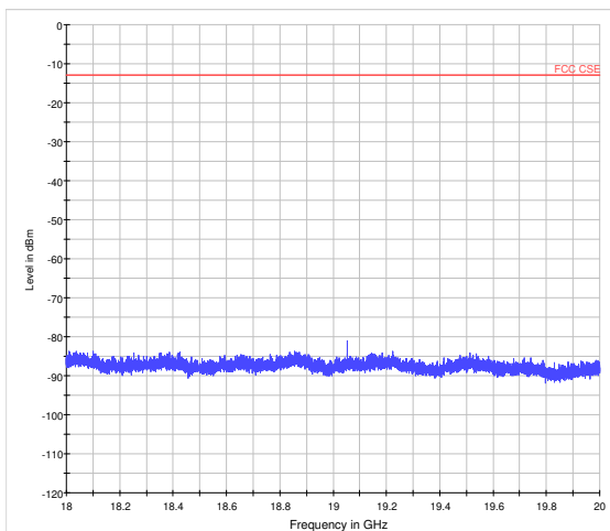
LTE Band 2 5MHz CH-High 18GHz~20GHz
