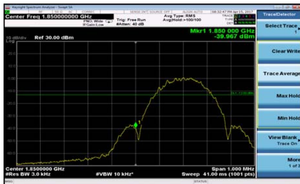
WCDMA Band II RMC CH-Low
