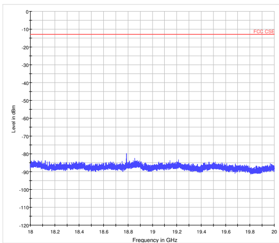
LTE Band 2 3MHz CH-Middle 18GHz~20GHz
