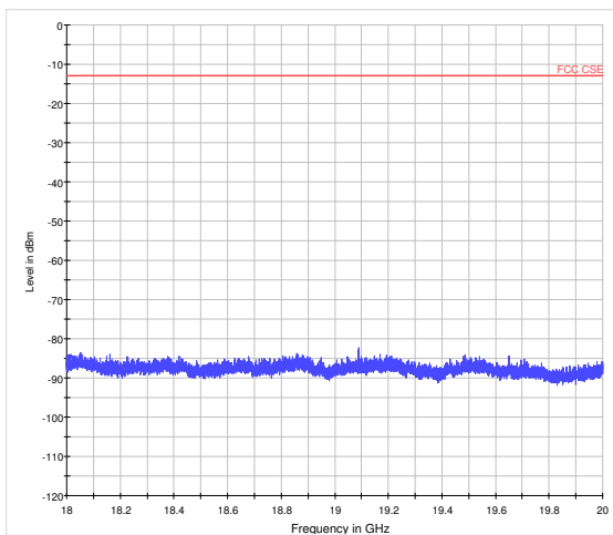
LTE Band 2 1.4MHz CH-High 18GHz~20GHz
