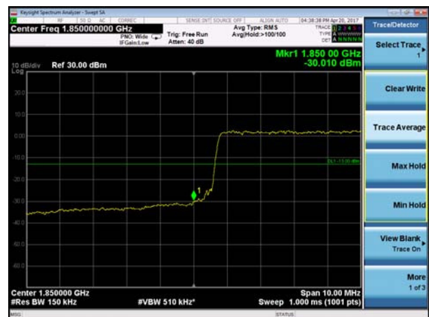
LTE Band 2 15MHz 16QAM 100%RB CH-Low
