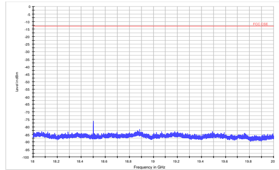
GSM 1900 CH-Low 18GHz~20GHz
