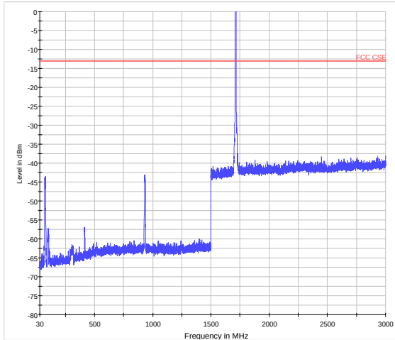
WCDMA Band IV CH-Middle 30MHz~3GHz
