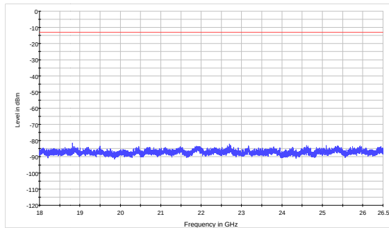
LTE Band 4 15MHz CH-Low 18GHz~26.5GHz
