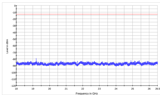
LTE Band 4 10MHz CH-High 18GHz~26.5GHz
