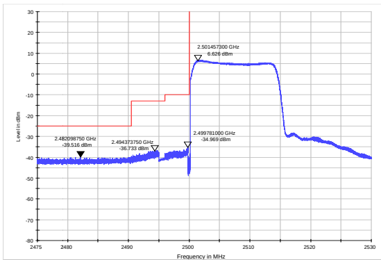
LTE Band 7 16QAM 20MHz CH-Low, RB 1
