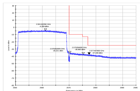
LTE Band 7 16QAM 20MHz CH-High, RB 100
