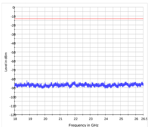
LTE Band 4 1.4MHz CH-Low 18GHz~26.5GHz
