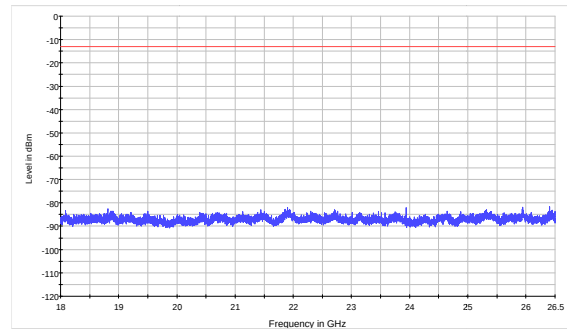
LTE Band 4 3MHz CH-Low 18GHz~26.5GHz
