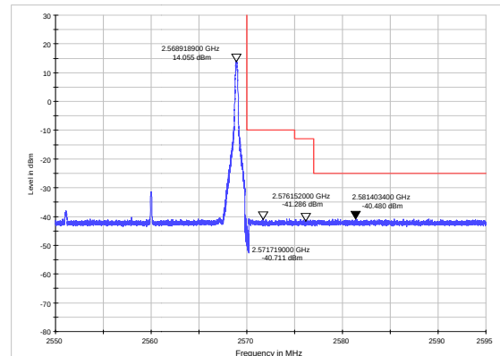
LTE Band 7 16QAM 20MHz CH-High, RB 100
