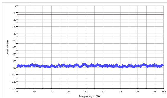
LTE Band 4 10MHz CH-Middle 18GHz~26.5GHz
