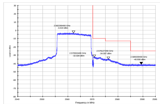
LTE Band 7 16QAM 20MHz CH-High, RB 1
