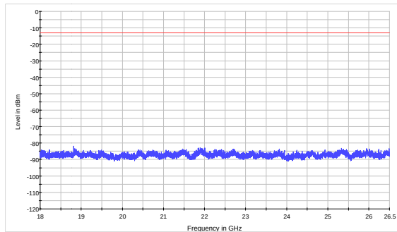
LTE Band 4 5MHz CH-Low 18GHz~26.5GHz
