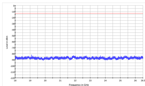
LTE Band 4 20MHz CH-High 18GHz~26.5GHz
