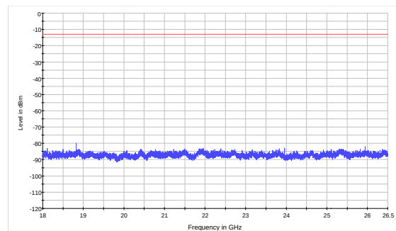
LTE Band 4 20MHz CH-Low 18GHz~26.5GHz
