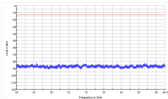
LTE Band 4 15MHz CH-High 18GHz~26.5GHz
