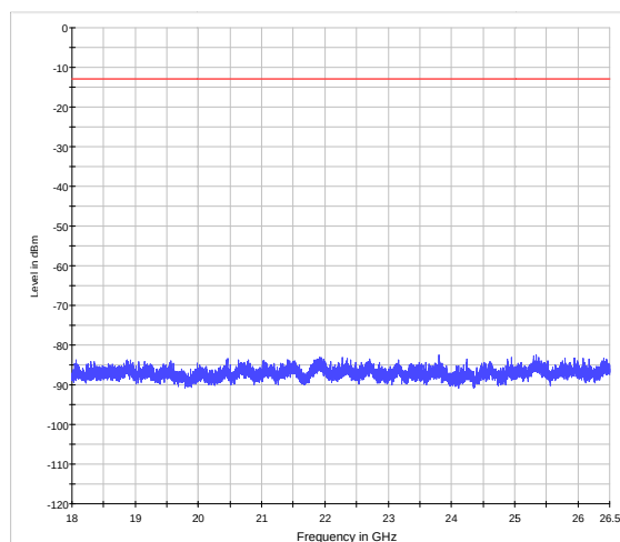
LTE Band 4 1.4MHz CH-Middle 18GHz~26.5GHz
