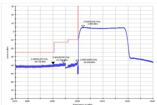
LTE Band 7 16QAM 20MHz CH-Low, RB 100
