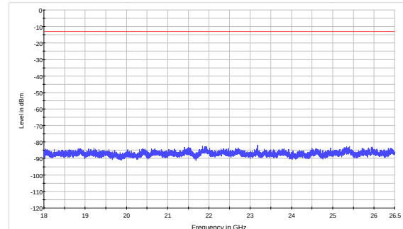
LTE Band 4 3MHz CH-High 18GHz~26.5GHz
