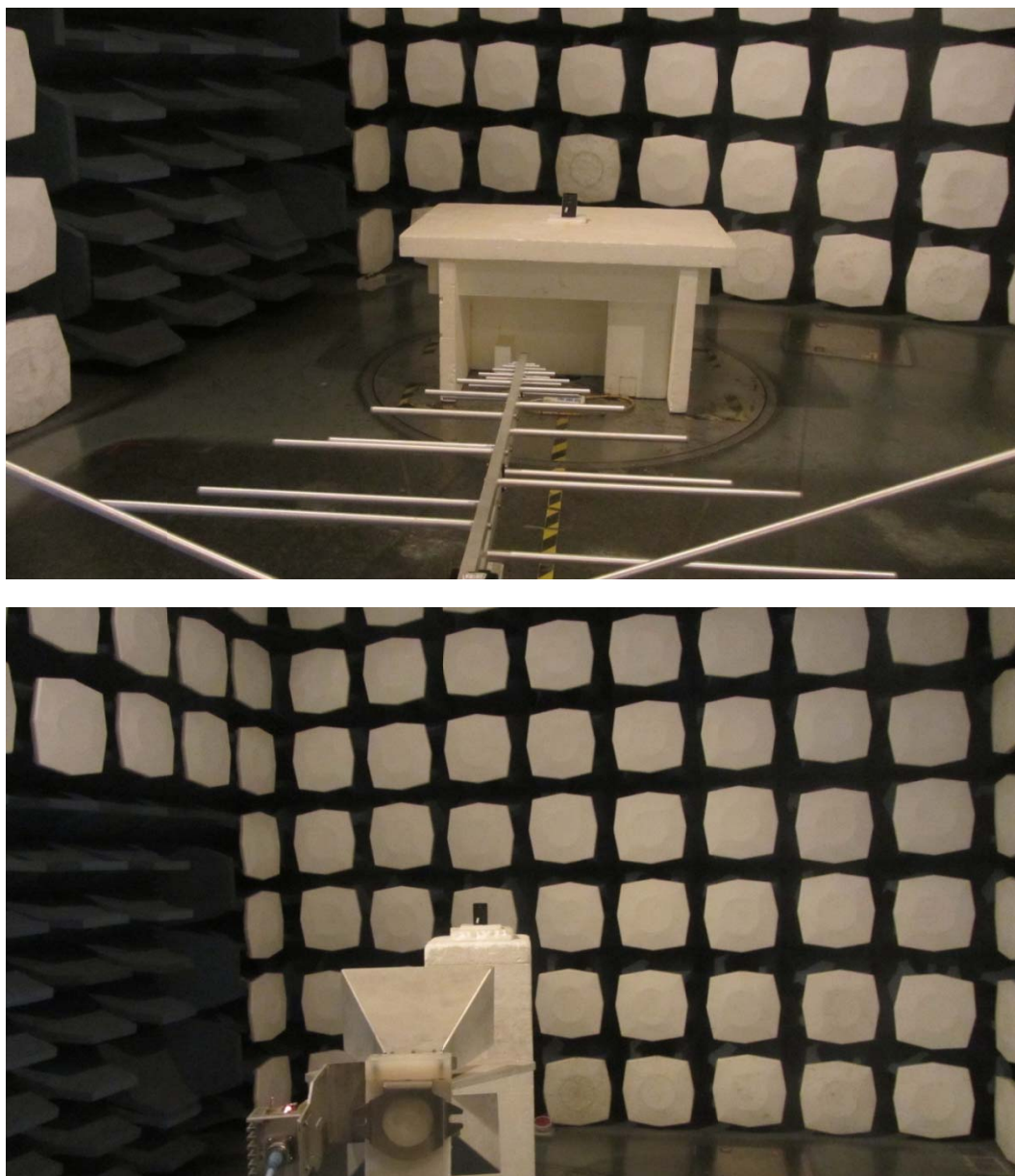
Picture 2: Radiated Spurious Emissions Test setup
