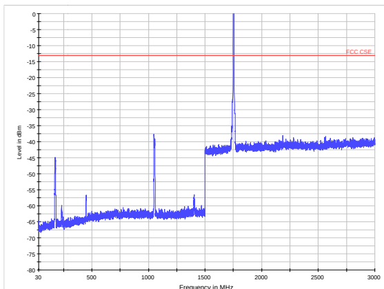
WCDMA Band IV CH-High 30MHz~3GHz
