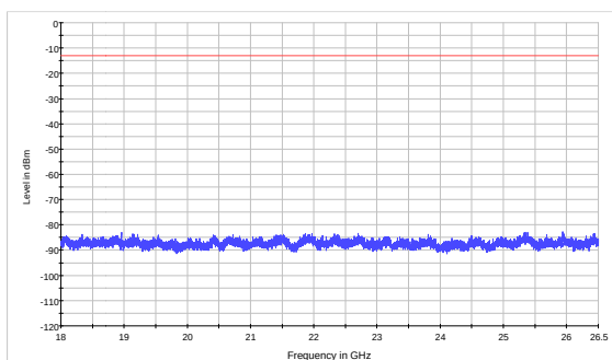
LTE Band 4 20MHz CH-Middle 18GHz~26.5GHz
