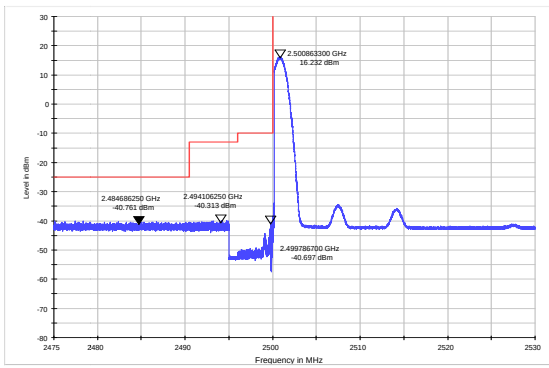
LTE Band 7 16QAM 15MHz CH-Low, RB 75
