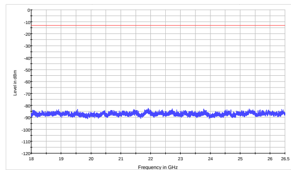
LTE Band 4 10MHz CH-Low 18GHz~26.5GHz
