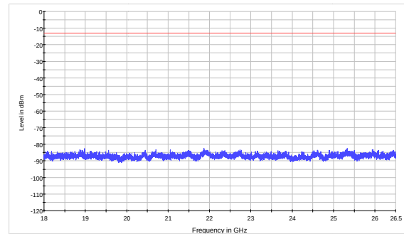
LTE Band 4 15MHz CH-Middle 18GHz~26.5GHz
