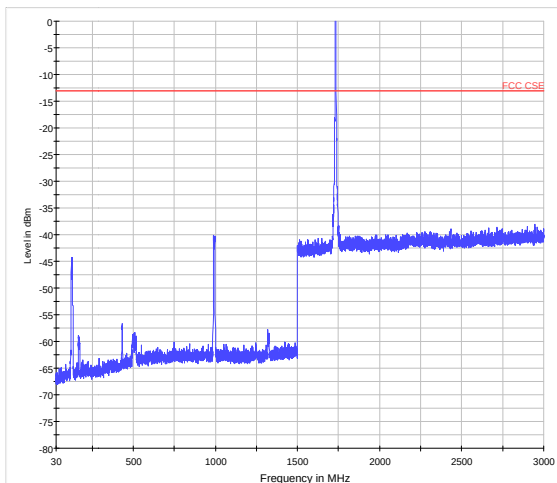
WCDMA Band IV CH-High 30MHz~3GHz
