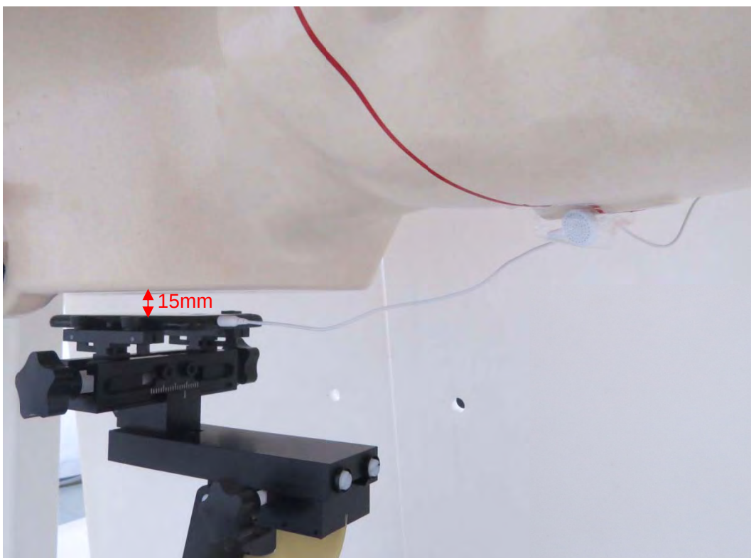
Picture 27: Back Side with Earphone 2, the distance from handset to the bottom of the Phantom is 15mm
