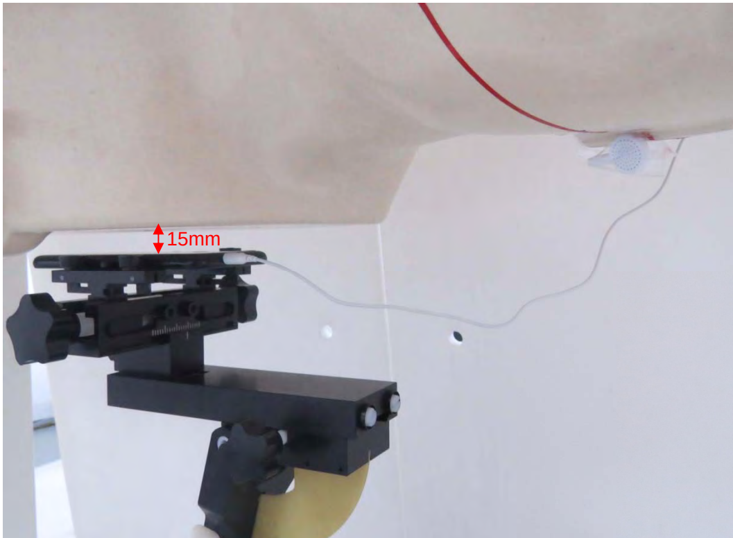
Picture 26: Back Side with Earphone 1, the distance from handset to the bottom of the Phantom is 15mm
