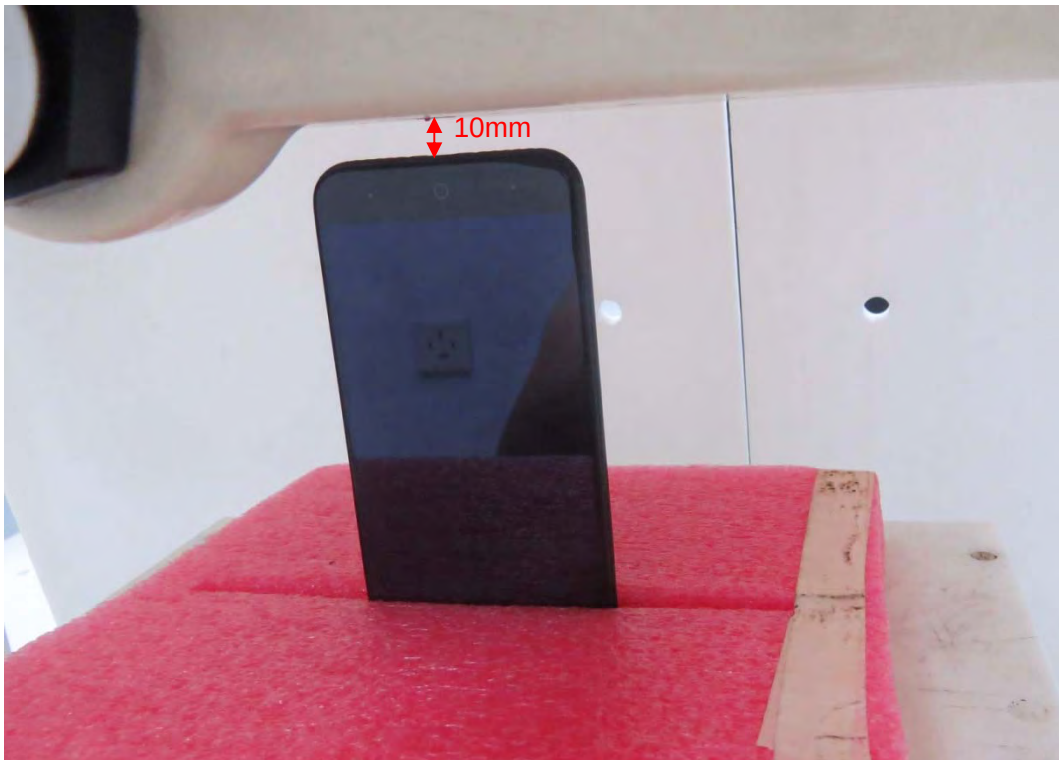
Picture 25: Bottom Side, the distance from handset to the bottom of the Phantom is 10mm
