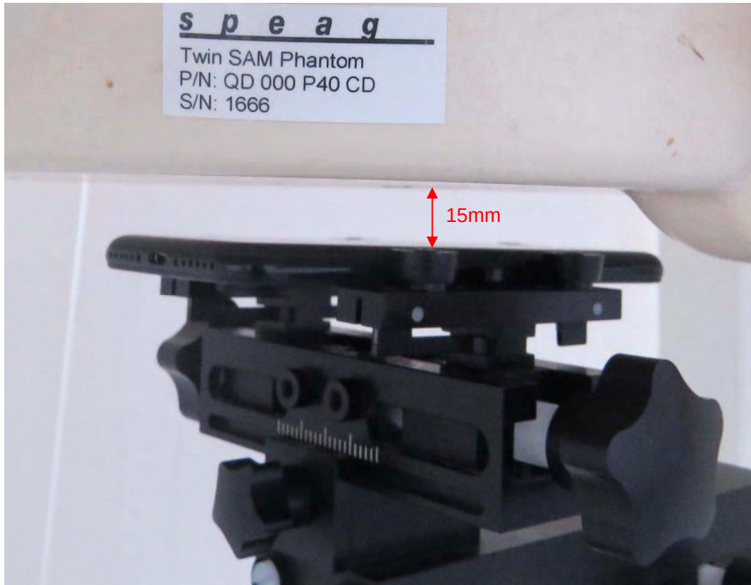
Picture 18: Back Side, the distance from handset to the bottom of the Phantom is 15mm
