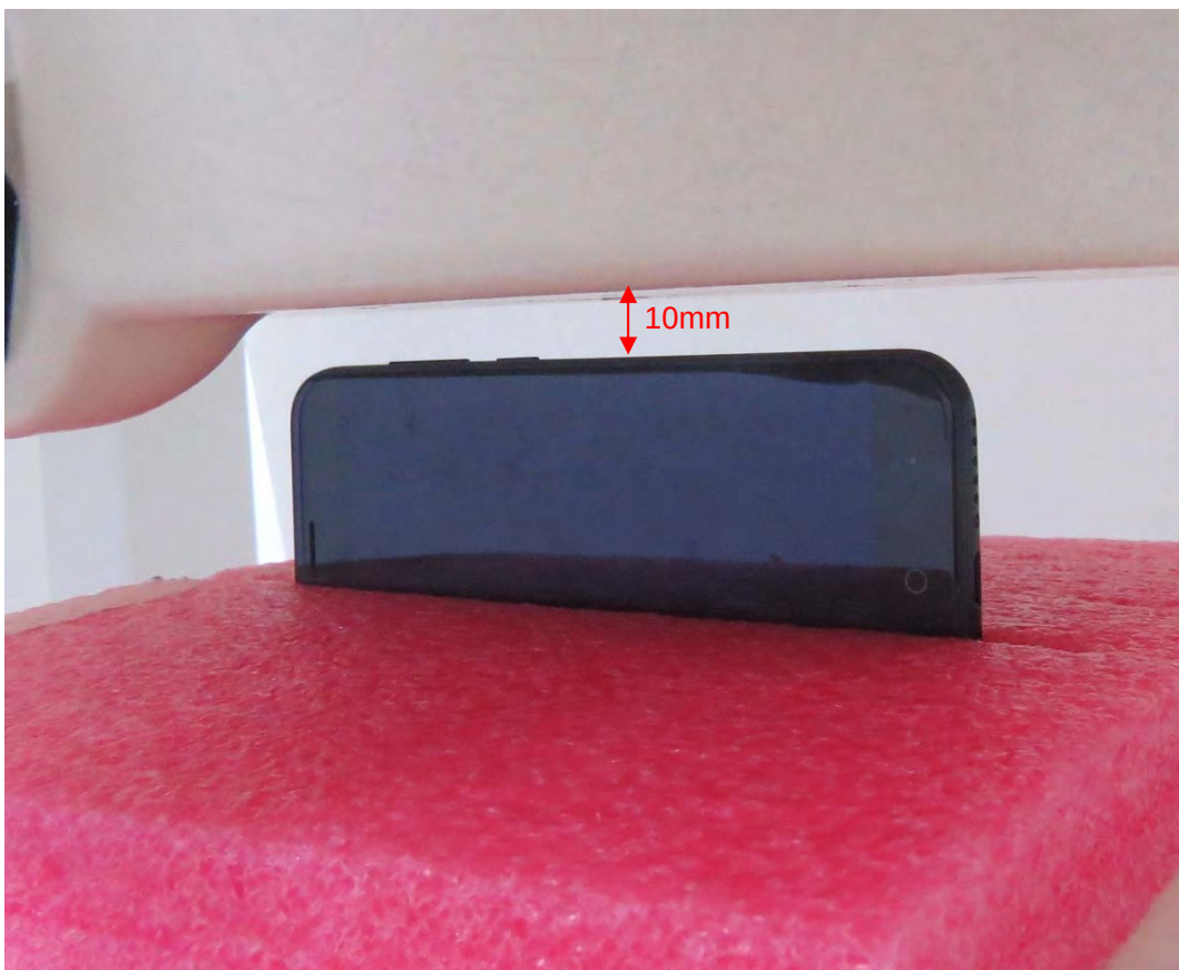
Picture 23: Right Side, the distance from handset to the bottom of the Phantom is 10mm
