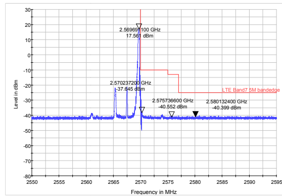
LTE Band 7 16QAM 5MHz CH-High, 100%RB
