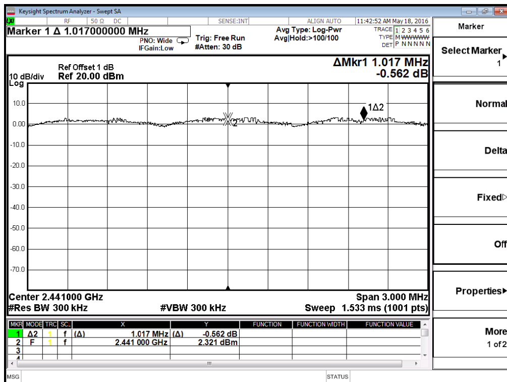
8-DPSK Mode
