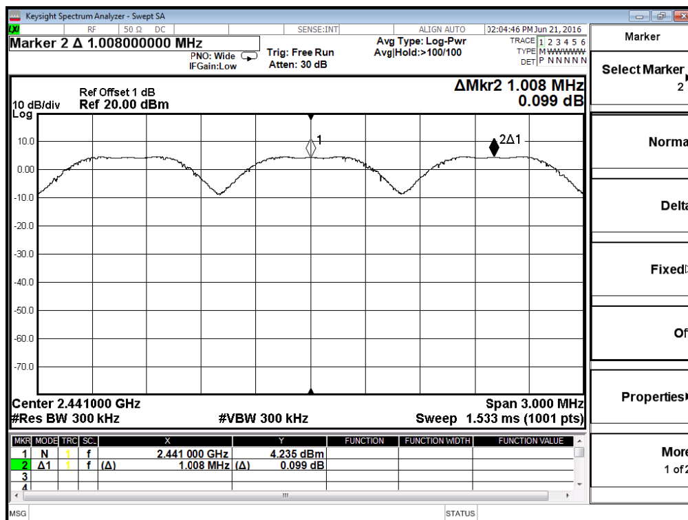
GFSK Mode
