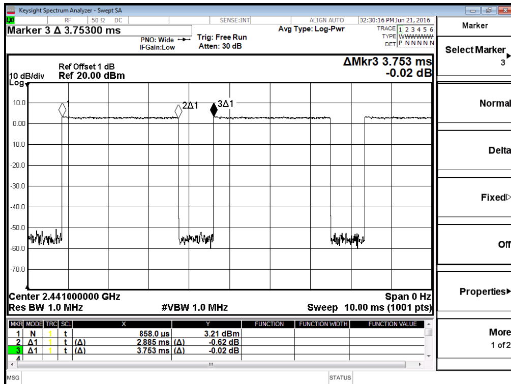
39 Channel @ 2DH5
