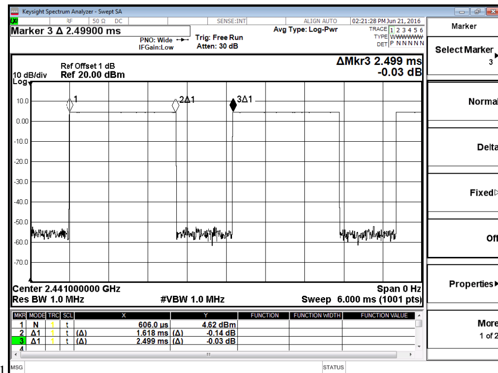
39 Channel @ DH3
