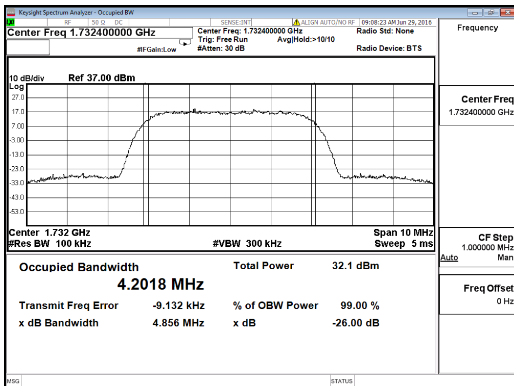
(Plot G2: WCDMA 1700 MHz Channel = 1412 bandwidth)
