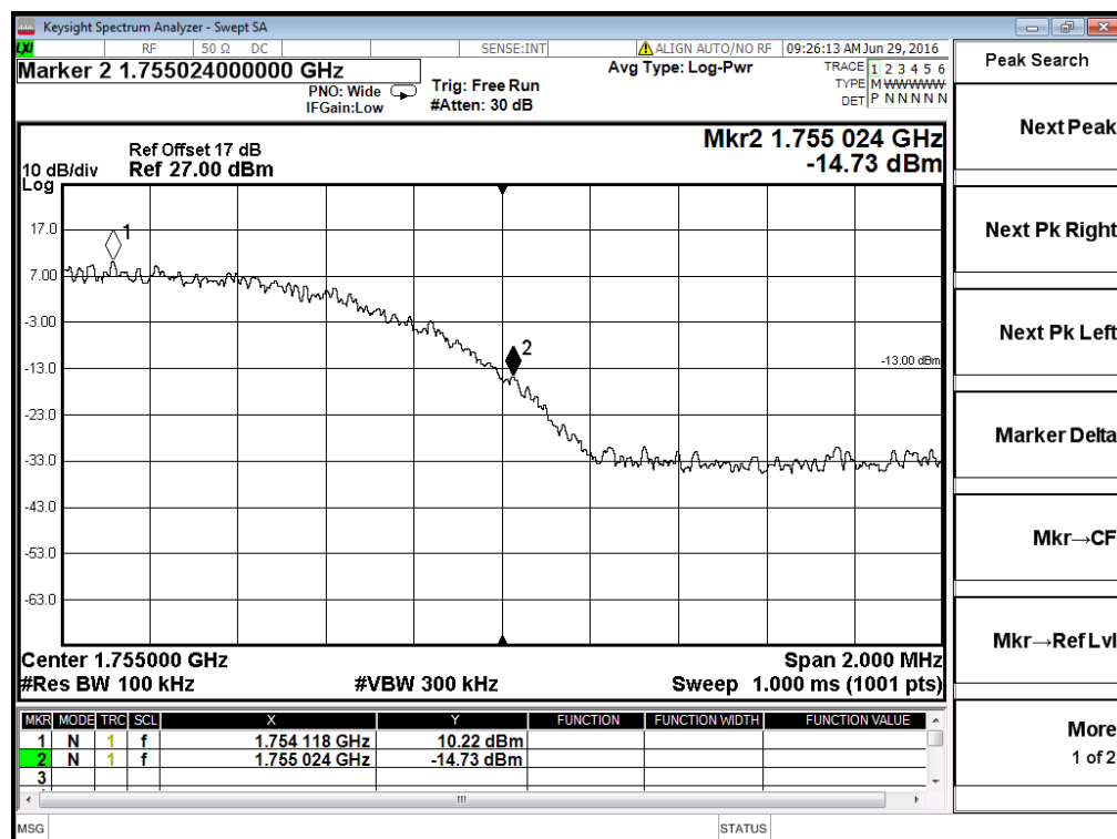
(Plot N: WCDMA 1700 Channel = 1513)
