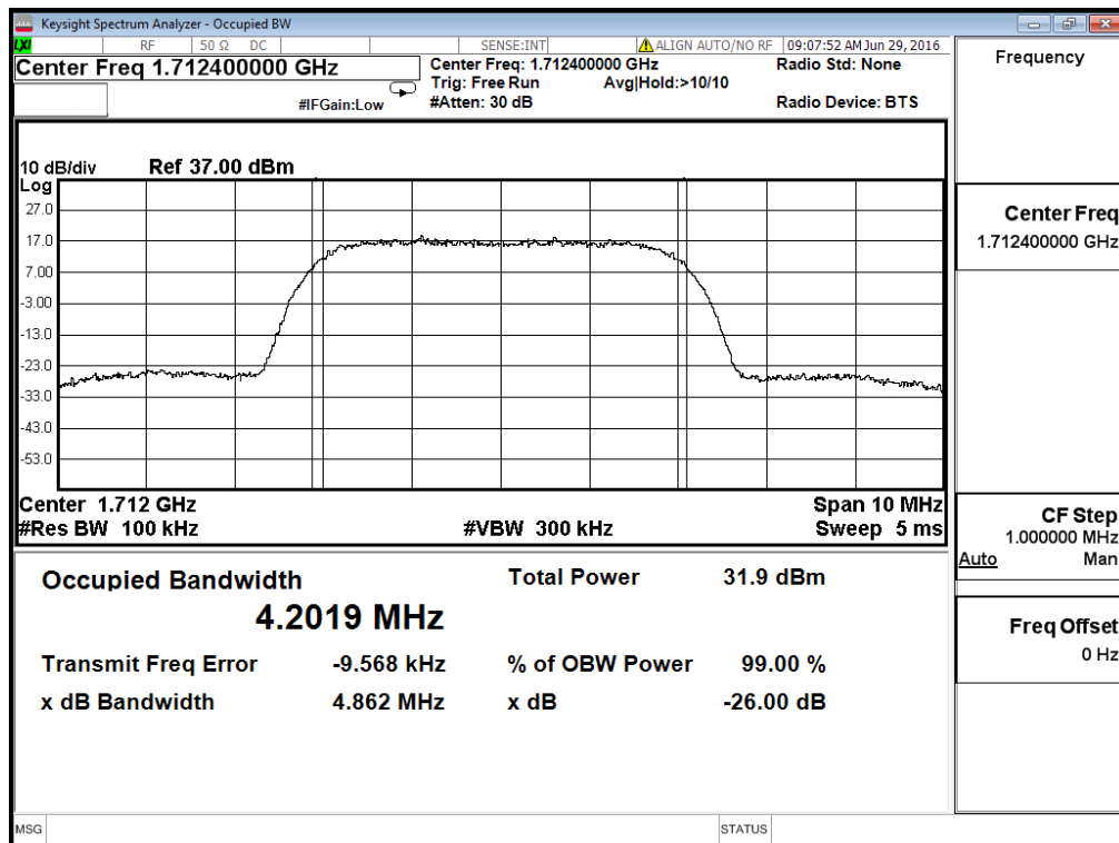
(Plot G1: WCDMA 1700MHz Channel = 1312 bandwidth)
