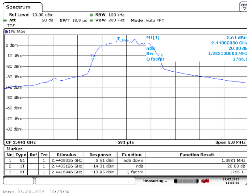
Fig. 57 Occupied 20dB Bandwidth (8DPSK, Ch 39)
