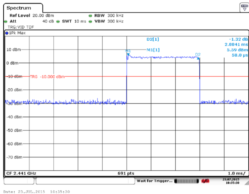
Fig. 61 Time of Occupancy(Dwell Time) ( \pi/4 DQPSK, Ch39)
