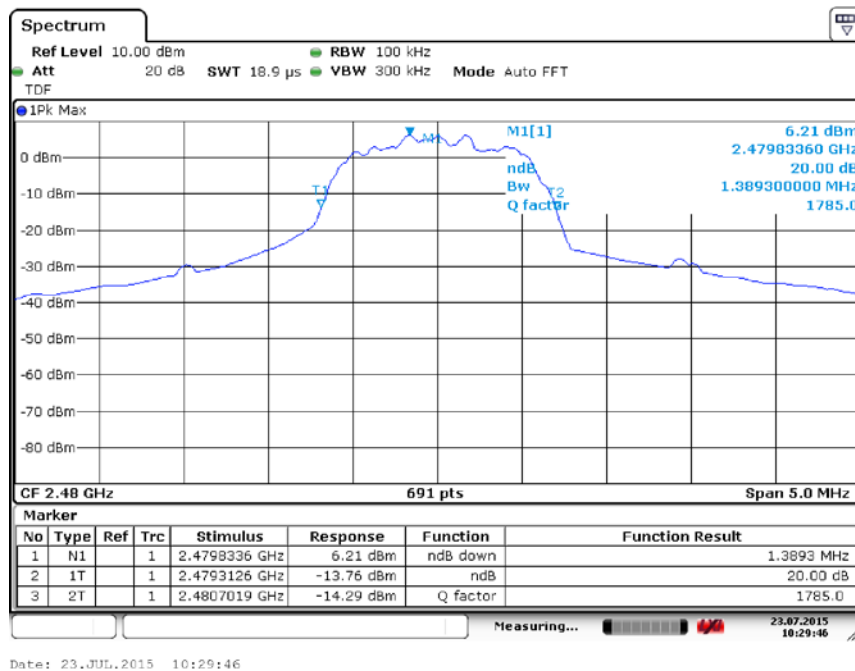
Fig. 58 Occupied 20dB Bandwidth (8DPSK, Ch 78)
