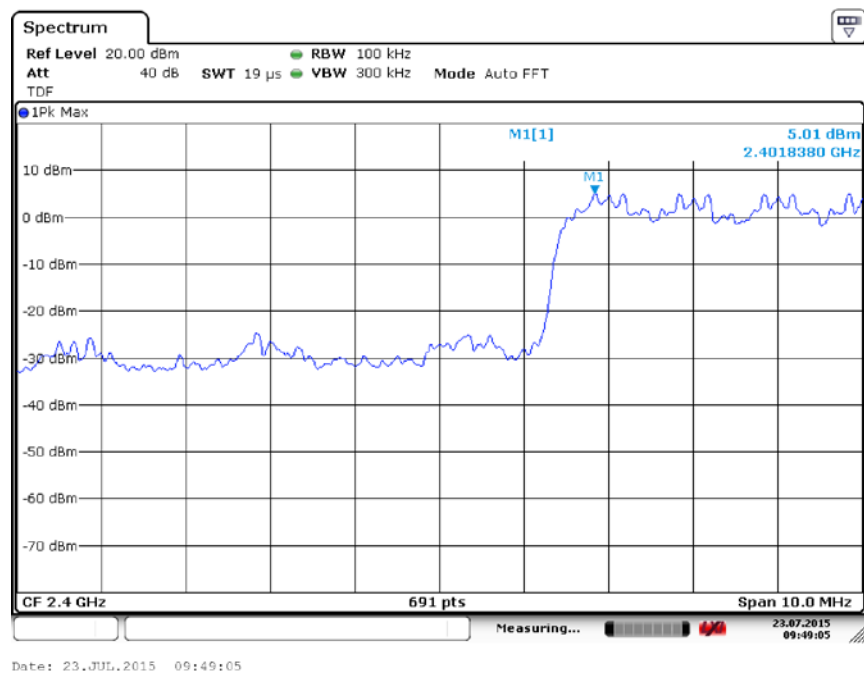
Fig. 14 Band Edges (8DPSK, Ch 0, Hopping ON)
