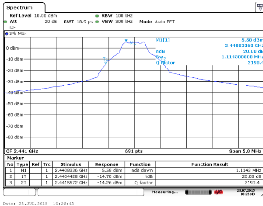
Fig. 51 Occupied 20dB Bandwidth (GFSK, Ch 39)
