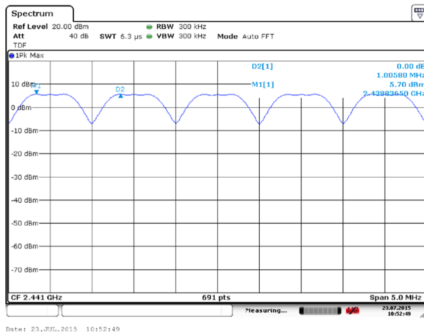
Fig. 71 Carrier Frequency Separation (GFSK, Ch39)
