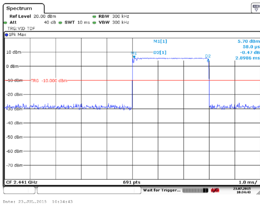
Fig. 59 Time of Occupancy(Dwell Time) (GFSK, Ch39)
