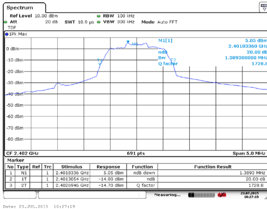
Fig. 53 Occupied 20dB Bandwidth ( \pi/4 DQPSK, Ch 0)
