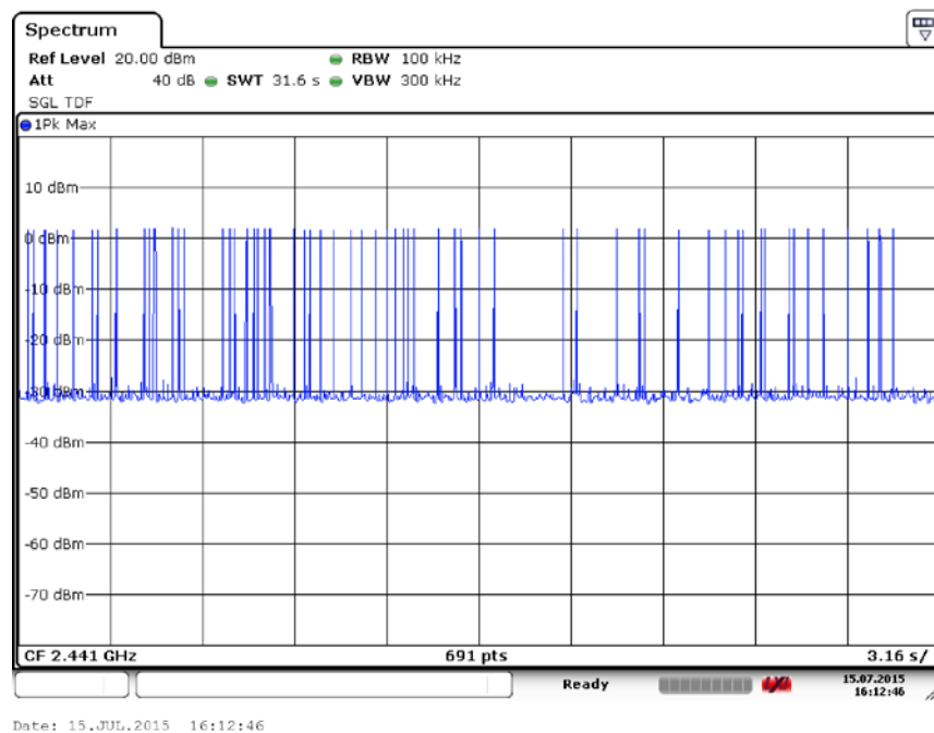
Fig. 64 Number of Transmissions (8DPSK, Ch39)
