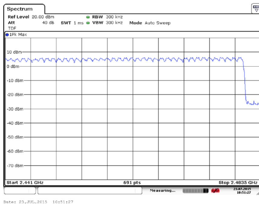
Fig. 70 Hopping channel ch39~78 (8DPSK, Ch39)
