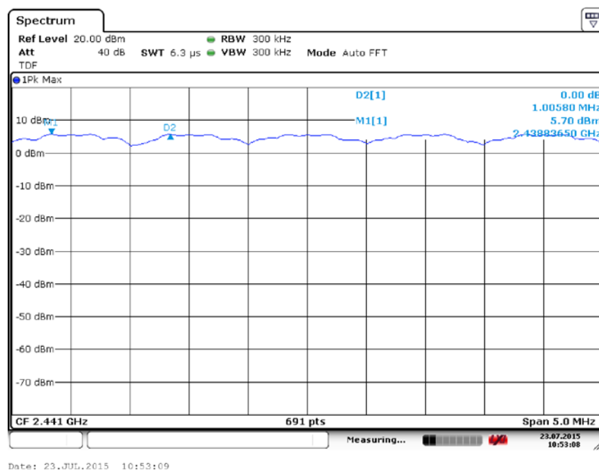
Fig. 72 Carrier Frequency Separation ( \pi/4 DQPSK, Ch39)
