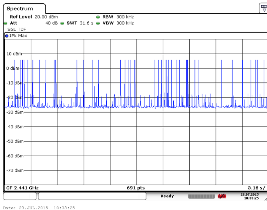
Fig. 60 Number of Transmissions (GFSK, Ch39)
