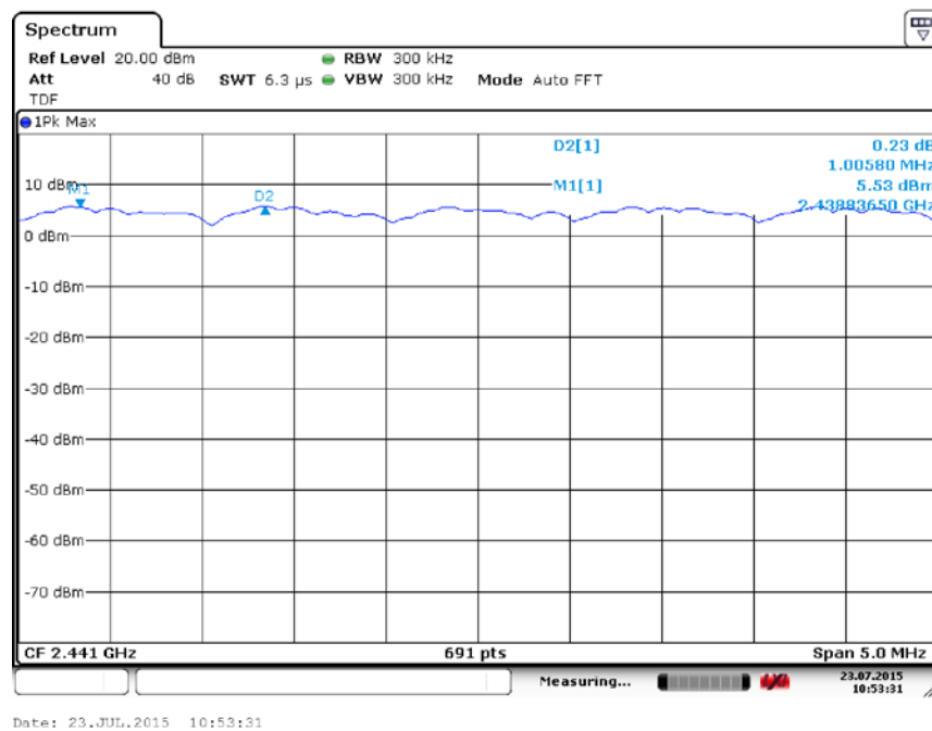
Fig. 73 Carrier Frequency Separation (8DPSK, Ch39)
