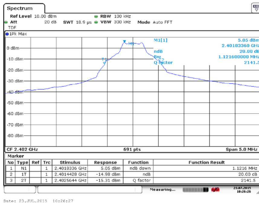
Fig. 50 Occupied 20dB Bandwidth (GFSK, Ch 0)
