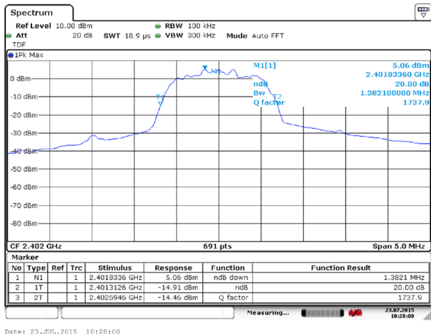
Fig. 56 Occupied 20dB Bandwidth (8DPSK, Ch 0)
