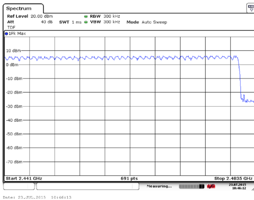
Fig. 67 Hopping channel ch0~39 ( \pi/4 DQPSK, Ch39)
