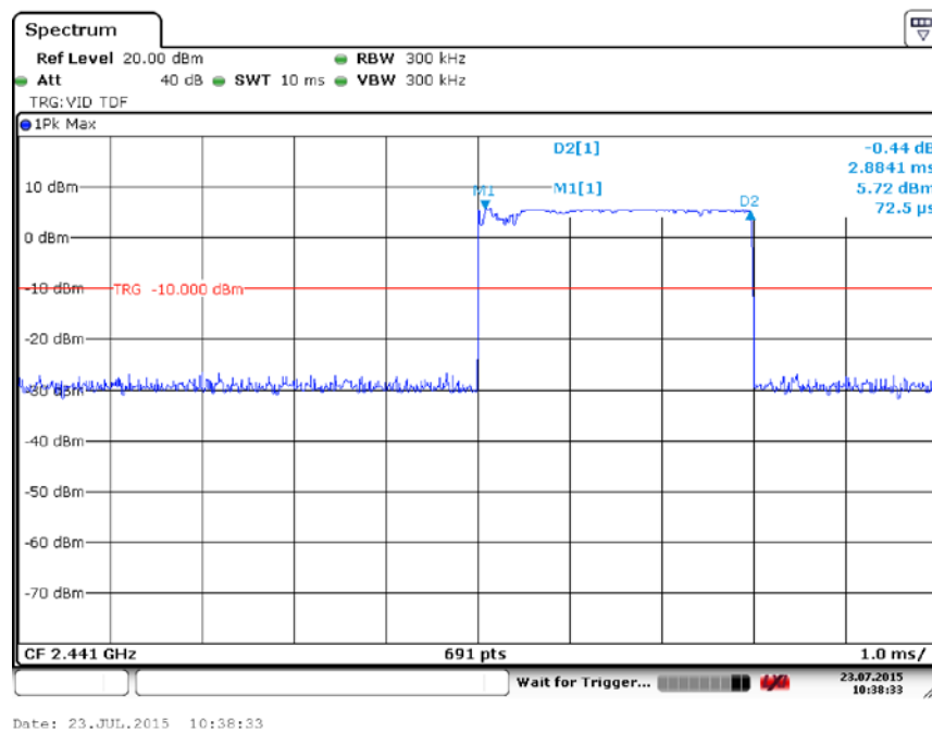
Fig. 63 Time of Occupancy(Dwell Time) (8DPSK, Ch39)
