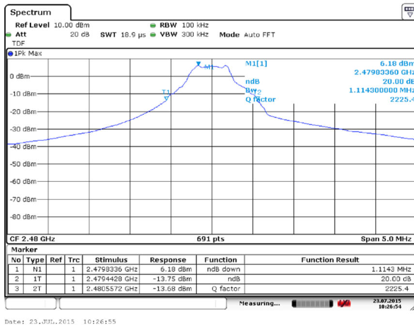
Fig. 52 Occupied 20dB Bandwidth (GFSK, Ch 78)
