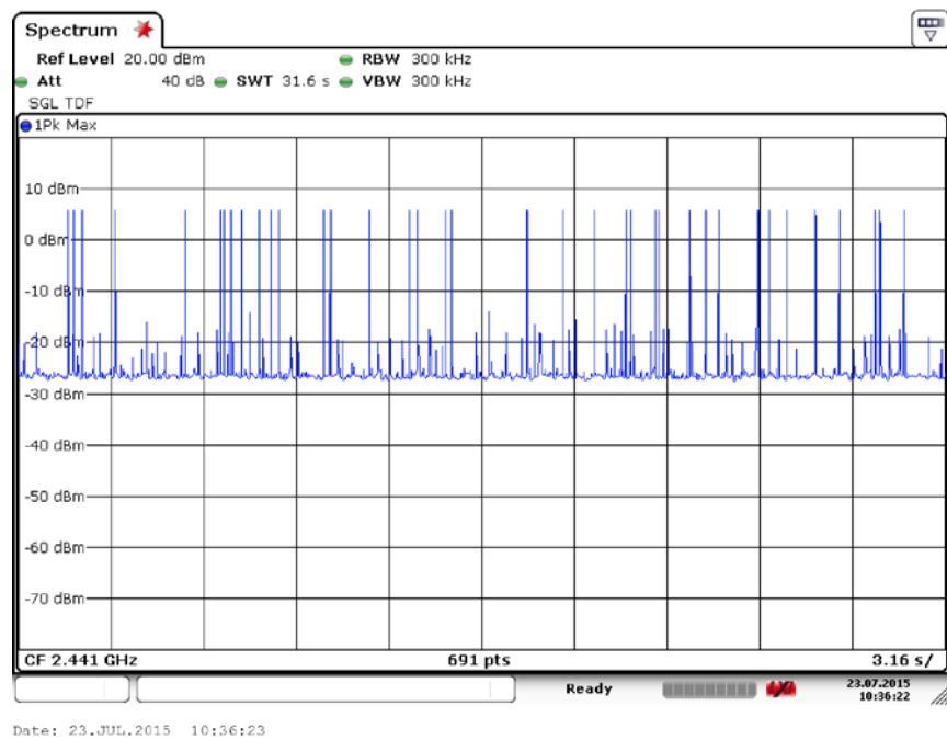
Fig. 62 Number of Transmissions ( \pi/4 DQPSK, Ch39)
