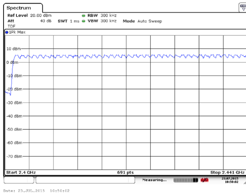
Fig. 69 Hopping channel ch0~39 (8DPSK, Ch39)
