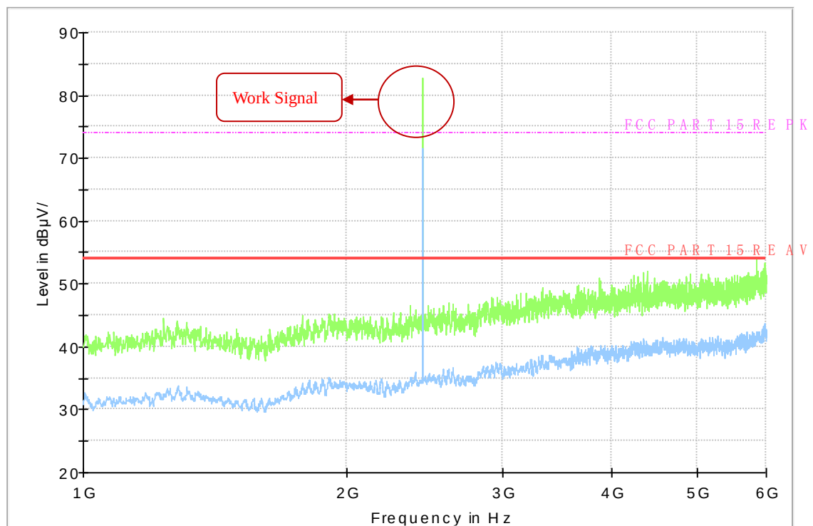
Fig.2 Radiated Emission of channel 0 in 1GHz-6GHz
