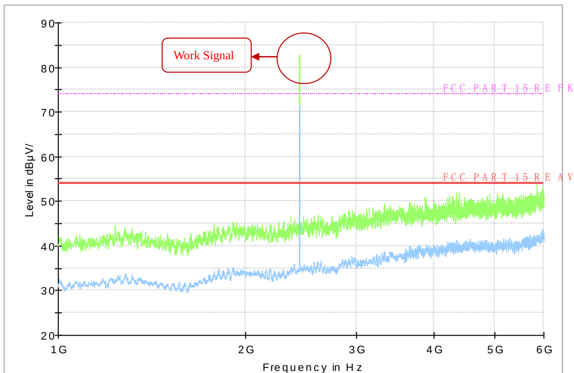
Fig.6 Radiated Emission of channel 78 in 1GHz-6GHz
