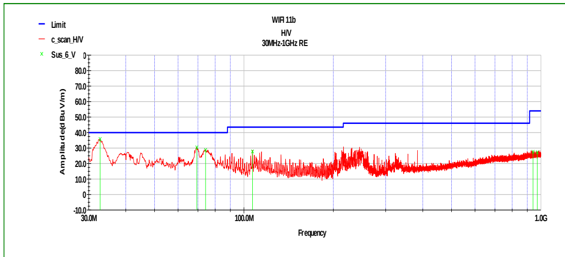
Fig.1 Radiated Emission of channel 1 in 30MHz-1GHz
