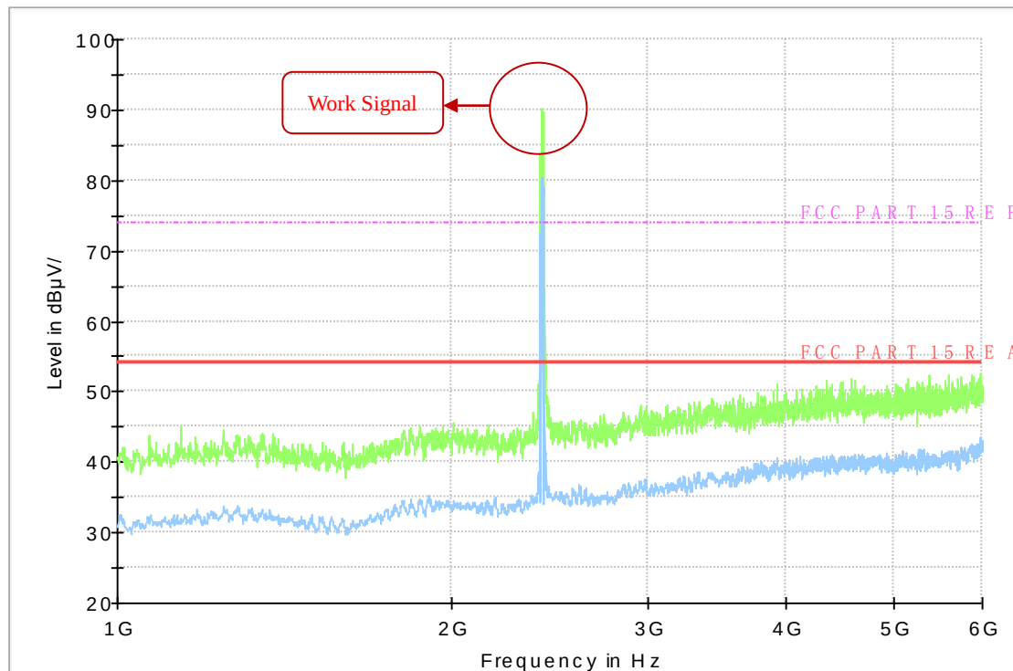
Fig.12 Radiated Emission of channel 1 in 1GHz-6GHz
