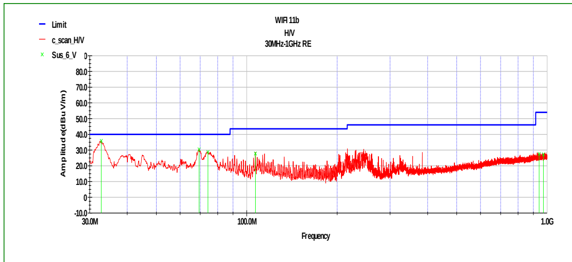
Fig.3 Radiated Emission of channel 6 in 30MHz-1GHz
