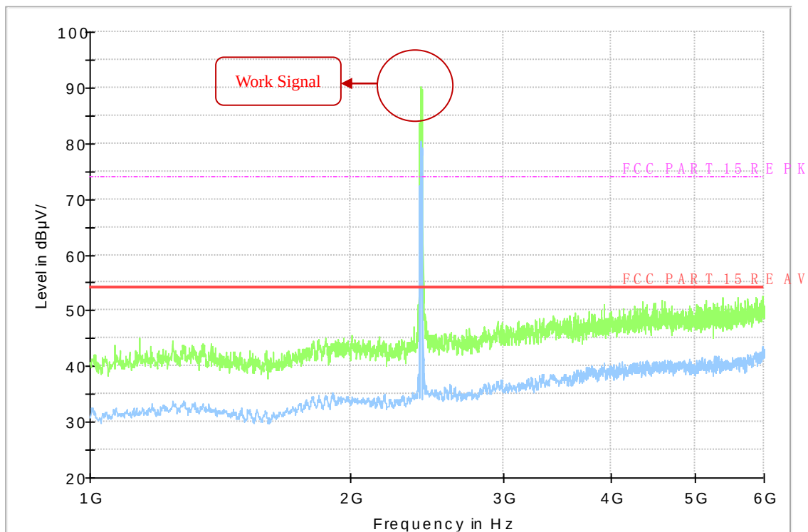
Fig.6 Radiated Emission of channel 11 in 1GHz-6GHz
