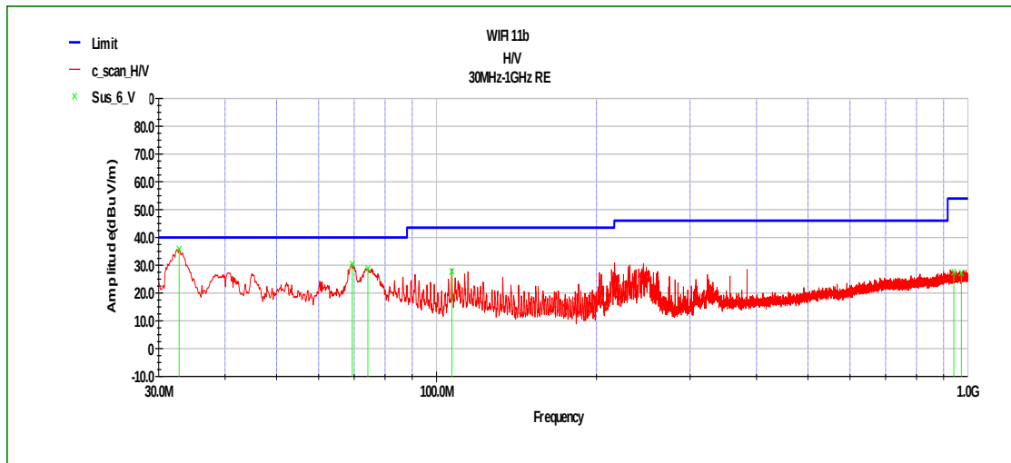
Fig.5 Radiated Emission of channel 11 in 30MHz-1GHz
