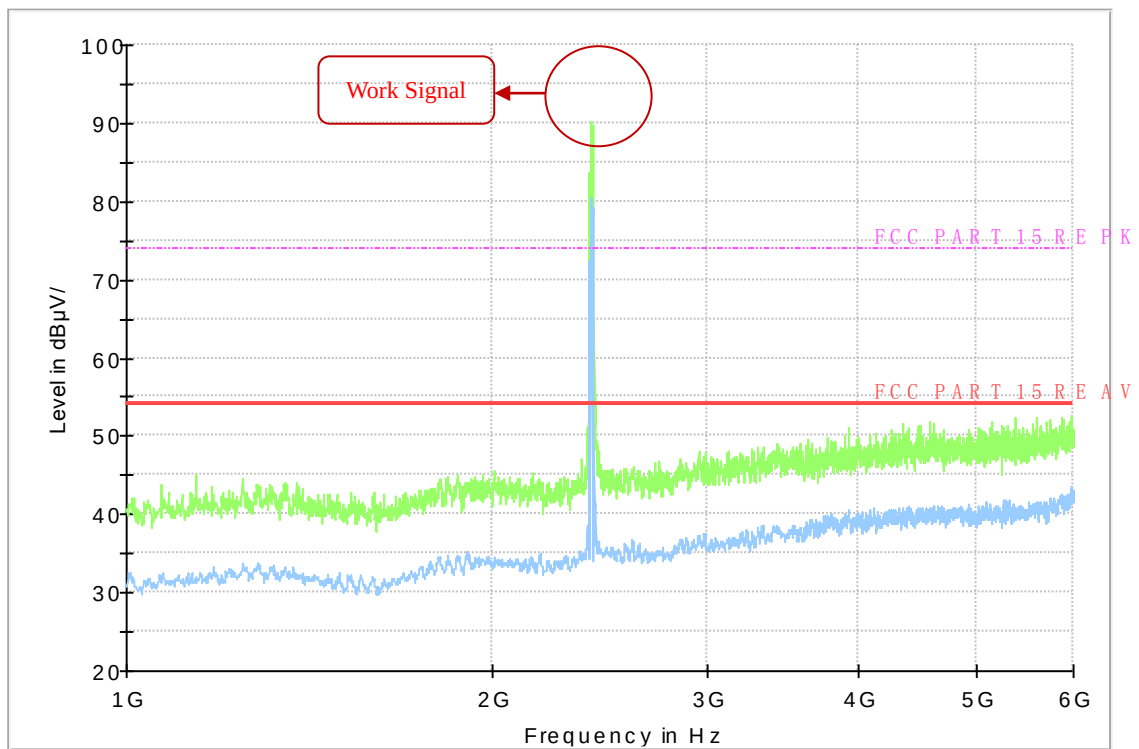
Fig.4 Radiated Emission of channel 6 in 1GHz-6GHz
